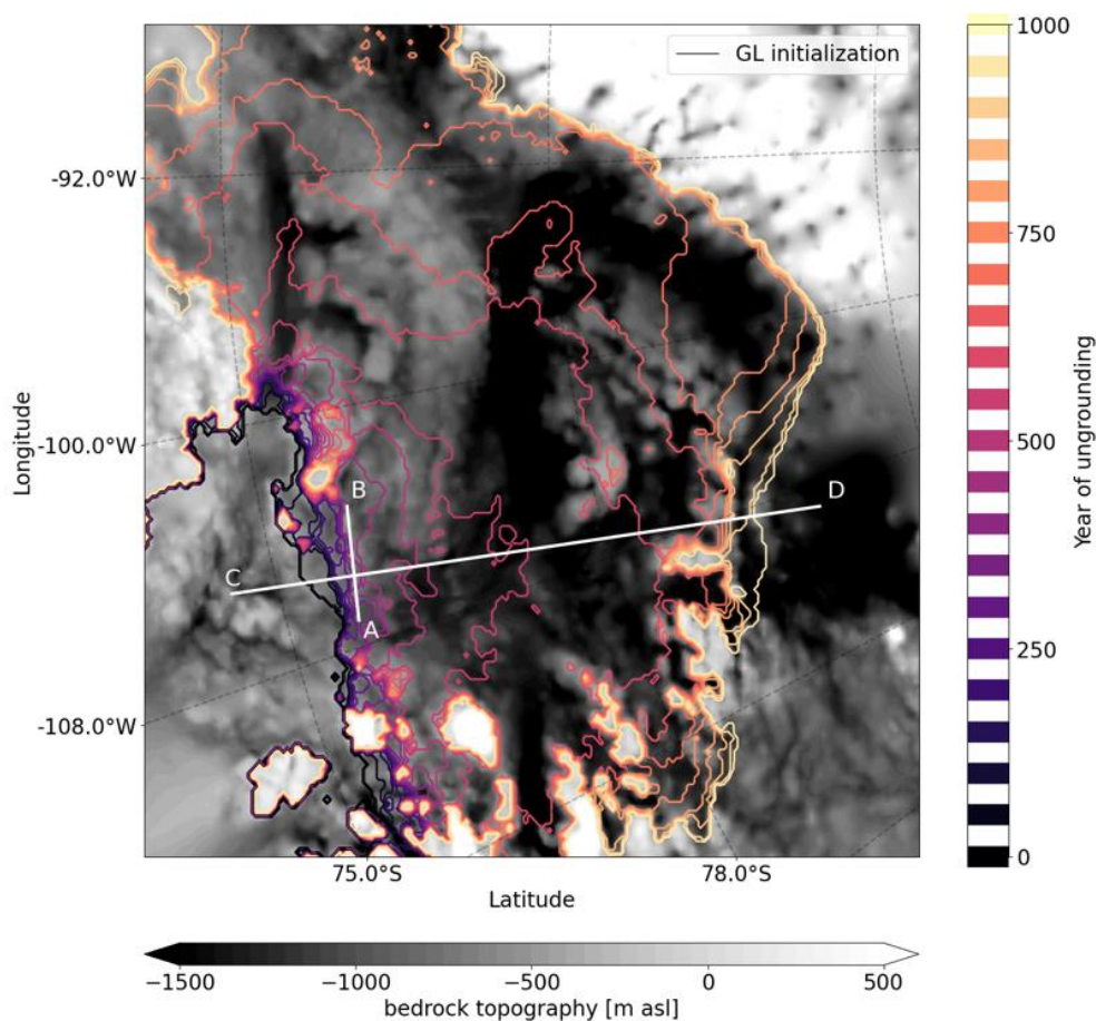
Figure 4. ASE bedrock topography and grounding line migration of the future simulation. The bedrock elevation (m) is shown with grey shading. Magma contours show the grounding line position at different times during the default continuation experiment. Contour lines clumped together highlight areas where the grounding line stabilizes for long periods. The short white line ( AB ) shows the last prominent ridge before the accelerated collapse starts, and the long white semi-horizontal white line ( CD ) shows the location of the cross section plotted in Fig. 2 in the main text. 390
