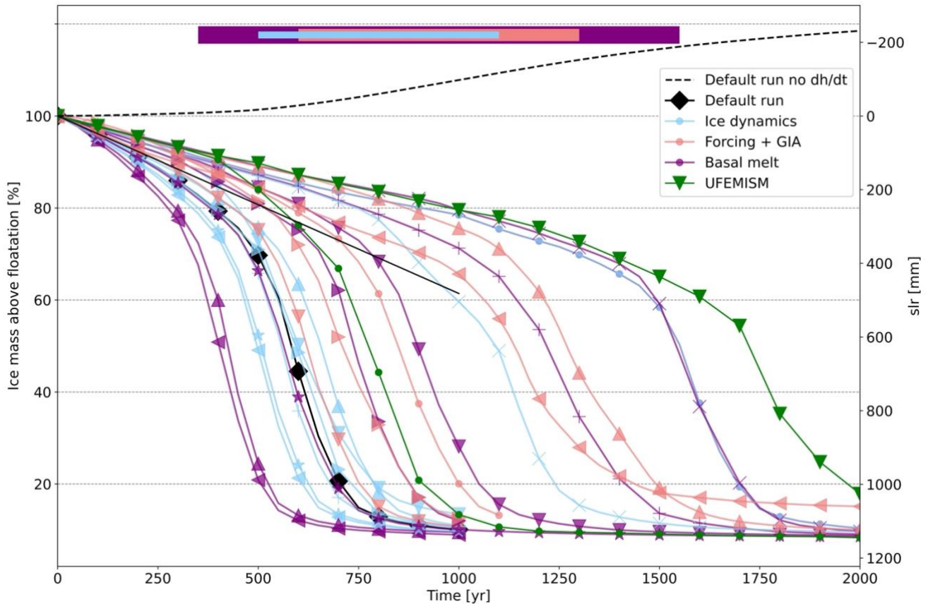
Figure 8. Sensitivity analysis. Ice mass above floatation (left y-axis) and resulting sea level rise (right axis) in the combined Thwaites and Pine Island Glacier basins for different experiments (22 in total). The mass change is calculated as the percentage difference relative to the initial value in the TG and PIG basins. The default run shown in Fig. 3 is plotted with black diamonds. The same run without applying the present-day mass change rates, i.e. the model drift experiment, is shown as a dashed line. The UFEMISM runs are shown in green, and the extrapolated observations as in Fig. 2b are shown in marker-free black. Most runs start with the observed mass change rates but deviate early in the run due to dynamic feedbacks. Some runs, e.g. “SMB increases by 20% instantly” start with different mass change rates. This explains the spreading trajectories in the first 100 years. The colored bars at the top indicate the range of times that the simulations reach 50% of their present-day ice volume, to highlight the uncertainty related to different categories. See Table 3 for a description of each run.
