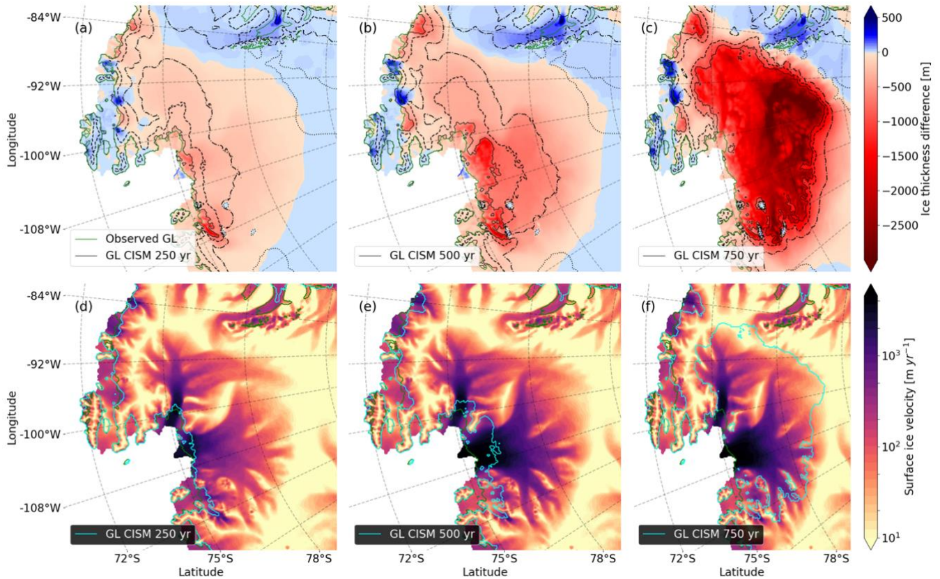
410 Figure 5. Development of the collapse at three times. (Top) Ice thickness difference with respect to the end of the initialization at t=250 yr (a), t=500 yr (b) and t=750 yr (c) after the start of the default continuation experiment. The present- day GL from observations is shown in green, and the modeled GL is shown in black. The ice surface elevation lines are contours of 500 (dashed), 1000 (dash-dotted) and 2000 (dotted) meters. (Bottom) Ice surface velocities at t=250 (d), t=500 (e) and t=750 (f) years, with the modeled GL shown in cyan, and the observed GL in green.
