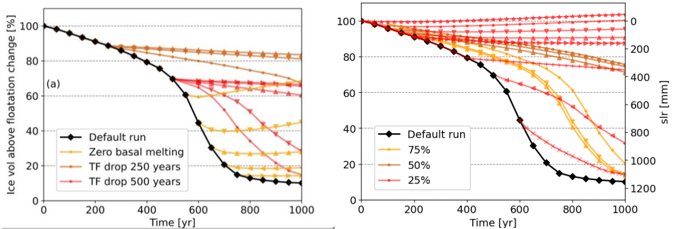
430 Figure 6. The impact of decreasing basal melt rates on the ice retreat. (Left) Evolution of ice volume (shown as a percentage relative to the initial volume (see Fig. 1) for PIG and TG combined and as sea-level equivalent on the right y-axis) over 1000 years in experiments with a sudden decrease in basal melt rates. Brown lines show where the thermal forcing (TF) is instantly decreased after 250 years by 1 K, 1.5 K and 2 K, and the red lines show simulations where the thermal forcing is decreased after 500 years by 1.5 K, 2 K, 2.5 K and 3 K. Yellow lines indicate runs where the basal melting is instantly switched off after 500, 600, 700 and 800 years. (Right) Percentage of the basal melt rates applied: 25% (red), 50% (brown) and 75% (yellow). The 50% and 75% basal melt rate experiments are started at 50, 100 and 150 435 years, and the 25% basal melt rate experiments are started at 0, 50, 100, 150, 200, 400, 500 and 600 years after the start of a transient continuation run.
