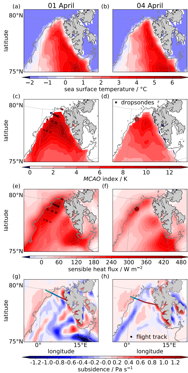
Figure 3. Overview of environmental conditions on 01 April (left) and 04 April (right). Maps of sea surface temperature (a, b), MCAO index (c, d), sensible heat fluxes (e, f), and subsidence at 925 (g) and 975 hPa (h) from ERA5 reanalysis data. Positive subsidence values indicate downward motion. MCAO indices (c, d) and sensible heat fluxes (e, f) from dropsonde observations are shown as circles. Flight tracks in (g) and (h) are color-coded according to the measurement categorization (Table 1). The gray lines indicate the 15 % sea ice concentration from ERA5.
