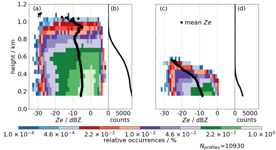
Figure 5. Contoured frequency by altitude diagram (a, c) and absolute counts per altitude (b, d) for all radar reflectivities ( Ze ) obtained by MiRAC in the 'cloud street' regime on 01 April (a, b) and 04 April (c, d). Moreover, each averaged Ze profile (black dots), and the total number of profiles ( N_{\text{profiles}} ) is displayed.
