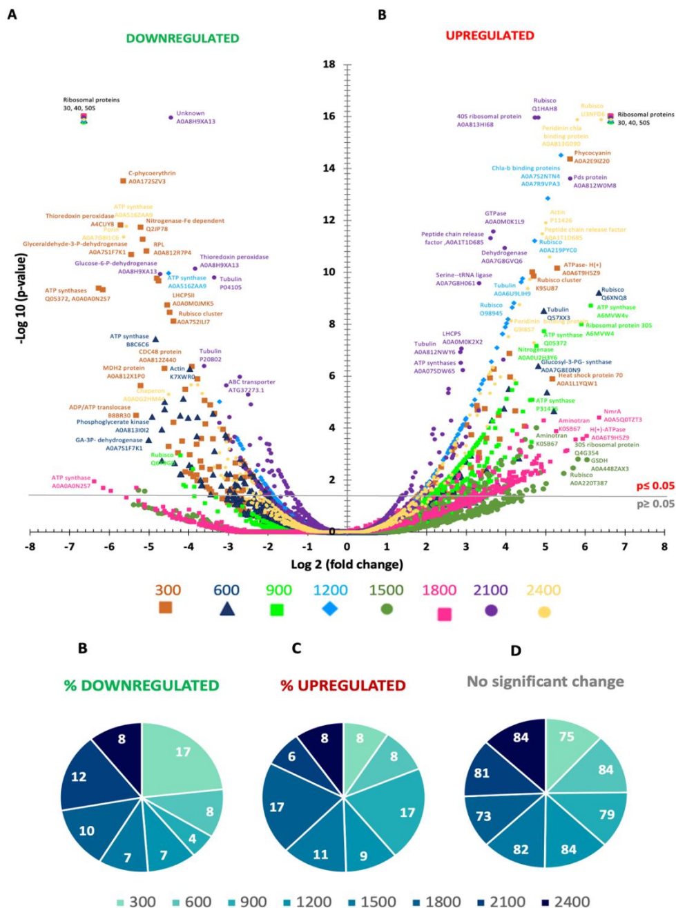
Figure 3. A) Volcano plot showing the metaproteome analysis on t27 of the experiment for all the mesocosms except for the control \Delta TA 0. The statistical significance ( -\log_{10} p-value) of the magnitude of change ( \log_2 -fold-change) is tested with respect to the control. Each dot in the plot is one protein normalised by housekeeping proteins and by the control. Downregulated protein abundances appear in the left part of the plot, whilst upregulated ones are shown at the right half of the plot. B) Pie-sector plots representing the percentages of significant proteins abundances upregulated, downregulated and with no changes. Colour and symbol-codes for alkalinity levels for each mesocosm are shown below each plot.
