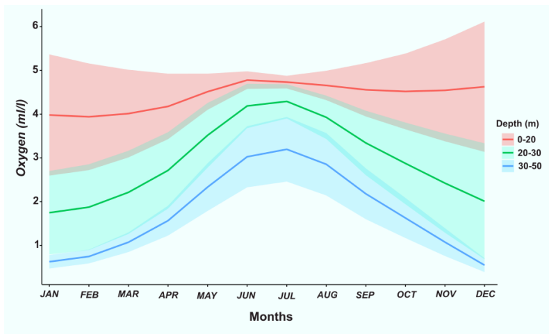
New Fig. 3. The annual cycle (monthly climatology) of oxygen concentration in three strata in the upper 50 m layer at central-southern Chile (36°30' S). Oxygen data are from the time series study at Station 18 off central-southern Chile during the period 2002-2016 (Frederick et al., 2024).
