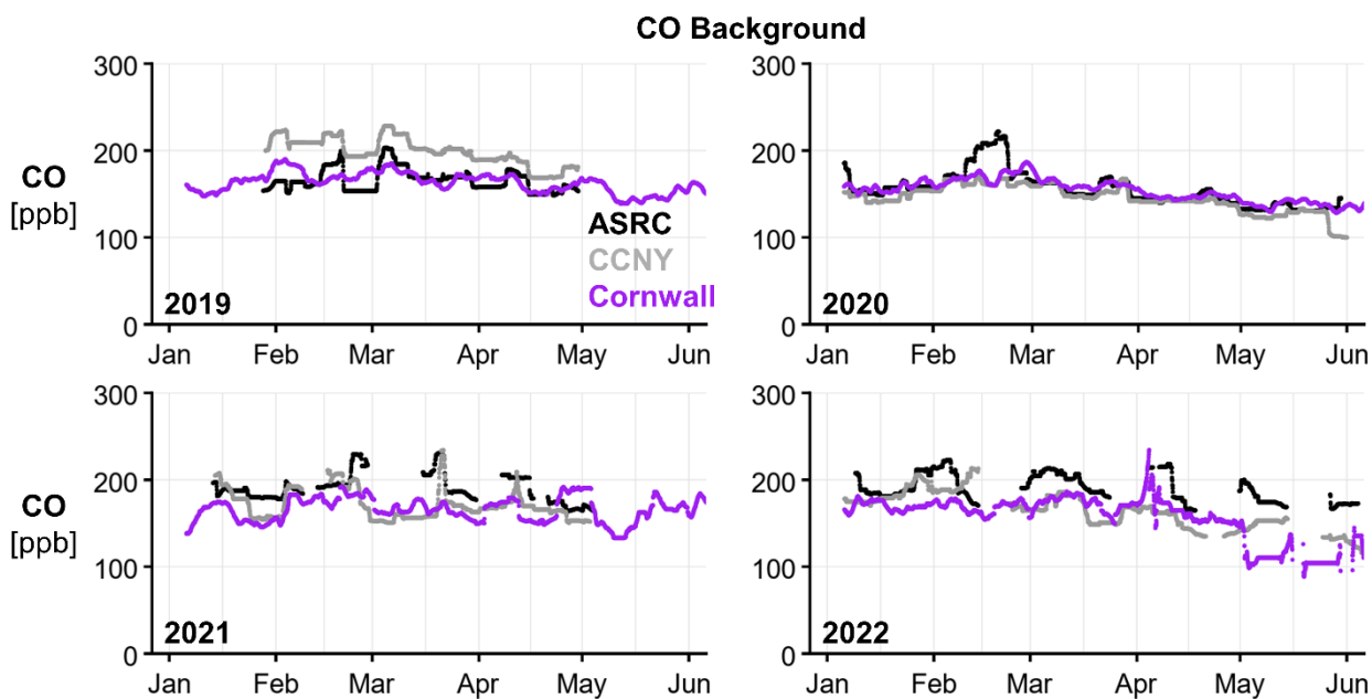
Figure S3. Timeseries of the CO backgrounds to the NYCMA for 2019-2022 using the 5 th percentile method at the ASRC (black) and CCNY (grey) sites and as the 10-day mean of observations at the Cornwall site (purple).
