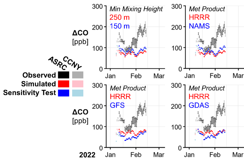
35 Figure S7. Timeseries of 10-day mean observed (black/grey) and simulated (red/pink) \Delta\text{CO} for the NYCMA domain at the ASRC (black/red) and CCNY (grey/pink) sites as in Fig. 2 during January–February 2022. Additional simulated \Delta\text{CO} from various sensitivity tests of STILT shown for the ASRC site in blue and the CCNY site in light blue: reducing minimum mixing height from 250 m to 150 m (upper left), using the NAMS (North American Mesoscale Forecast System) meteorological product to drive STILT instead of HRRR (High-Resolution Rapid Refresh) (upper right), using GFS (Global Forecast System) meteorology (lower left), and using GDAS (Global Data Assimilation System) meteorology (lower right). 40
