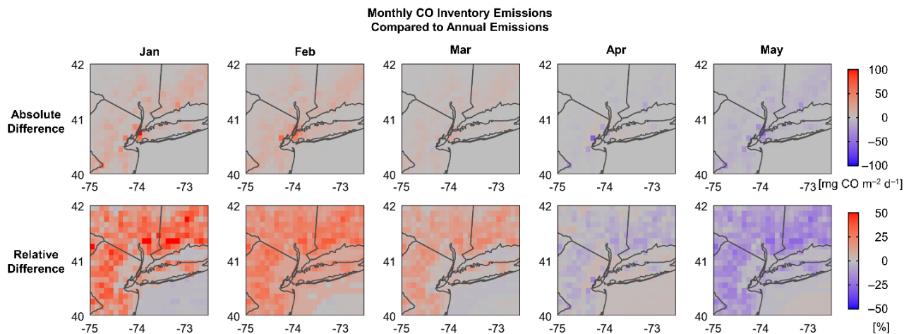
25 Figure S4. Monthly (January-May; left to right) EDGAR CO emissions compared to the annual mean EDGAR CO emissions for the NYCMA. The absolute difference (monthly–annual) is shown in the top row, while the relative difference (monthly/annual) is shown in the bottom row.
