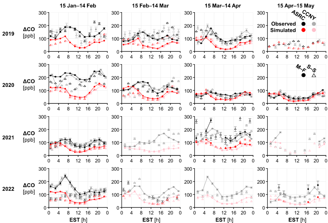
30 Figure S5. Diurnal time series of mean observed (black/grey) and simulated (red/pink) \Delta\text{CO} for the NYCMA domain at the ASRC (black/red) and CCNY (grey/pink) sites as in Fig. 3 for the time periods as shown: 15 January–14 February, 15 February–14 March, 15 March–14 April, 15 April–15 May (left to right) for 2019–2022 (top to bottom).
