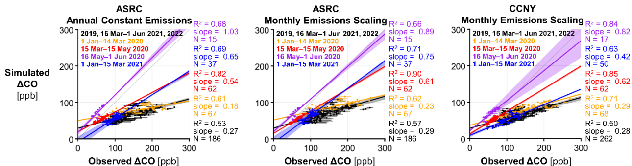
Figure S8. Comparison of observed and simulated \Delta\text{CO} as in Fig. 4a using: (i) ASRC observations and annual mean EDGAR CO emissions (left), (ii) ASRC observations and monthly EDGAR CO emissions (center, same as Figure 3a), and (iii) CCNY observations and monthly EDGAR CO emissions (right).
