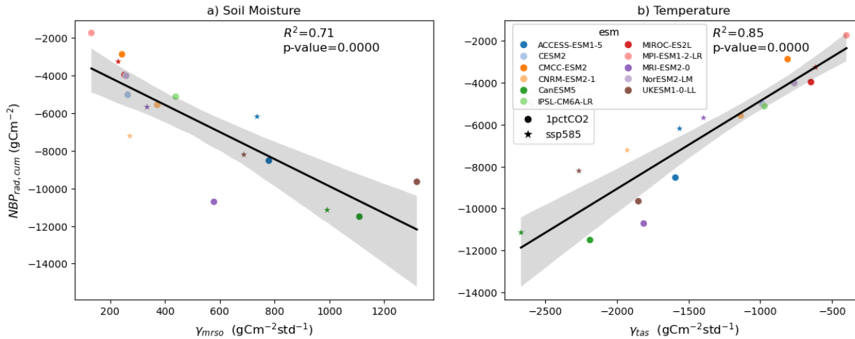
275 Figure 3: Intermodel uncertainty in climate-driven cumulative NBP (y-axis) as explained by differences in ESMs representation of temperature ( Y_{tas} ) and soil moisture ( Y_{mrso} ) impacts in 1pctCO2-rad and ssp585-rad simulations. The reported values are the zonally averaged within the Amazon basin geographical domain.
