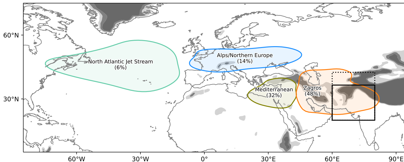
Figure 5. Regions of climatological WD cyclogenesis, computed using the WD track dataset described in Hunt (2024). Genesis points from all ~6000 winter WDs in the dataset are clustered into four groups using a simple k -means approach. A Gaussian kernel density estimate is then applied to each cluster, with the 90% contour plotted. Regions are labelled after upstream mountain ranges or water sources, with the figures in parentheses indicating the fraction of the total WD population with geneses in that region. Filled grey contours represent smoothed orography at heights of 1, 1.5, and 2 km. The black box indicates the commonly-used WD track-capture region used in some tracking studies (60–80°E, 20–36.5°N). The dotted box shows the extension to 42.5°N which has also been used in some more recent studies.
