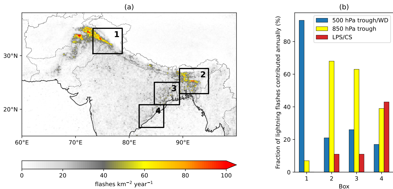
Figure 12. Following Unnikrishnan et al. (2021). (a) annual lightning frequency [flashes km -2 year -1 ] in the period 1998–2013, from the TRMM LIS-Lightning Imaging Sensor 0.1 Degree Very High Resolution Gridded Climatology (Albrecht et al., 2016). (b) fraction of lightning strikes in each of the boxes labelled in (a) associated with WDs [blue], low-level troughs [yellow], and low-pressure systems or cyclonic storms [red]. LPS = low-pressure system; CS = cyclonic storm.
