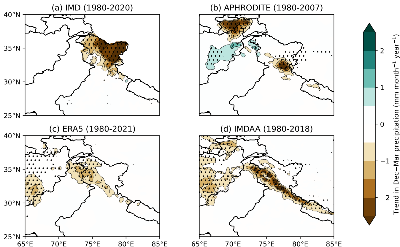
Figure 22. Trends in winter (DJFM) precipitation [ \text{mm month}^{-1} \text{ year}^{-1} ] over Pakistan and North India since 1980, as recorded in four datasets, two gridded gauge-based products: (IMD and APHRODITE), and two reanalyses (ERA5 and IMDAA). Stippling indicates where trends are significantly different from zero at the 95% confidence interval.
