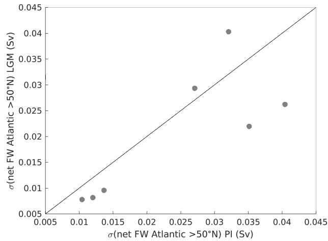
Figure B1. Interannual standard deviation of the net freshwater flux into the North Atlantic north of 50^\circ\text{N} as simulated by different PMIP3/4 models at the LGM (y-axis) versus the pre-industrial (PI) (x-axis).
