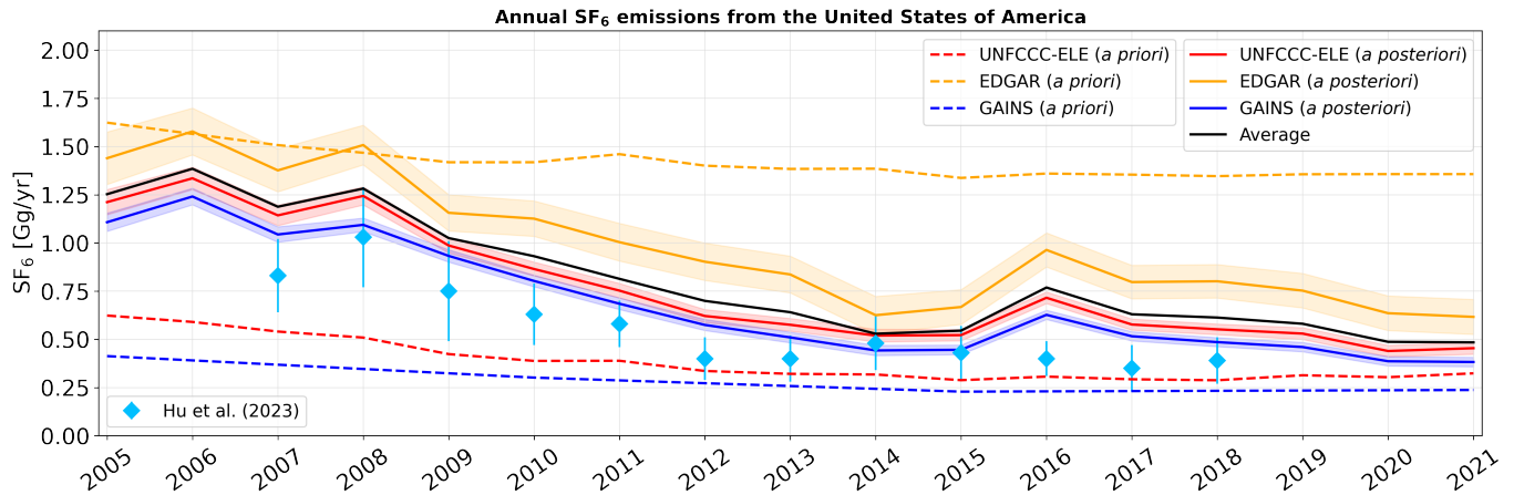
Figure 8. Annual a priori (dashed lines) and a posteriori (solid lines) SF 6 emissions in the U.S., shown for the period between 2005 and 2021 when using different a priori emissions-inventories (UNFCCC-ELE red, EDGAR orange, GAINS blue). A posteriori emissions are illustrated together with their respective \pm 1\sigma uncertainties (colored shadings, defined as the minimum and maximum 1\sigma uncertainty limits across the inversion results for different a priori variations ). The a posteriori emissions averaged over the inversion results using the different inventories are shown with a black solid line. The results of Hu et al. (2023) are shown with blue diamonds together with their respective 2\sigma uncertainties.
