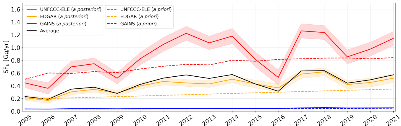
Figure A8. Annual a priori (dashed lines) and a posteriori (solid lines) \text{SF}_6 emissions from India, shown for the period between 2005 and 2021 when using different a priori emissions-emission inventories (UNFCCC-ELE red, EDGAR orange, GAINS blue). A posteriori emissions are illustrated together with their respective 1\text{-}\sigma uncertainties (colored shadings, defined as the minimum and maximum 1\text{-}\sigma uncertainty limits across the inversion results for different a priori variations ). The a posteriori emissions averaged over the inversion results using the different inventories are shown with a black solid line.
