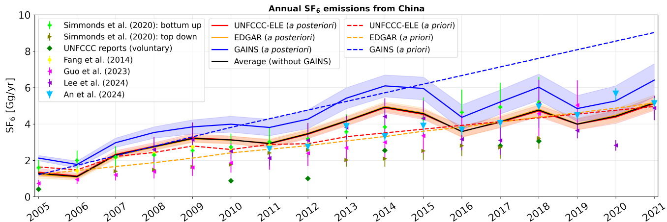
Figure 10. Annual a priori (dashed lines) and a posteriori (solid lines) SF 6 emissions from China, shown for the period between 2005 and 2021 when using different a priori emissions-emission inventories (UNFCCC-ELE red, EDGAR orange, GAINS blue). A posteriori emissions are illustrated together with their respective 1-\sigma uncertainties (colored shadings, defined as the minimum and maximum 1-\sigma uncertainty limits across the inversion results for different a priori variations). The a posteriori emissions averaged over the inversion results using EDGAR and UNFCCC-ELE are shown with a black solid line.
