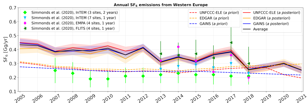
Figure A5. Annual a priori (dashed lines) and a posteriori (solid lines) SF 6 emissions from Western Europe, shown for the period between 2005 and 2021 when using different a priori emissions-emission inventories (UNFCCC-ELE red, EDGAR orange, GAINS blue). A a posteriori emissions are illustrated together with their respective \pm 1\sigma uncertainties (colored shadings, defined as the minimum and maximum 1\sigma uncertainty limits across the inversion results for different a priori variations ). The a posteriori emissions averaged over the inversion results using the different inventories are shown with a black solid line. Further, the results from Simmonds et al. (2020) are shown, using four different inversion setups.
