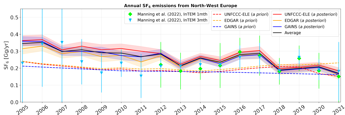
Figure A4. Annual a priori (dashed lines) and a posteriori (solid lines) SF 6 emissions from North-West Europe, shown for the period between 2005 and 2021 when using different a priori emissions-emission inventories (UNFCCC-ELE red, EDGAR orange, GAINS blue). A a posteriori emissions are illustrated together with their respective \pm 1\sigma uncertainties (colored shadings, defined as the minimum and maximum 1\sigma uncertainty limits across the inversion results for different a priori variations ). The a posteriori emissions averaged over the inversion results using the different inventories are shown with a black solid line. The blue rectangles and the green diamonds represent the results from Manning et al. (2022) using the InTEM (Inversion Technique for Emissions Modelling) model with inversion time frames set to 3- and 1-months, respectively
