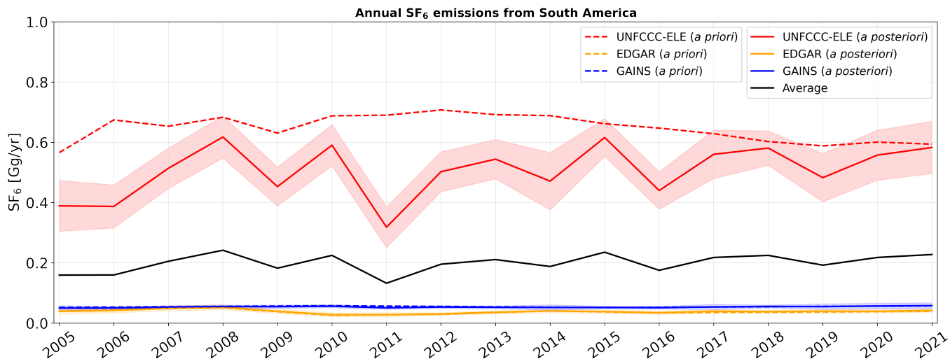
Figure A6. Annual a priori (dashed lines) and a posteriori (solid lines) SF 6 emissions from South America, shown for the period between 2005 and 2021 when using different a priori emissions-emission inventories (UNFCCC-ELE red, EDGAR orange, GAINS blue). A a posteriori emissions are illustrated together with their respective 1-\sigma uncertainties (colored shadings, defined as the minimum and maximum 1-\sigma uncertainty limits across the inversion results for different a priori variations ). The a posteriori emissions averaged over the inversion results using the different inventories are shown with a black solid line.
