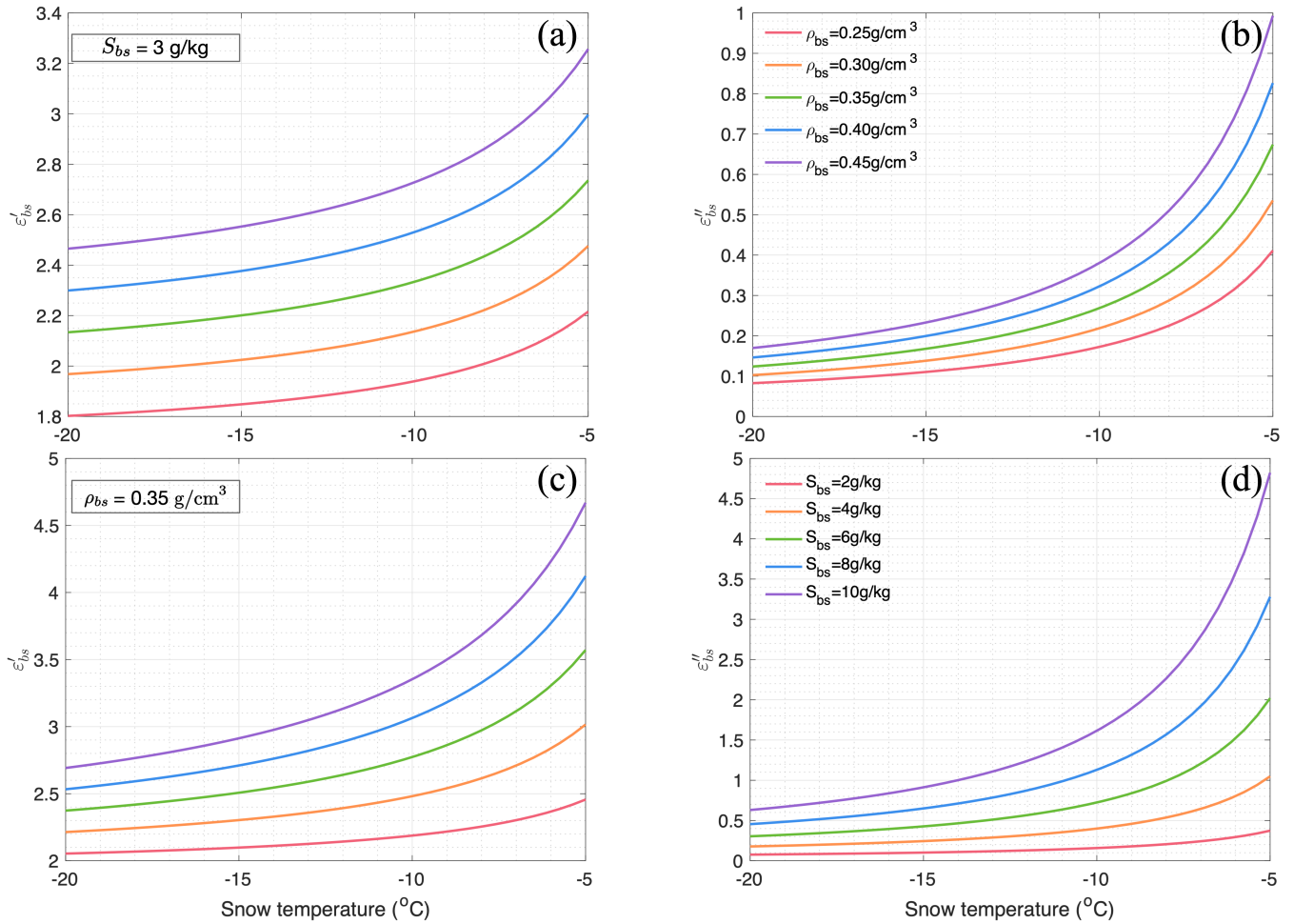
Figure B.9. Real ( \epsilon'_{bs} ): (a) and (c) and imaginary ( \epsilon''_{bs} ): (b) and (d) parts of complex dielectric constant of brine-wetted snow changes with the snow temperature for different snow density (Constant: S_{bs} = 3 \text{ g kg}^{-1} (a) and (b)) and salinity (Constant: \rho_{bs} = 0.35 \text{ g cm}^{-3} (c) and (d)).
