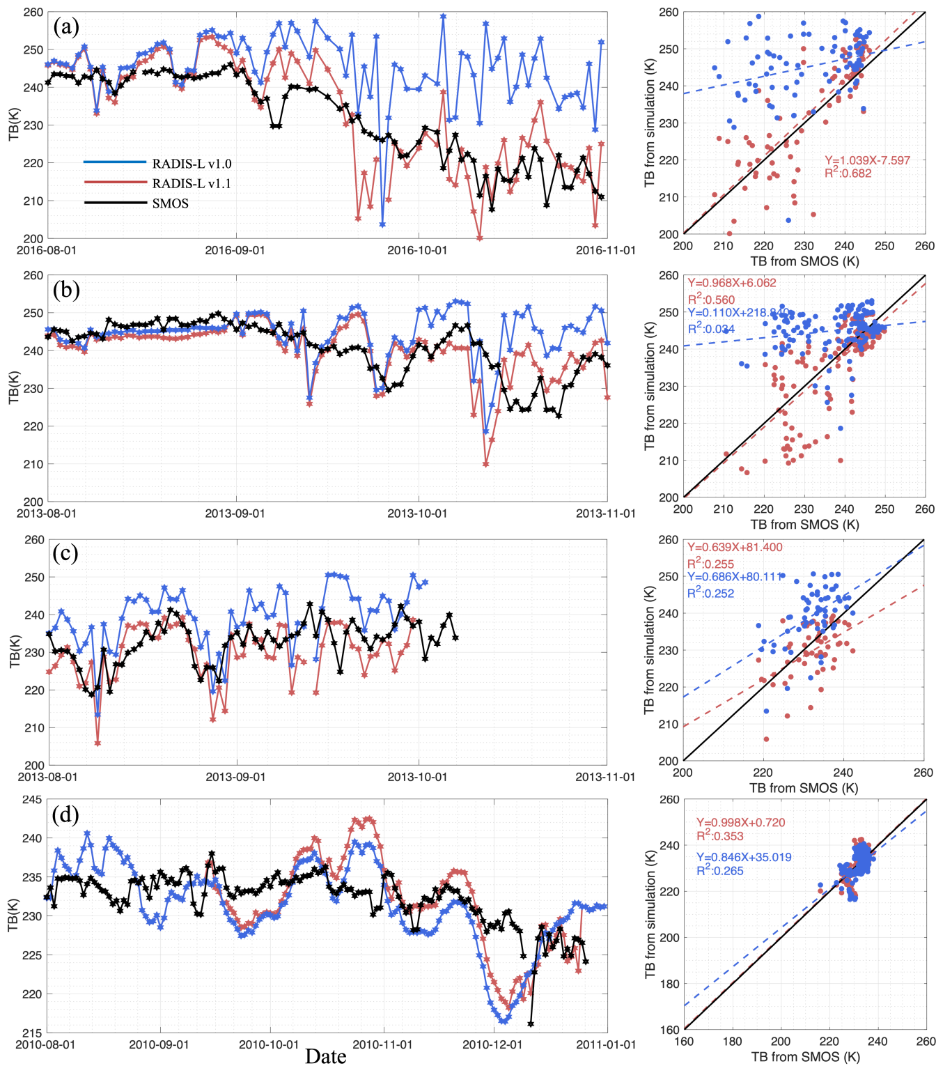
Figure 4. The mean of horizontal and vertical polarised Tbs comparison from SMOS and simulated from RADIS-L v1.0 and RADIS-L v1.1 along the buoy trajectories and scatters fittings in (a) AWI 2016S31, (b) PS81/506, (c) PS81/517, and (d) ZS-2010 buoy.
