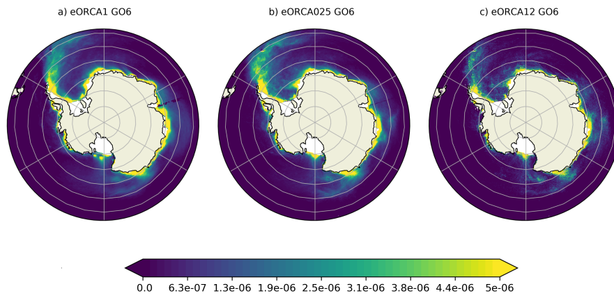
Figure S1. Annual mean of fresh water flux ( \text{kg}\cdot\text{m}^{-2}\cdot\text{s}^{-1} ) from iceberg melt calculated from G06 integrations.
