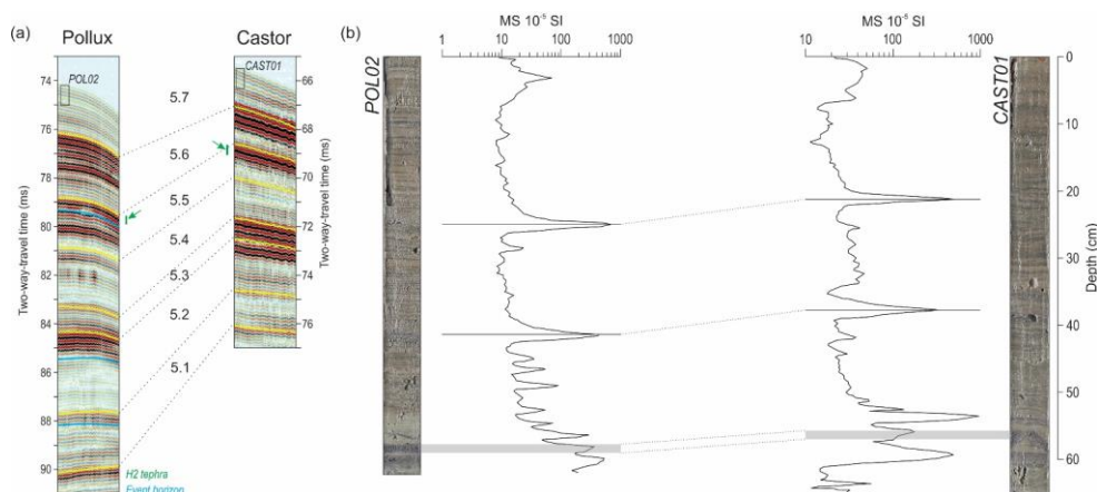
Figure 6. (a) Seismic section of Unit 5 showing all seven subunits identified on a pingar seismic profile in Lago Pollux (Fig. 2b) and Lago Castor (after Van Daele et al., 2016). (b) Correlation of two short cores from Lago Pollux (POL02) and Lago Castor (CAST01) with plotted MS data, showing two distinct peaks. At the base, a ~1.5 cm thick tephra in both cores is indicated in grey.
