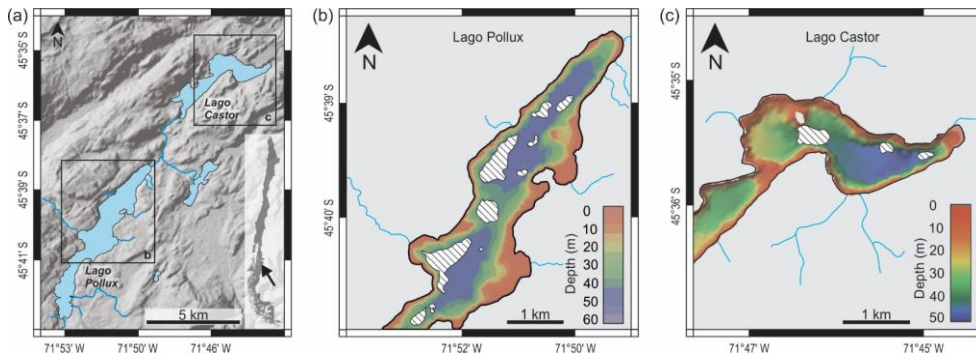
Figure 7. (a) SRTMGLIN terrain data (NASA JPL, 2013) of the area around Lago Pollux and Lago Castor. (b, c) Spatial distribution of the mass transport deposits (MTDs; the hatched shapes) identified in Unit 5.5 under the H2 tephra deposit for both Lago Pollux (b) and Lago Castor (c). Note that the distribution of MTDs in the southern part of Lago Pollux could not be mapped due to shallow bathymetry and limited seismic penetration, and that no MTDs were identified in the southwestern part of Lago Castor.
