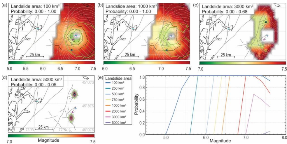
Figure 9. (a-d) Maps (modified after SERNAGEOMIN, 2003) showing the area (plotted in Figure 1a) in which an earthquake could have caused the observed pattern of sedimentological imprints in Lago Pollux, Lago Castor and Aysén Fjord (positive and negative evidence), considering an area of 100 (a), 1000 (b), 3000 (c) or 5000 (d) km 2 that was affected by landslides. Fault traces are mapped after SERNAGEOMIN (2003). The magnitude with the highest probability at each location is given in a green-to-red color scale. White dashed lines correspond to the probability; green line and enclosed hatched area mark the region where the probability is less than 0.1 below the maximum probability, highlighting the most likely epicentral region (indicated by a star). Sites of positive (plus) and negative (minus) evidence are shown in semitransparent magenta and cyan colors, respectively. Note that sites with both positive and negative evidence show a bluish color. (e) The maximum probability of an earthquake in the study area (independent of its location) with a magnitude ranging between 5 and 7.6 to have caused the observed pattern of sedimentological imprints in the Río Aysén catchment that were affected by landslides.
