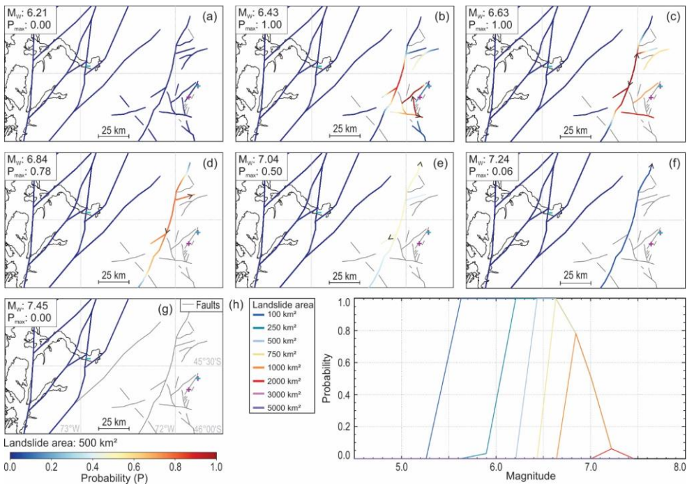
Figure 10. (a-g) Maps (modified after SERNAGEOMIN, 2003) showing all faults in the study area (plotted in Figure 1a), color-coded according to the probability that an earthquake of magnitude 6.21 (a), 6.43 (b), 6.63 (c), 6.84 (d), 7.04 (e), 7.24 (f), 7.45 (g) on each of the fault sections is capable of causing the observed spatial distribution of sedimentary earthquake evidence and by considering an area of 500 km 2 that has been affected by landslides. Fault traces are mapped after SERNAGEOMIN (2003). Arrows indicate the limits of the rupture trace resulting in the highest probability. Grey fault traces are not sufficiently long to cause a rupture with the tested magnitude. Sites of positive (plus) and negative (minus) evidence are shown in semitransparent magenta and cyan colors, respectively. Note that sites with both positive and negative evidence show a bluish color. (h) The maximum probability of an earthquake on any of the faults in the study area with a magnitude ranging between 5 and 7.6 to have caused the observed pattern of sedimentological imprints in Lago Pollux, Lago Castor and Aysén Fjord (positive and negative evidence), considering a range of minimum areas (100-5000 km 2 ) in the Río Aysén catchment that were affected by landslides.
