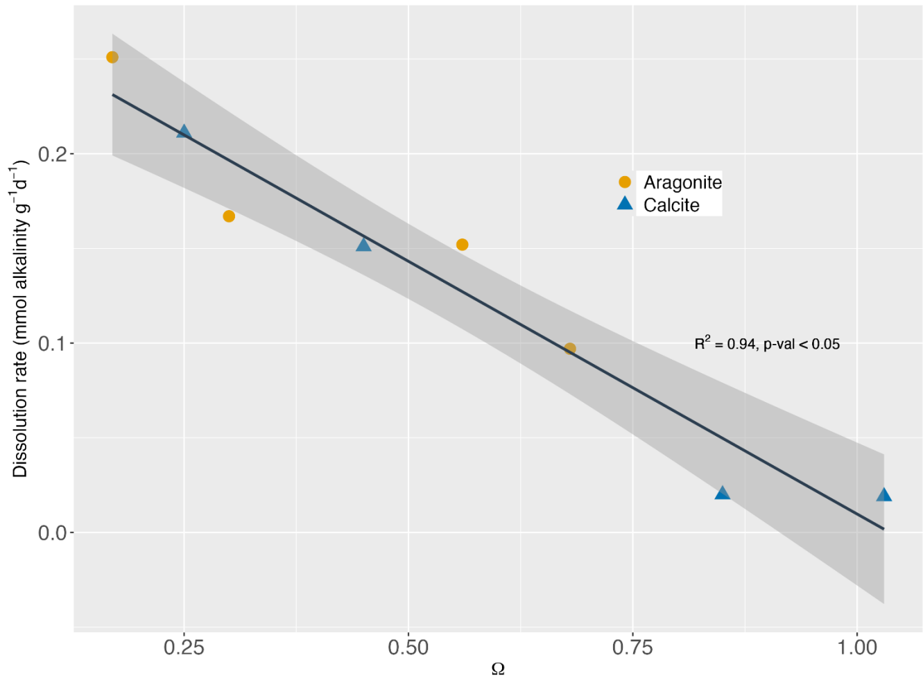
250 Figure 1: Saturation state for aragonite and calcite vs. their respective dissolution rates (mmol alkalinity g_{\text{solid}}^{-1} d^{-1} ). Line show the fit with n=1 . R^2 : coefficient of determination. p-val: statistical significance of the fit. Shaded area represents 95% confidence interval.
