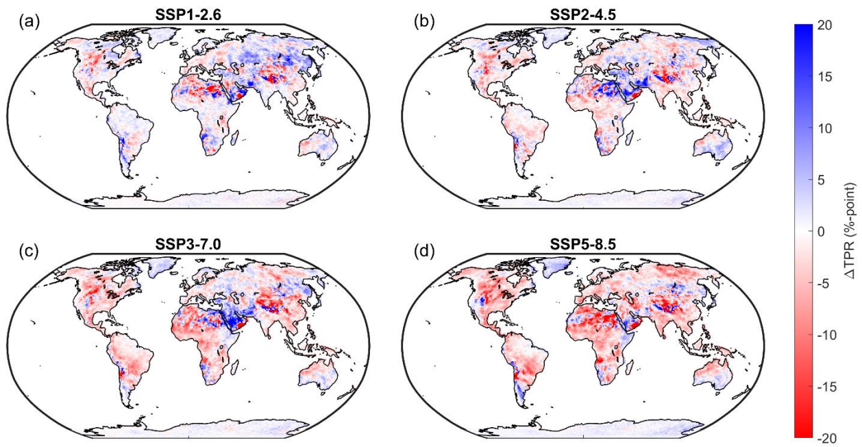
Figure 2. Differences in relative annual terrestrial precipitation recycling ratio ( \Delta TPR) across the globe between the baseline period (2015–2024) and the end of the century (2090–2099) in percentage points, for (a) SSP1-2.6, (b) SSP2-4.5, (c) SSP3-7.0, and (d) SSP5-8.5. Positive values indicate an increase in precipitation recycling ratio and negative values a decrease. Both significant and non-significant differences are shown. Color scales are truncated at -20 percentage points and 20 percentage points.
