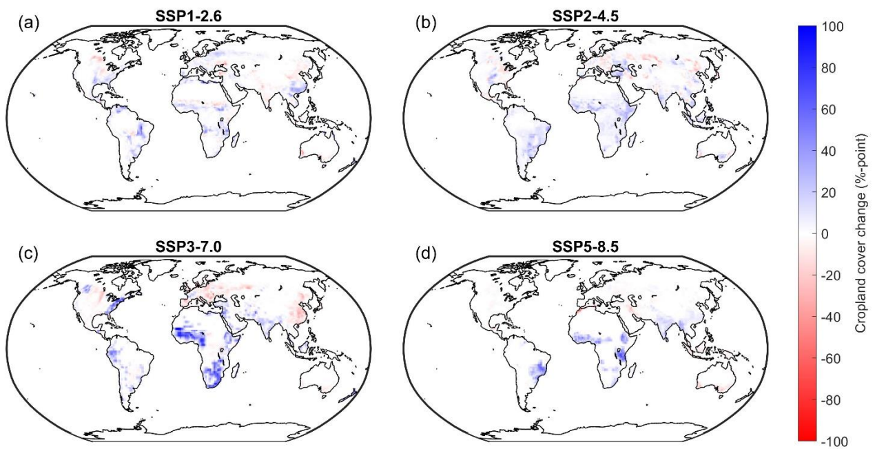
630 Figure A4. Differences in cropland cover (%-point) between the baseline period (2015–2024) and the end of the century (2090–2099) for (a) SSP1-2.6, (b) SSP2-4.5, (c) SSP3-7.0, and (d) SSP5-8.5.
