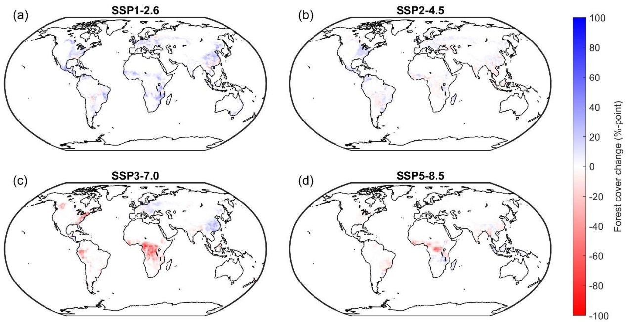
625 Figure A3. Differences in forest cover (%-point) between the baseline period (2015–2024) and the end of the century (2090–2099) for (a) SSP1-2.6, (b) SSP2-4.5, (c) SSP3-7.0, and (d) SSP5-8.5.
