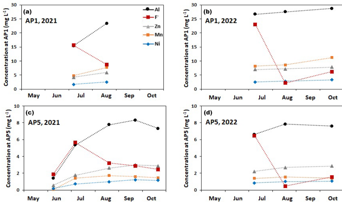
Figure 5. Seasonal variation in the concentrations of Al, F - , Zn, Mn, and Ni at the rock glacier spring AP1 and the upstream discharge monitoring location AP5 (Fig. 1). (a, b) Interpolation of solute concentrations of samples taken at AP1 in 2021 and 2022, respectively. (c, d) Interpolation of solute concentrations of samples taken at AP5 in 2021 and 2022, respectively.
