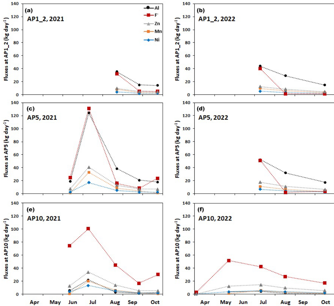
Figure 6. Interpolated fluxes of Al, F - , Zn, Mn, and Ni at the three main monitoring stations along the Aua da Prasūra stream. (a, b) Fluxes measured at the AP1_2 location in 2021 and 2022. (c, d) Fluxes measured at the upstream AP5 location in 2021 and 2022. (e, f) Fluxes measured at the downstream AP10 location in 2021 and 2022.
