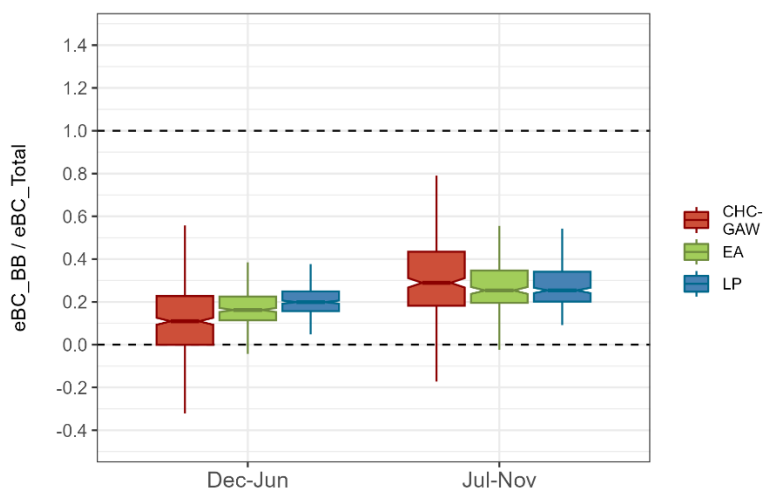
Figure 7. Box whiskers plot of the daily eBC_{BB}/eBC_{TOT} at 950 nm resulting from the bilinear Aethalometer method displaying maximum contributions during the biomass burning season (Jul-Nov). The horizontal bar in each box represents the median value. The lower (upper) hinge represents the percentile 25 (75), and the lower (upper) whiskers represent the smallest (largest) observation greater (less) than or equal to lower (upper) hinge \pm 1.5 times the interquartile range (IQR).
