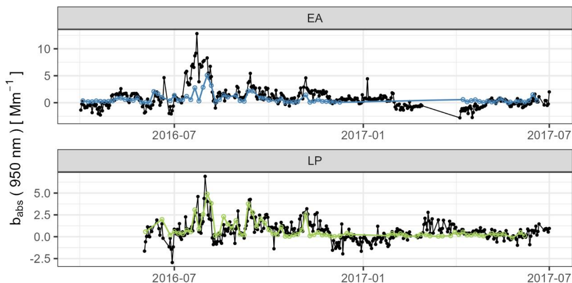
720 Figure 10. Timeseries of the contribution of agricultural biomass burning to the absorption coefficients at 950 nm measured at the two urban background sites (LP and EA) using two different apportioning methods: Aethalometer method (black lines, using AAE_{\text{TR}}=1 and AAE_{\text{BB}}=1.5 , percentiles (1,99)) and MLR deconvolution from the mass contribution of \text{PM}_{10} sources resolved by Mardoñez et al. (2023) (colored lines).
