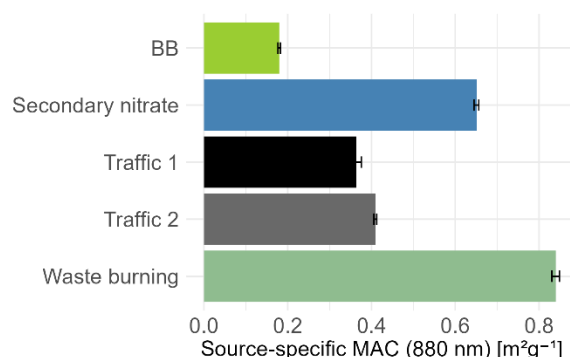
655 Figure 8. Median source-specific mass absorption cross sections ( \beta ) obtained from the multisite MLR between b_{\text{abs}} (880 nm) and the mass contribution of the six sources of \text{PM}_{10} , resolved by Mardoñez et al. (2023), that significantly contributed to the measured absorption coefficients. The black error bars represent the 95% CI of the median of the 500 bootstrap runs.
