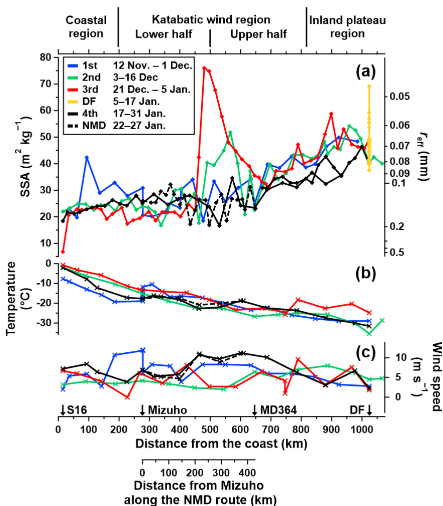
405 Figure 6: In situ measured (a) 10-surface mean SSA at each observation site, (b) Air temperature around noon, and (c) wind speed around noon during the four traverses between S16 and Dome Fuji and the stay at Dome Fuji.
