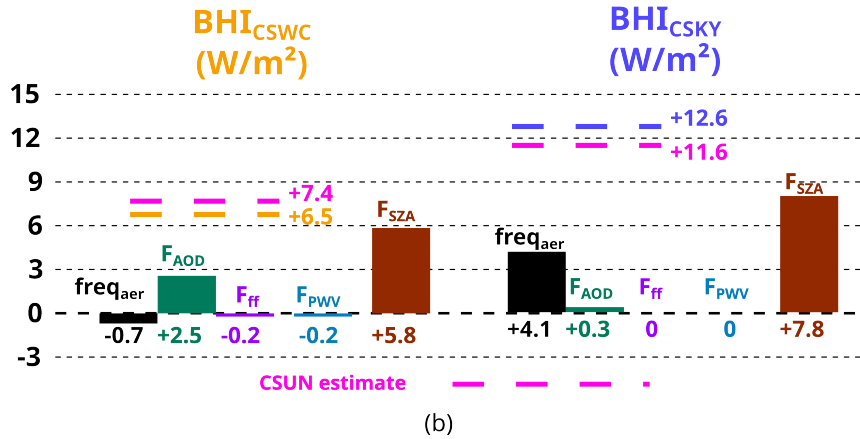
Figure 7. Illustration of the decomposition for spring 2020 : (a) of the all-sky SSI components (GHI, BHI, and DHI), and (b) of the direct component (BHI) in clear-sun with clouds and clear-sky conditions. In Figure (a), the green dashed lines represent the observed deviation from the 2010-2022 spring average for spring 2020. The red dashed lines correspond to the deviation derived from the decomposition based on the sky conditions. The decomposition is represented by the black, gray, orange, and blue colored columns, which respectively correspond to the contributions of the variability in the frequency of occurrence of sky conditions ( freq_{cond} ) and the intrinsic variability of the irradiances in CLOS ( F_{CLOS} ), CSWC ( F_{CSWC} ), and CSKY ( F_{CSKY} ) conditions. The additional decomposition of BHI_{CSWC} and BHI_{CSKY} with respect to the scene's parameters is illustrated in panel (b). The orange and blue columns from panel (a), which represent the intrinsic variability of the BHI under CSWC and CSKY conditions, respectively, are represented as dashed lines of the same color in panel (b). The pink dashed lines represent the values estimated from the decomposition of the BHI according to the scene's parameters as in Equation 6. The latter decomposition is also illustrated by the colored columns, which represent the contributions of the variability in the frequency of occurrence of aerosol classes ( freq_{aer} , black column), as well as the variability of the AOD (green column), ff (violet column), PWV (blue column), and SZA (brown column).
