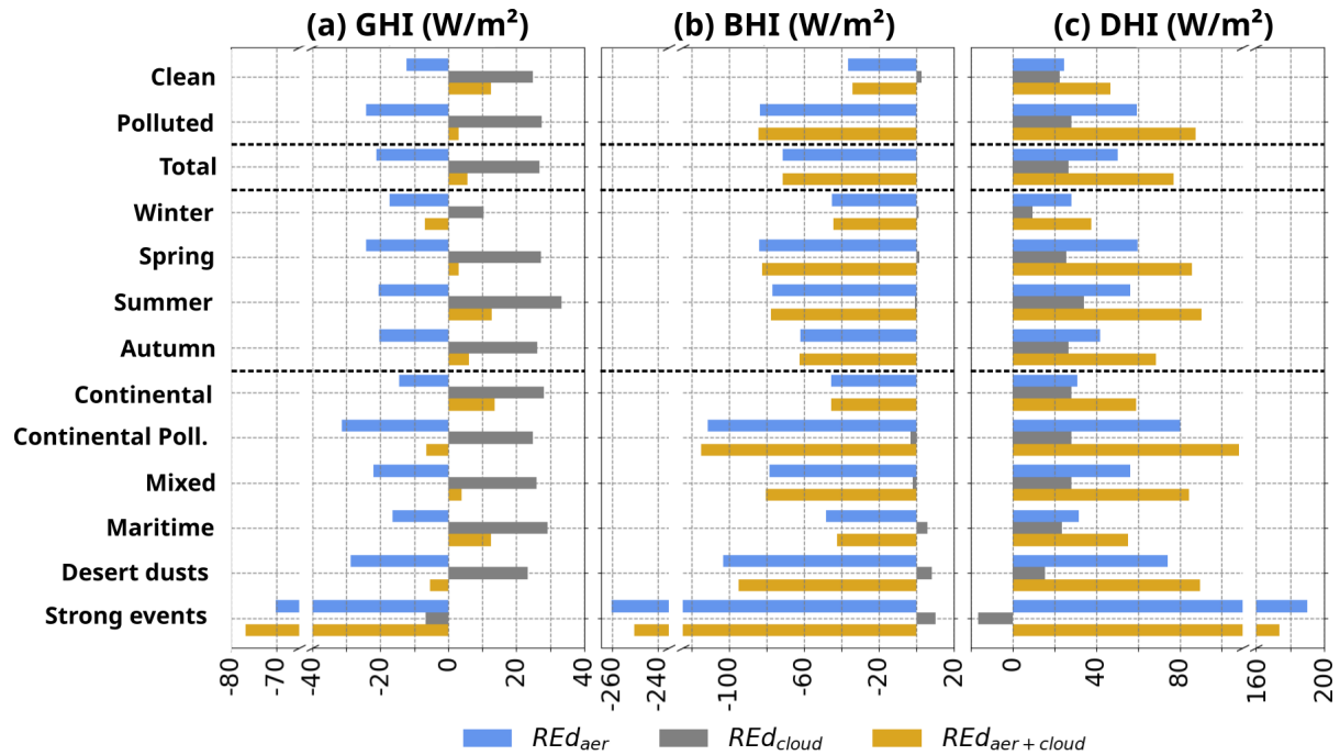
Figure 10. Mean RE_d on SSI, under CSWC conditions, of aerosols and clouds combined (yellow), clouds (gray), and cloud free RE_d of aerosols (blue), on SSI for (a) the global (GHI), (b) the direct (BHI), and (c) the diffuse (DHI) components over the period 2010-2022. Points considered as the ones coincident AERONET measurements. Instantaneous values are calculated using ATOLL SSI measurements and SOLARTDECO clear-sky simulations with and without aerosols. As in Table 5, the "total" averages correspond to the overall mean RE_d over the period 2010-2022.
