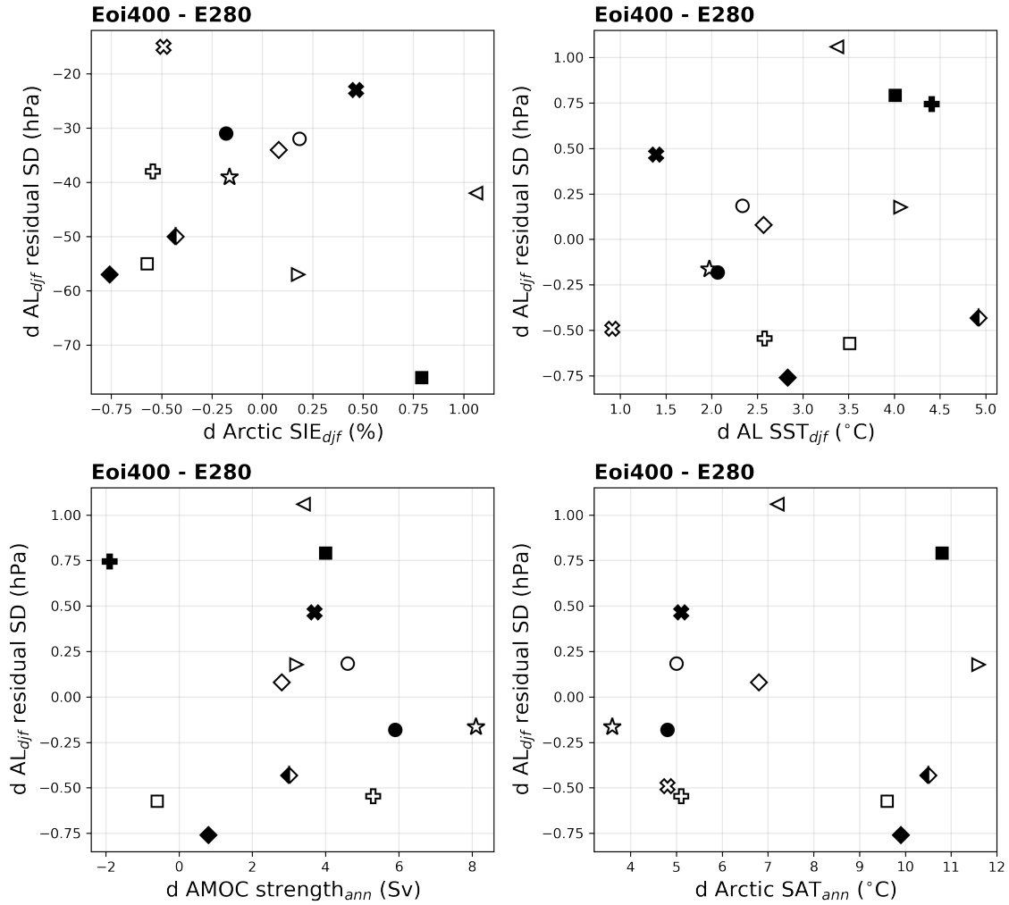
Figure S6: Change (Eoi400 - E280) in the residual DJFM AL variability (i.e. the part of the variability that is not linearly correlated to ENSO) as a function of: (top left) relative change in Arctic sea-ice extent in DJF (SIE); (top right) absolute change in sea-surface temperatures (SST) averaged in the AL region in DJF; (bottom left) absolute change in annual mean AMOC strength; and (bottom right) absolute change in annual mean Arctic surface air temperatures (SAT). None of the ensemble scatters show a significant correlation.
