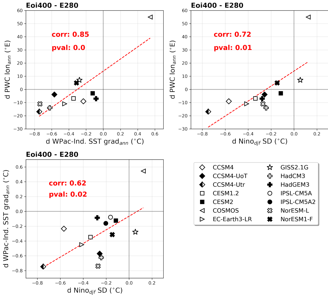
Figure S7: Scatter plots of three changes between the mid-Pliocene and pre-industrial simulations (Eoi400 - E280). Change in the central longitude of the Pacific Walker circulation (PWC) in the annual mean (d PWC lon), Change in the SST difference between the tropical West Pacific Ocean and Indian Ocean in the annual mean (d Indo-Pac SST grad), and Change in the winter ENSO amplitude (d Nino SD). The three scatter plots show the three possible combinations of two of these changes. All combinations between these variables yield a significant ensemble correlation.
