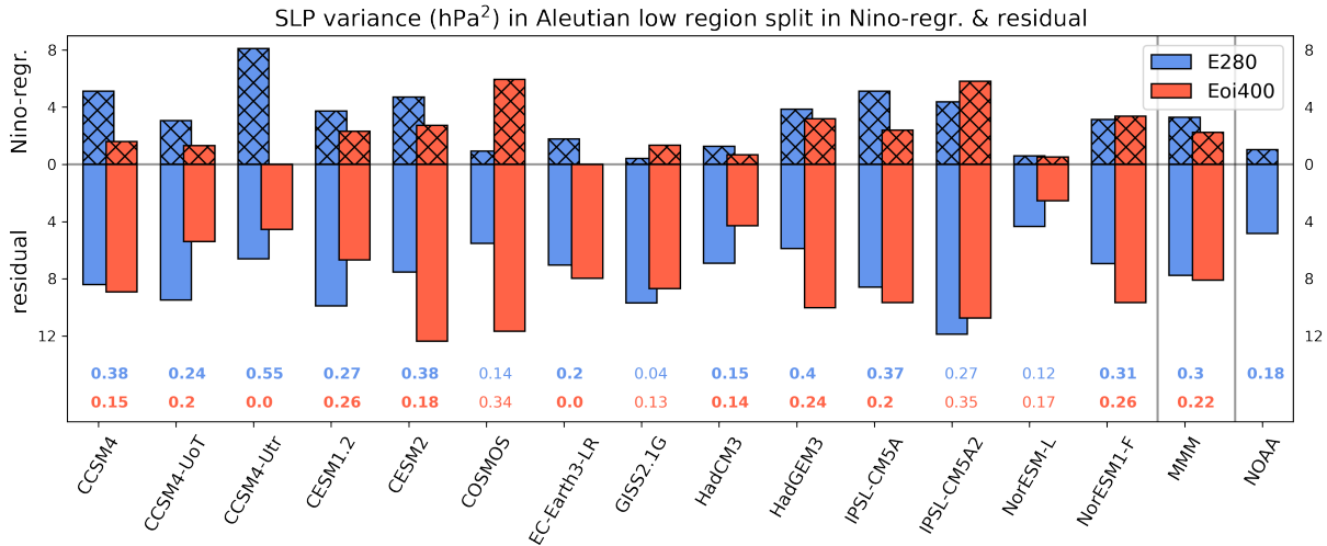
Figure 5. Aleutian low (AL) variance split (following a linear regression model, LRM) in AL variance that regresses with Niño (Niño-regr. part , hatched) and the residual AL variance. Per model for the E280 (blue) and Eoi400 (red), including multi-model mean (MMM) and result from NOAA observations. Full bar length represents total AL variance. Values below are the variance fraction of the Niño-regr. part, for E280 (blue, top) and Eoi400 (red, bottom), in bold when the variance fraction is lower in the Eoi400 compared to the E280.
