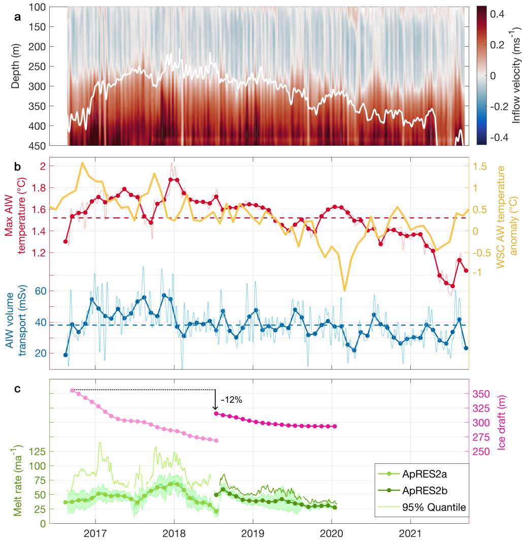
Figure 13. Evolution of the AIW inflow to the cavity below 79NG. (a) Inflow (red)/outflow (blue) velocities recorded by a mooring deployed at the 79NG calving front (Fig. 4). The white line is the depths of the 1 °C isotherm. (b) Timeseries of weekly and monthly maximum AIW temperature (red), near-surface mean AW temperature anomaly in the WSC (eastern Fram Strait) from mooring observations (yellow), and AIW volume transport (blue) into the cavity. Dashed horizontal lines are the respective mean values. (c) Local ice draft (pink) and basal melt rate (green) timeseries of the ApRES measurements (monthly means). The two deployments were between 2016–2018 (lighter colours) and 2018–2020 (darker colours) (Methods). The shaded area around the melt rates marks the range between the 25% and 75% quantile, and the thin line the 95% quantile. Note that the maximum grounding depth of the 79NG slightly exceeds 600 m (Zeising et al., 2024), while the ice draft shown here corresponds to the local ice draft at the position of the instrument. Figure adapted from McPherson et al. (2024).
