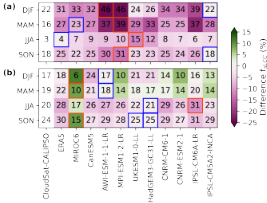
Figure 4. Magnitude of seasonal area-weighted averages (between 145^{\circ} - 82^{\circ} ) of f_{sLCC} for CloudSat-CALIPSO, ERA5, CMIP6 models (numbers). The heatmap colors correspond to the differences of area-weighted averages of f_{sLCC} between CloudSat-CALIPSO and ERA5 and CMIP6 models. Green (pink) values indicate underestimation (overestimation) of the individual model with respect to CloudSat-CALIPSO. (a) for the mid-to-high latitude NH, and (b) for the mid-to-high latitude SH. Per season, the smallest (largest) seasonal and spatial differences are outlined with blue (red) lines.
