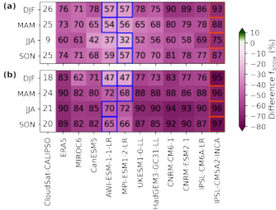
Figure 8. Magnitude of seasonal area-weighted averages (between 145^{\circ} - 82^{\circ} ) of f_{\text{snow}} for CloudSat-CALIPSO, ERA5, CMIP6 models (numbers). The heatmap colors correspond to the differences of area-weighted averages of f_{\text{snow}} between CloudSat-CALIPSO and ERA5 and CMIP6 models. Green (pink) values indicate underestimation (overestimation) of the individual model with respect to CloudSat-CALIPSO. (a) for the mid-to-high latitude NH, and (b) for the mid-to-high latitude SH. Per season, the smallest (largest) seasonal and spatial differences are outlined with blue (red) lines.
