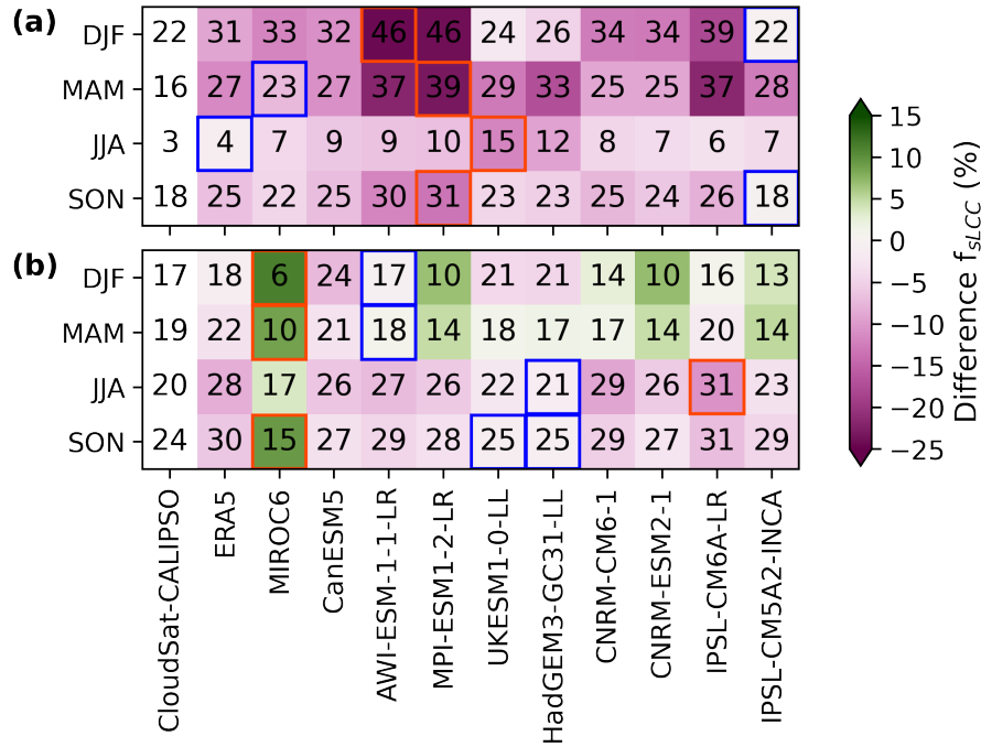
Figure 4. Seasonal-Magnitude of seasonal area-weighted averages (between 145^{\circ} - 82^{\circ} ) of f_{sLCC} for CloudSat-CALIPSO, ERA5, CMIP6 models (numbers). The heatmap colors correspond to the absolute differences of area-weighted averages of f_{sLCC} between CloudSat-CALIPSO and ERA5 and CMIP6 models. Green (pink) values indicate underestimation (overestimation) of the individual model with respect to CloudSat-CALIPSO. (a) for the mid-to-high latitude NH, and (b) for the mid-to-high latitude SH. Per season, the smallest (largest) absolute seasonal and spatial differences are outlined with blue (red) lines.
