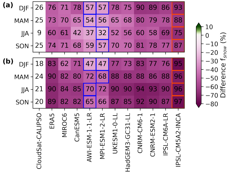
Figure 8. Seasonal-Magnitude of seasonal area-weighted averages (between 145^{\circ} - 82^{\circ} ) of f_{\text{snow}} for CloudSat-CALIPSO, ERA5, CMIP6 models (numbers). The heatmap colors correspond to the absolute -differences of area-weighted averages of f_{\text{snow}} between CloudSat-CALIPSO and ERA5 and CMIP6 models. Green (pink) values indicate underestimation (overestimation) of the individual model with respect to CloudSat-CALIPSO. (a) for the mid-to-high latitude NH, and (b) for the mid-to-high latitude SH. Per season, the smallest (largest) absolute -seasonal and spatial differences are outlined with blue (red) lines.
