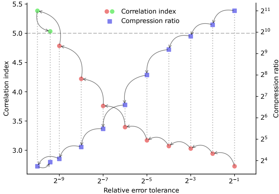
Figure 1. Illustration of how the bisection method works to find the optimal parameter. The circles represent the correlation indices corresponding to each parameter, with red circles indicating that the correlation index does not meet the defined threshold, and green circles indicating that the index fulfills the requirement. The arrows represent a step of the algorithm. In this case, we are using SZ2 with the relative error mode. Since the parameter range goes from 0 to 1, we perform the first evaluation at the middle of this range and continue adjusting the parameter until the correlation index value falls within the defined threshold (indicated by a dotted horizontal line). The variable temperature at 2 meters above the surface from the ERA5 dataset was used.
