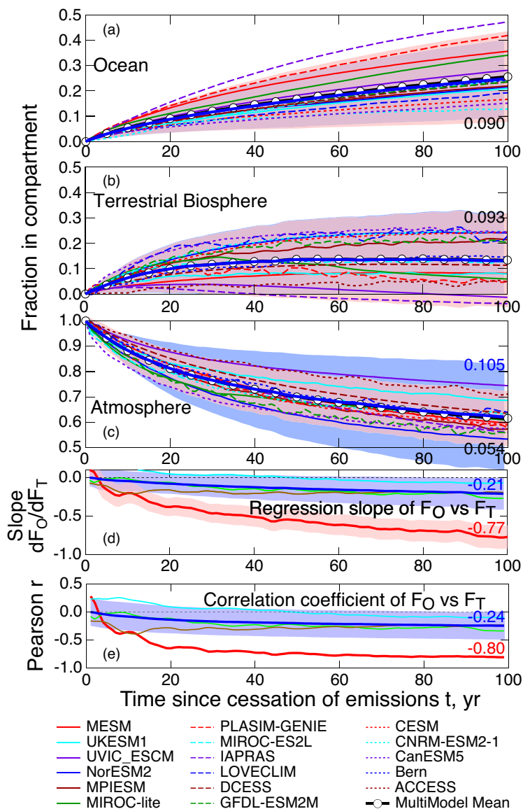
Figure 4. Time dependence of the fraction of excess atmospheric CO 2 (above preindustrial) at the time of cessation of anthropogenic emissions taken up by (a), the world ocean, and (b), the terrestrial biosphere, and (c), remaining in the atmosphere, subsequent to abrupt cessation of emissions, f_O , f_T , and f_A , respectively, as calculated by the
