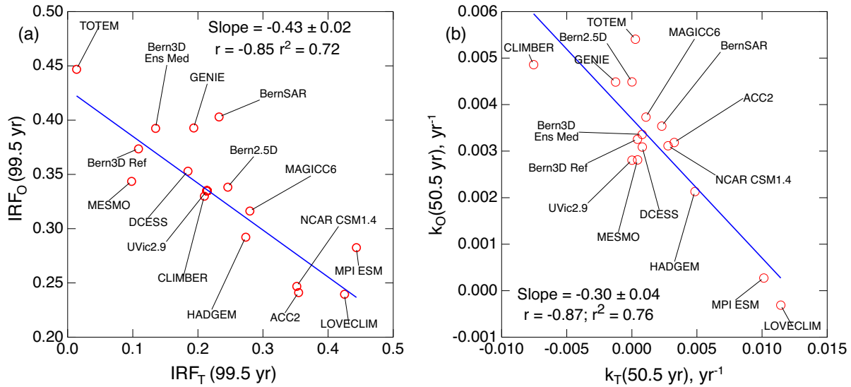
60 Figure 2. (a). IRF for uptake of excess CO 2 by the world ocean versus that by the terrestrial biosphere, both given as fraction relative to the magnitude of the pulse, at time t = 99.5 years subsequent to pulse injection, as represented by the models that participated in the model intercomparison study of Joos et al. (2013, J13). Blue line denotes linear regression; also shown are the regression slope; the Pearson correlation coefficient r , the negative value of which denotes anticorrelation; and r^2 , the fraction of the variance that is accounted for by the regression. For identification
