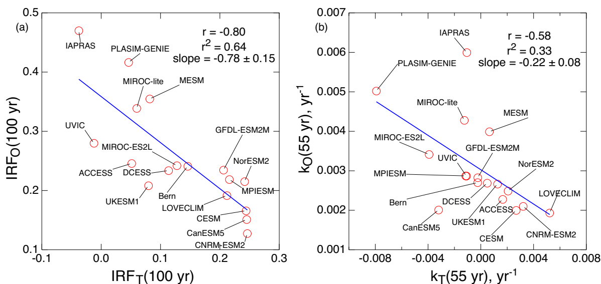
65 Figure 5. (a). Net uptake of CO 2 in the world ocean IRF O versus that in the terrestrial biosphere IRF T , both expressed as fraction of excess atmospheric CO 2 (i.e., above preindustrial) at the time of cessation of emissions, at time t = 100 years subsequent to cessation of anthropogenic emissions, as represented by the models that participated in the ZECMIP
