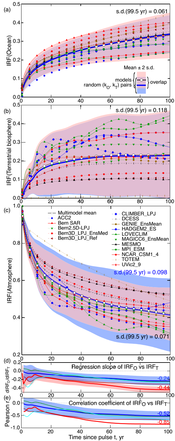
Figure 1. Time dependent impulse response functions (IRF's, f ) for the perturbations in stocks in (a), the world ocean f_O ; (b), the terrestrial biosphere f_T ; and (c), the global atmosphere f_A , as a function of time t subsequent to emission of
