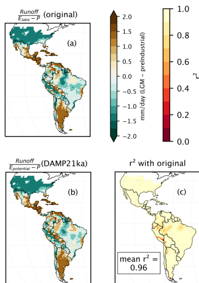
355 Figure 4: Comparison of lake status PSM equations. Lake status was calculated using runoff and precipitation data of CCSM4 simulations and different evaporation values. (a) Mean LGM minus preindustrial lake status values using lake evaporation data calculated from these simulations by Lowry and Morrill (2019). (b) The same values calculated using E_{\text{potential}} as in this study (c) For each gridcell, an we calculate an r^2 value between the two methods using all 200 annual values. A scatterplot of these values is shown by Fig. S4.
