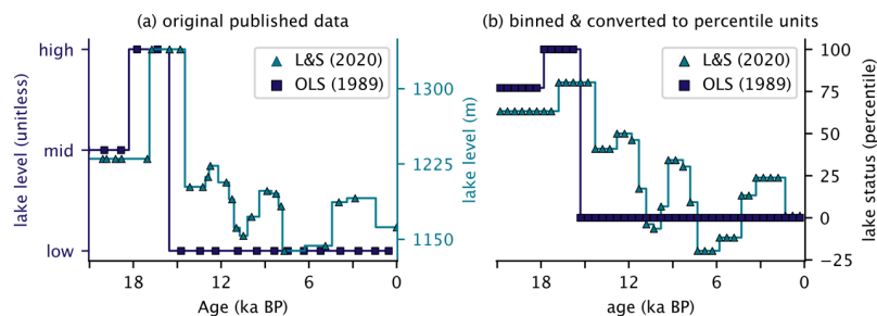
Figure 2: Data pre-processing for two lake records from Pyramid Lake, Nevada, USA. The record from the Oxford lake status data bank is shown by purple squares (Broecker and Orr, 1958; Street-Perrott et al., 1989). These data were superseded by a newer record (Benson et al., 1990; Briggs et al., 2005) compiled by Liefert and Shuman (2020) which is shown as teal triangles. (a) The original data for the two records. (b) The same records standardized to a common time axis using a nearest neighbor interpolation and converted percentile unit for assimilation. The mean value during the 11.7–0 ka reference period is then subtracted from each record.
