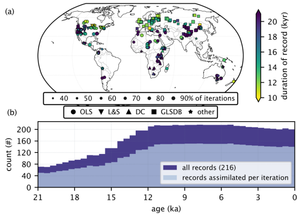
Figure 1: Lake status proxy records. (a) Map showing the spatial distribution of proxy records. Colors indicate the duration of each record, and the size is proportional to the number of iterations each record is used in the assimilation. Shape represents the source of the data including OLS for the Oxford Lake Status databank, GLS for the Global Lake Status databank, L&S for Liefert and Shuman (2020), and DC for De Cort et al. (2021). Other indicates records from smaller data compilations or individual publications. A reference list for each site is provided in Table S1. (b) Data density plot showing the total number of available proxy records at each time step (dark blue) and the mean number of records used by each iteration of the assimilation (light blue). The difference between these represents the number of proxies records withheld for validation.
