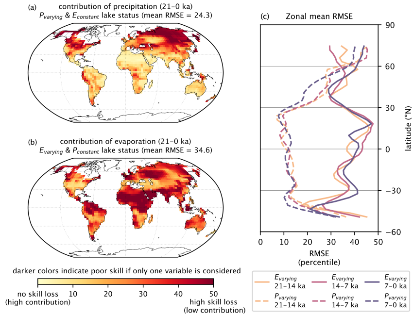
540 Figure 8. Lake status PSM sensitivity tests. Lake status values used in the assimilation were compared to similar values calculated using constant runoff and potential evaporation (a) or constant runoff and precipitation (b). Low RMSE values indicate areas where lake status can be accurately predicted using only the single variable. Panels a and b show values calculated for the entire timeseries. Panel c shows zonal mean RMSE values for sensitivity tests performed for three time periods.
