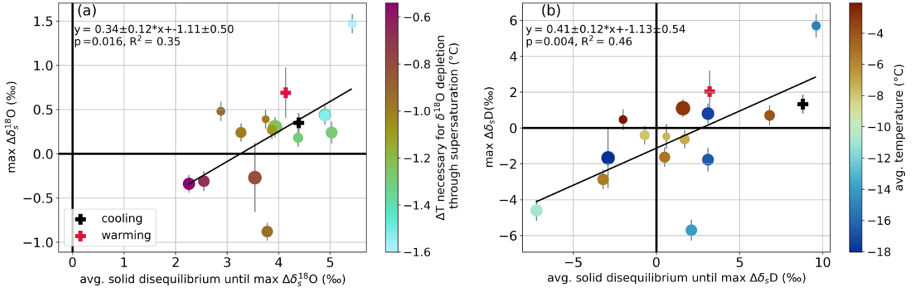
Fig. 6: Changes in snow isotope signal explained The y-axes show the maximum isotopic change observed between airborne snow sample and initial snow sample for \delta^{18}\text{O} in (a) and for \delta D in (b) (same as Fig. 3 (d) and (e)). The x-axes show the average solid disequilibrium in the period after the snow had been added until the maximum change in snow isotopic composition was observed. The colour code in (b) shows the average temperature of the experiments. In (a) the colour code shows the minimum particle-air temperature difference required to produce supersaturation conditions that lead to a negative \delta^{18}\text{O} change in the snow. Linear least-square fits to the data and the corresponding fitting statistics are given.
