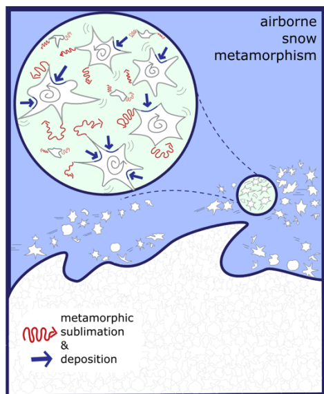
Fig. 7 Conceptual scheme of airborne snow metamorphism The scheme visualises that micro-scale processes of metamorphic sublimation and metamorphic deposition are happening continuously and simultaneously even under net sublimation conditions. We hypothesize that metamorphic vapour deposition on the largest airborne particles due to temperature differences between surrounding air and particle surface together with preferential sublimation of convex sub-grain boundaries and preferential deposition in concavities cause a decrease in SSA and particle growth.
