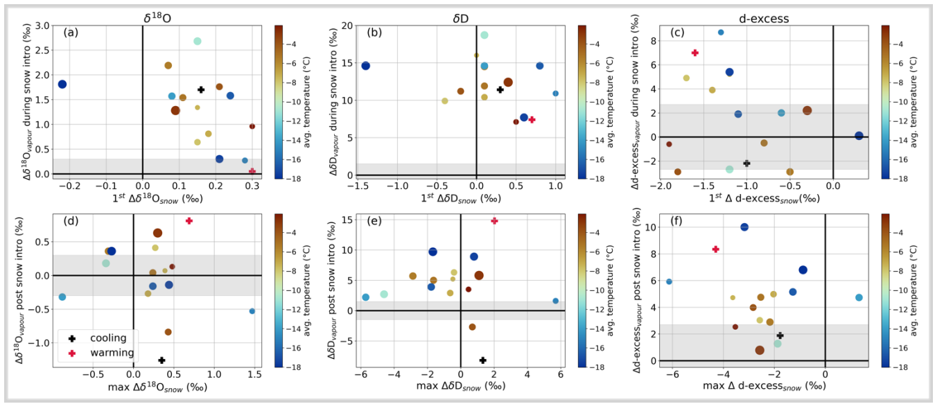
Figure 5 The co-evolution of changes in vapour and snow isotopes in all experiments with vapour isotope observations The change in the snow isotopes (x-axes) is plotted against the changes in the vapour isotopes (y-axes). The changes in vapour isotopes are calculated from the 3-min averaged data. The upper row (a, b, c) shows changes in vapour isotopes during the snow introduction plotted against the observed change in snow isotopes of the first airborne sample (see Fig. 3). The lower row (d, e, f) shows the subsequent change in vapour isotopes post snow introduction until the end of the experiment plotted against the maximum observed change in the snow isotopic composition. Shaded areas represent low variability in vapour isotopic composition ( |\Delta\delta^{18}\text{O}| < 0.3 \text{ ‰} , |\Delta\delta\text{D}| < 1.5 \text{ ‰} , |\Delta\text{d-excess}| < 2.7 \text{ ‰} ). Note that the colour code represents the average air temperature during the experiments and allows the comparison between upper and lower row and the results shown in Fig. 3. The cooling (black cross) and warming (red cross) experiments are exempt.
