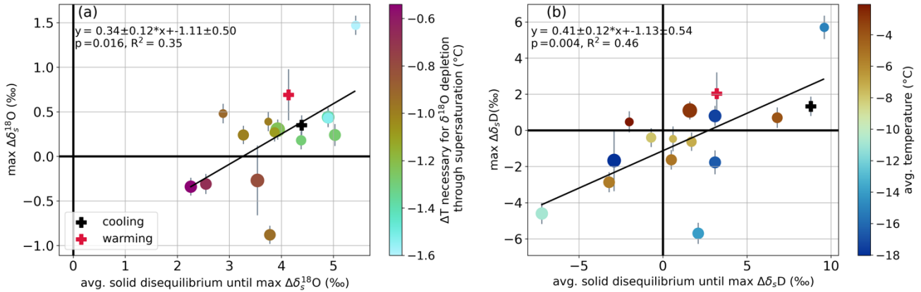
620 Fig. 65: Changes in snow isotope signal explained The y-axes show the maximum isotopic change observed between airborne snow sample and initial snow sample for \delta^{18}\text{O} in (a) and for \delta\text{D} in (b) (same as Fig. 3 (d) and (e)). The x-axes show the average solid disequilibrium in the period after the snow had been added until the maximum change in snow isotopic composition was observed. The colour code in (b) shows the average temperature of the experiments. In (a) the colour code shows the minimum particle-air temperature 625 difference required to produce supersaturation conditions that lead to a negative \delta^{18}\text{O} change in the snow. Linear least-square fits to the data and the corresponding fitting statistics are given.
