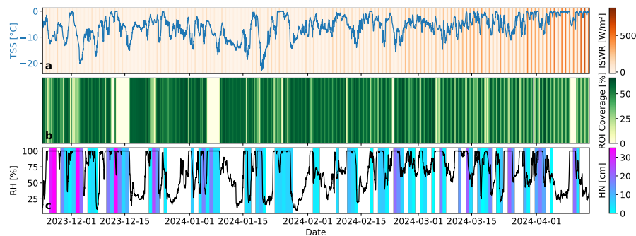
Figure 8. a) Incoming short wave radiation (ISWR, color) and snow surface temperature (TSS, line), b) spatial coverage of the ROI, and c) new snow height (HN, color, white indicates no new snow) and relative humidity (RH, line).
