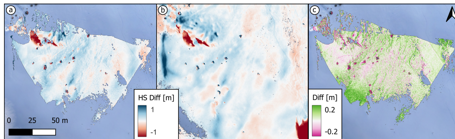
Figure 10. Comparison of the snow depth (HS) differences between 19 December 2023 and 6 February 2024, from a) the lidar point clouds and b) photogrammetric UAV acquisitions. The discrepancies between a) and b) are shown in c). The background image is derived from UAV data from 19 December 2023.
