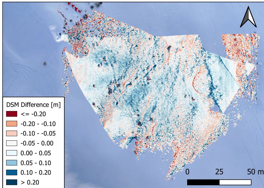
Figure 9. Difference of the DSMs from a UAV photogrammetric acquisition and the lidar point clouds on 19 December 2023, 11:00 UTC. The background image is derived from the UAV data. Ski and snowboard tracks are visible outside of as well as cutting through the monitored area.
