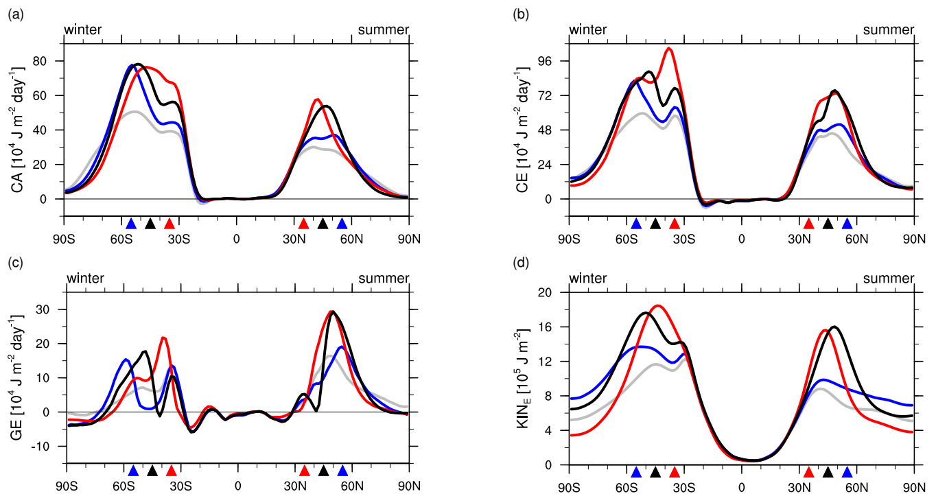
Figure 6. (a) CA, (b) CE, (c) GE, and (d) KIN_E averaged zonally and vertically from 850hPa to 200hPa for F35 (red), F45 (black), F55 (blue), REF (gray), respectively.
