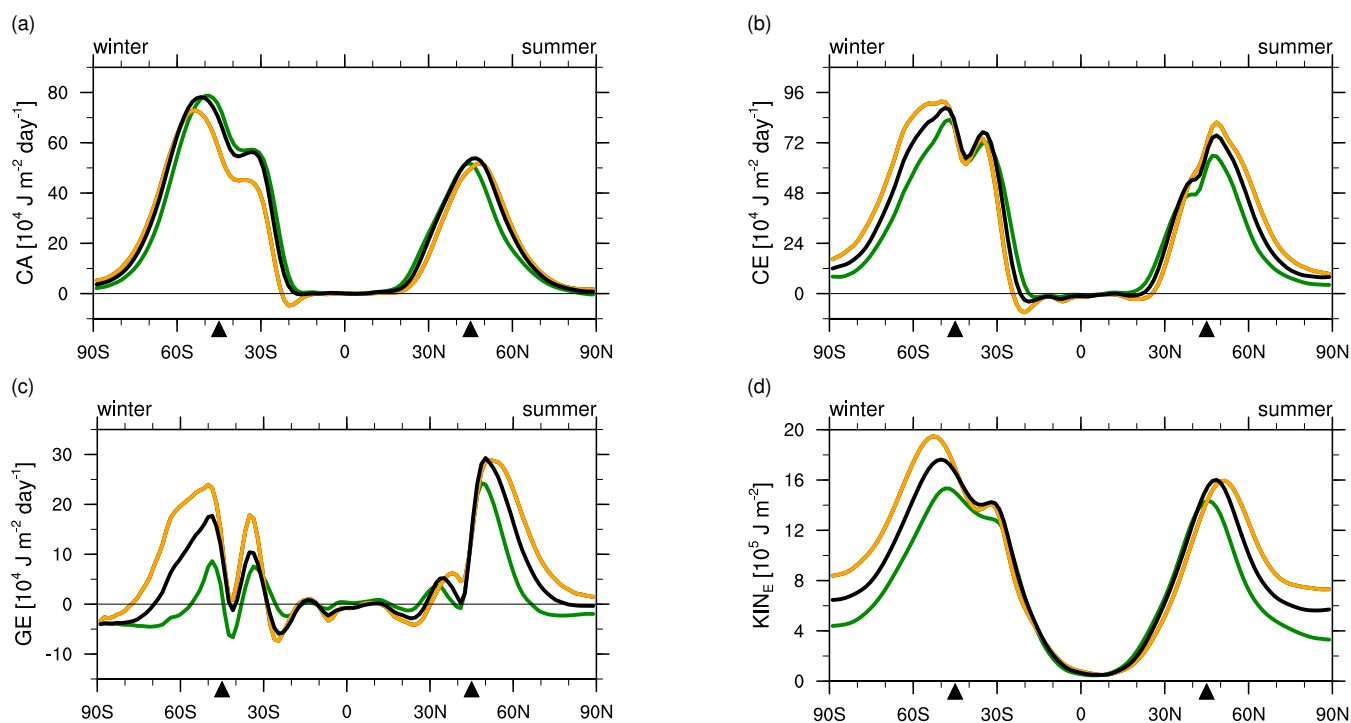
Figure 8. as fig. 6, but for F+45 (orange), F45 (black) and F-45 (green).
