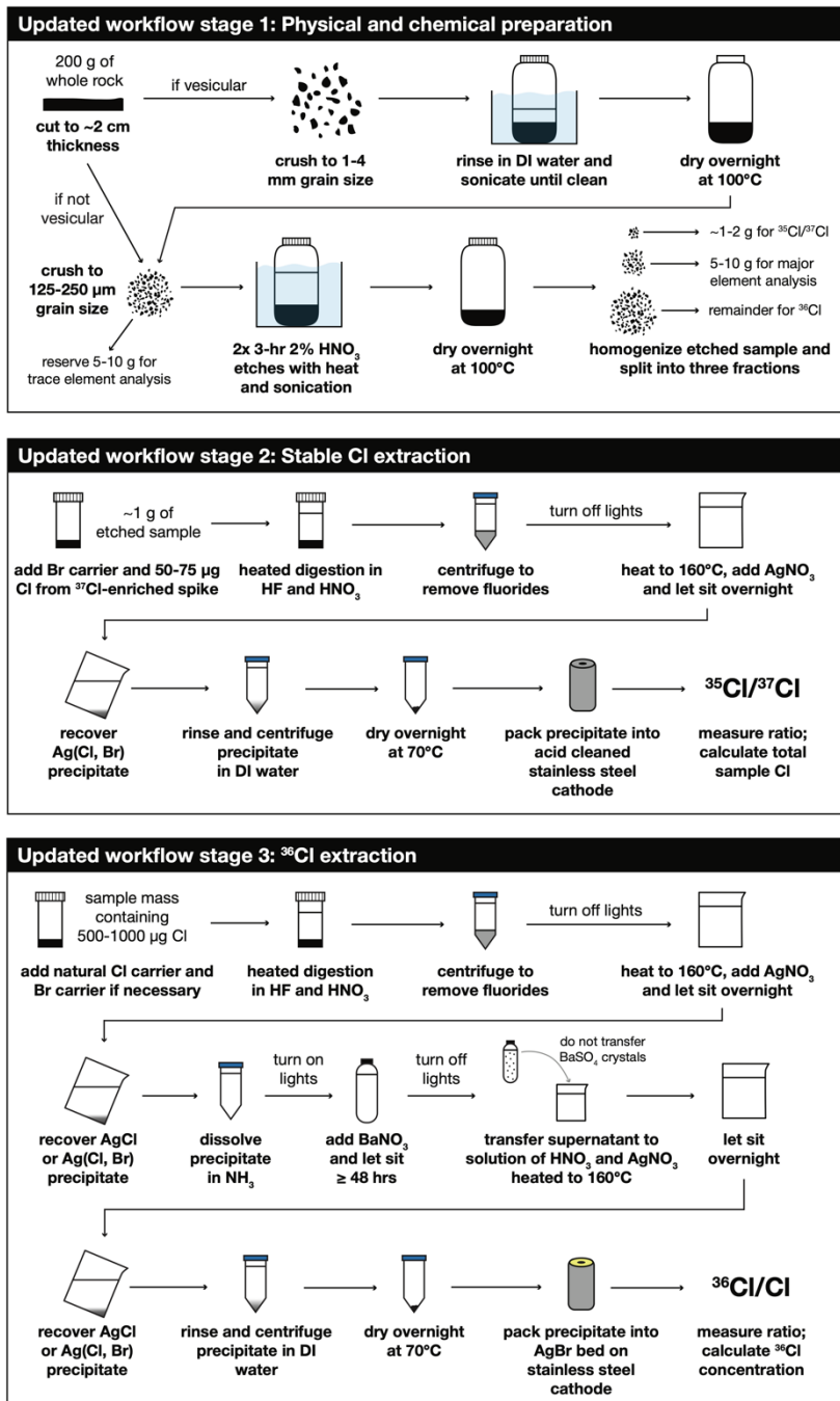
190 Figure 2: Schematic of the updated workflow for cosmogenic 36 Cl analysis presented here. Black arrows indicate the order of steps for each stage of the process. Note that while we use a 37 Cl-enriched spike solution for the stable Cl extraction, these procedures are also suitable for use with a 35 Cl-enriched spike.
