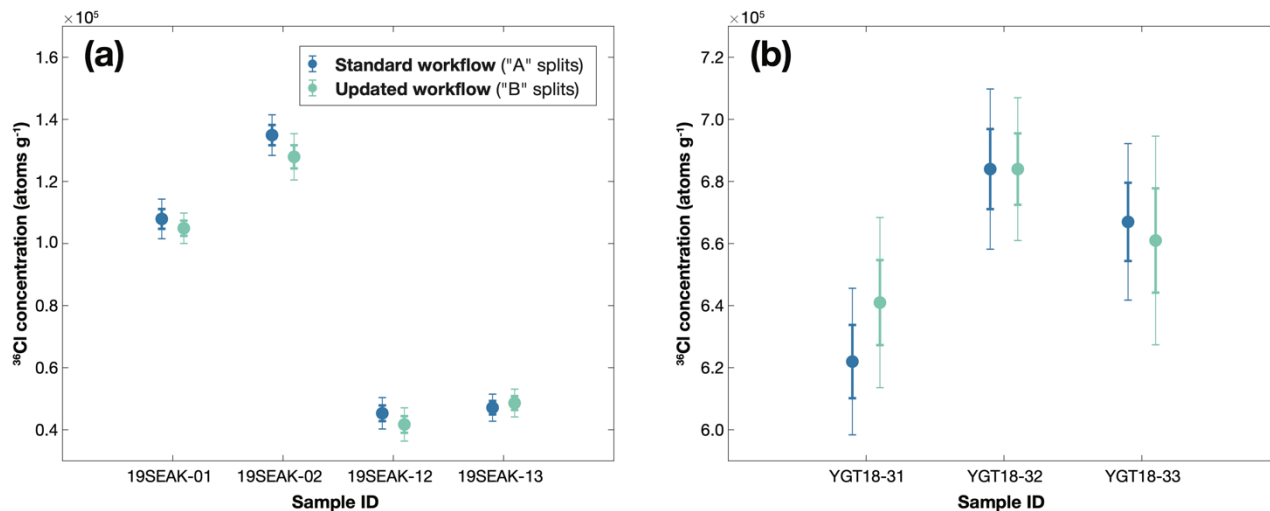
320 Figure 5: Comparison of blank-corrected ^{36}\text{Cl} concentrations (atoms \text{g}^{-1} ) for the geologic test samples (a: Alaskan basalt; b: Yellowstone rhyolite) prepared using the standard workflow (“A” splits; blue dots) and the updated workflow presented here (“B” splits; green dots). Measurement uncertainties for each sample are shown at 1-sigma (thick vertical lines) and 2-sigma (thin vertical lines). Although measurement uncertainties on ^{36}\text{Cl} concentrations for the three YGT18 samples appear visually larger than those of the 19SEAK samples, percent uncertainties on both sets of samples are comparable (Table 4). For ease of comparison, the range of the y-axis in both panels is 1.4 \times 10^5 atoms \text{g}^{-1} .
