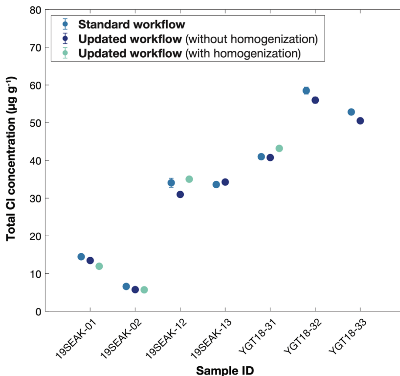
305 Figure 4: Comparison of total Cl concentrations ( \mu\text{g g}^{-1} ) for samples measured using the standard workflow “A” splits (blue dots; all samples), the updated workflow “B-1” splits with aliquots separated without homogenization (purple dots; all samples), and the updated workflow “B-2” splits with aliquots separated after homogenization with a riffle splitter (green dots; four samples only). With the exception of 19SEAK-12A and YGT18-32A, total uncertainties for each sample (Table 3) are smaller than the symbol size. For 19SEAK12-A and YGT18-32A, 2-sigma uncertainty is shown as a vertical line.
