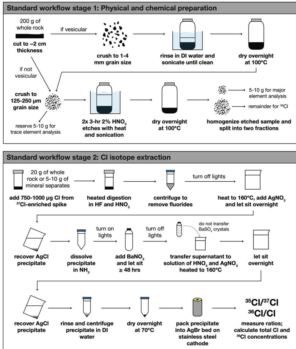
70 Figure 1: Schematic of the standard workflow for cosmogenic ^{36}\text{Cl} analysis based on Licciardi et al. (2008). Black arrows indicate the order of steps for each stage of the process. Note that while we use a ^{37}\text{Cl} -enriched spike solution for the stable Cl extraction, these procedures are also suitable for use with a ^{35}\text{Cl} -enriched spike.
