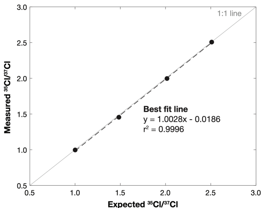
285 Figure 3: Measured vs. expected 35 Cl/ 37 Cl for dilutions of the UNH Wildcat spike and the Weeks Island Halite carrier. Error bars on measured 35 Cl/ 37 Cl are too small to be visible on the figure. Solid gray diagonal line shows a 1:1 relationship between expected and measured 35 Cl/ 37 Cl and dotted black line shows the best fit line between the data points. The equation and r 2 value for the best fit line are also provided.
