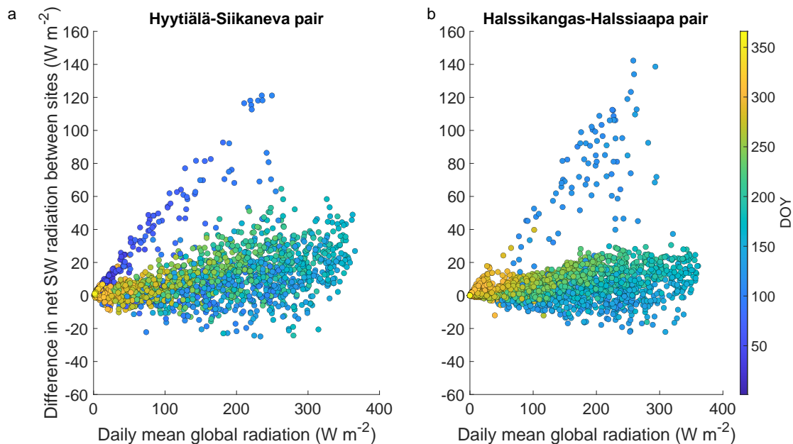
Figure A12. The difference in the net SW radiation between (a) Hyytiälä and Siikaneva and (b) Halssikangas site and Halssiaapa as a function of the mean global radiation over the sites. Daily averages, colour of the markers by DOY. Only days with snow depth at the peatland site of less than 30 cm are included.
