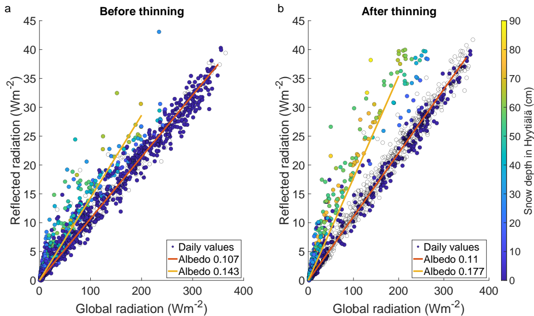
Figure 7. The reflected shortwave radiation in Hyytiälä as a function of global shortwave radiation, coloured by the snow depth. a) Time up to end of January 2020, before the thinning, b) after the thinning, starting from April 2020. Open circles have no snow depth value available, and are typically snow-free points. The albedo values are from a linear model in which the p-values of all predictors are below 1 \times 10^{-6} . Albedo values are presented in Fig. A7.
