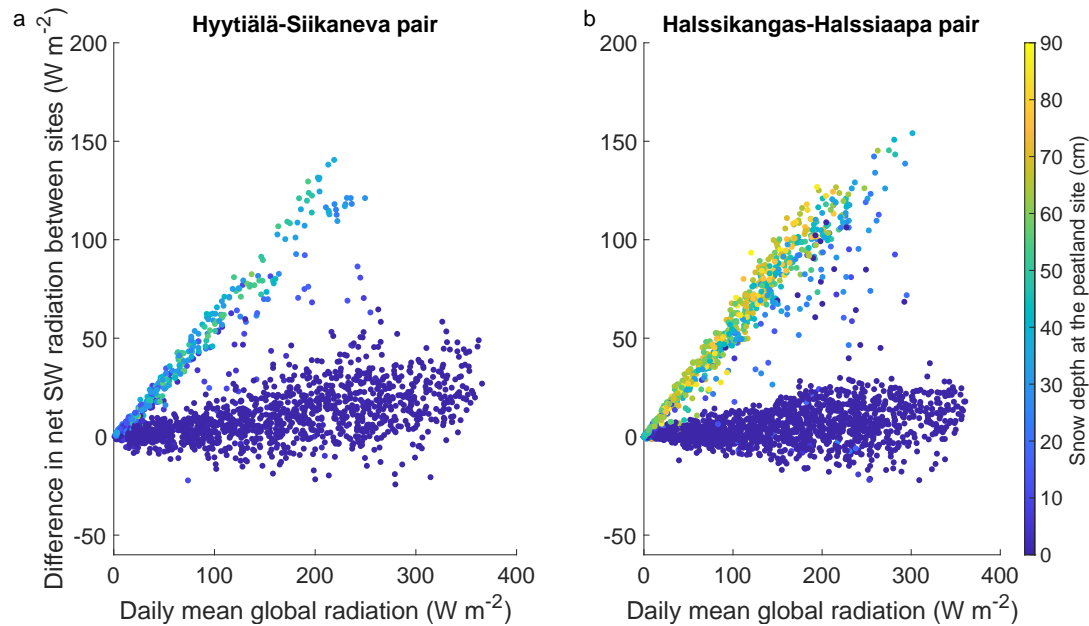
Figure 8. The difference in the net SW radiation between (a) Hyytiälä and Siikaneva and (b) Halssikangas site and Halssiaapa as a function of the mean global radiation over the sites. Daily averages, colour of the markers by the snow depth at the peatland site.
