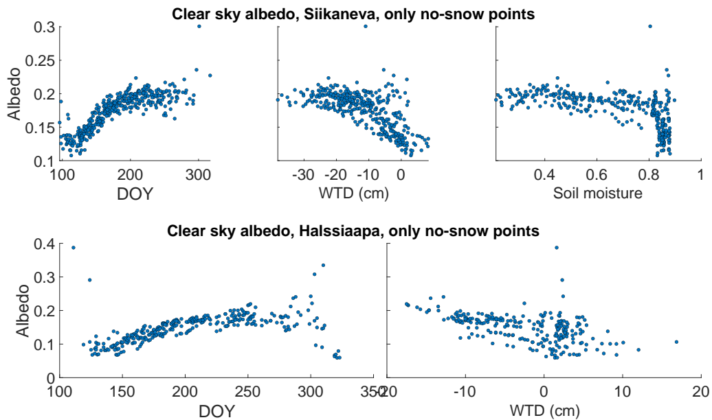
Figure A16. The dependence of peatland summertime albedo on DOY, water table depth, and soil moisture.
