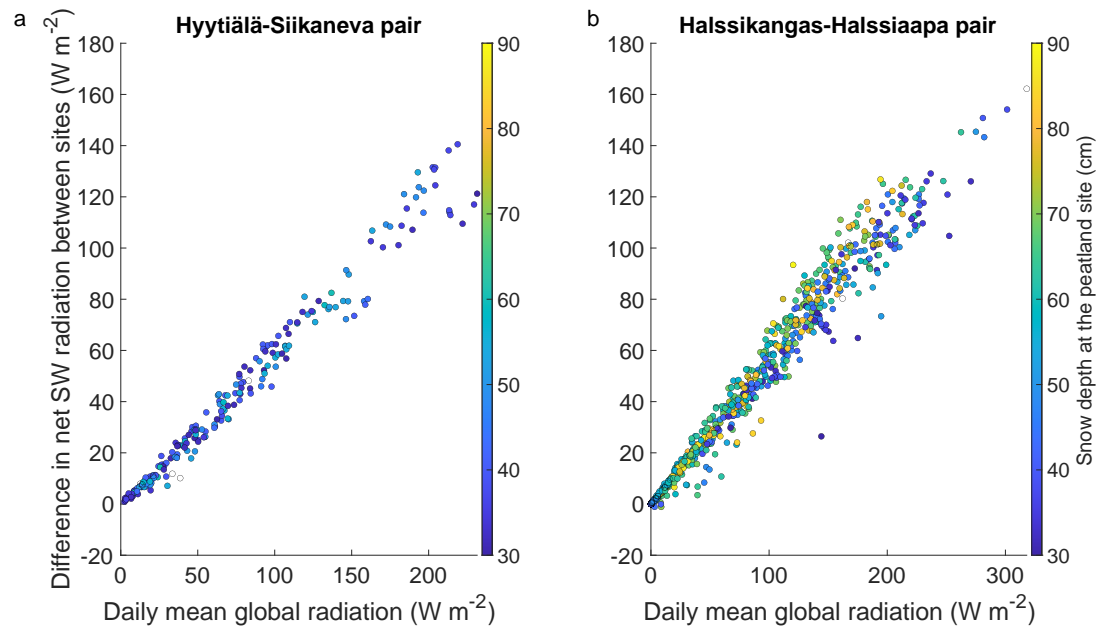
Figure A11. The difference in the net SW radiation between (a) Hyytiälä and Siikaneva and (b) Halssikangas site and Halssiaapa as a function of the mean global radiation over the sites, when the snow depth at the peatland site is at least 30 cm. Daily averages, colour of the markers by the snow depth at the peatland site.
