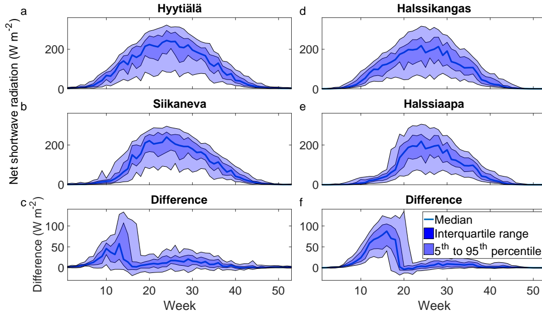
Figure A9. Typical annual cycles of the net SW radiation in the a) Hyytiälä, b) Siikaneva, c) difference of Hyytiälä and Siikaneva, d) Halssikangas, e) Halssiaapa and f) difference of Halssikangas and Halssiaapa. The statistics are calculated for all of the daily values belonging to each week number, over all of the years. The data are not gap-filled, and therefore the data coverage for each panel differs. The Hyytiälä-Siikaneva data set includes eight years, the Halssikangas-Halssiaapa data set includes 12 years. The average annual absorbed shortwave radiation, calculated as a sum of daily medians, is 3.15 \text{ GJ m}^{-2} for Hyytiälä, 2.68 \text{ GJ m}^{-2} for Siikaneva, 2.53 \text{ GJ m}^{-2} for Halssikangas and 2.03 \text{ GJ m}^{-2} for Halssiaapa. The average annual difference between Hyytiälä and Siikaneva, calculated in the same way, is 0.35 \text{ GJ m}^{-2} , and between Halssikangas and Halssiaapa 0.45 \text{ GJ m}^{-2} . Due to the differing data coverages, these numbers are not directly comparable.
