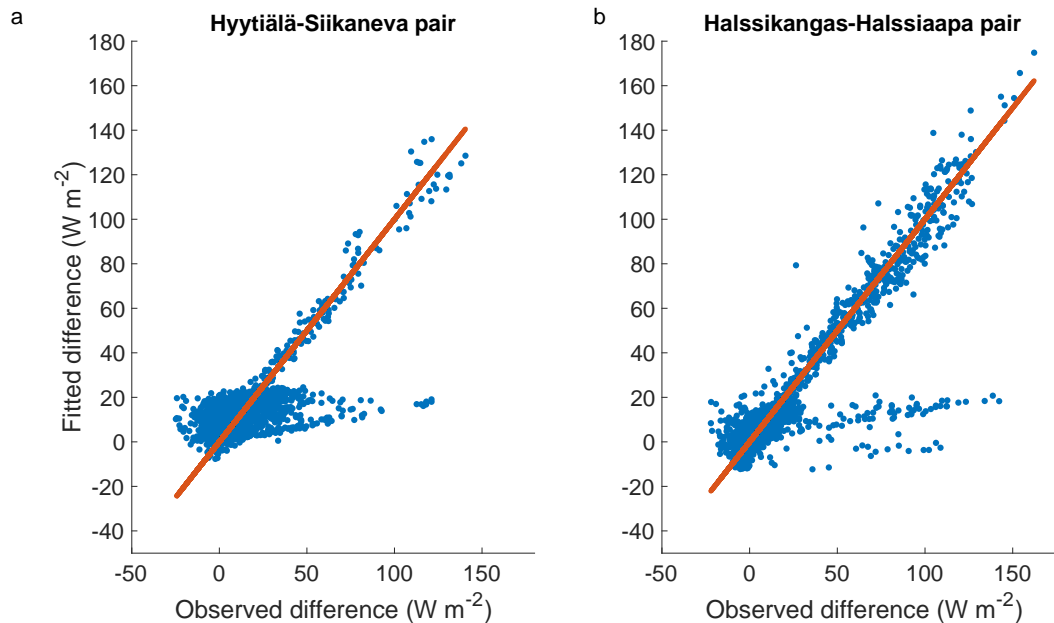
Figure A13. The predicted vs. observed net SW difference values difference in (a) Hyytiälä and Siikaneva and (b) Halssikangas site and Halssiaapa. Predicted points based on linear model with global radiation, snow cover and DOY as predictors, 1:1 line drawn as a reference
