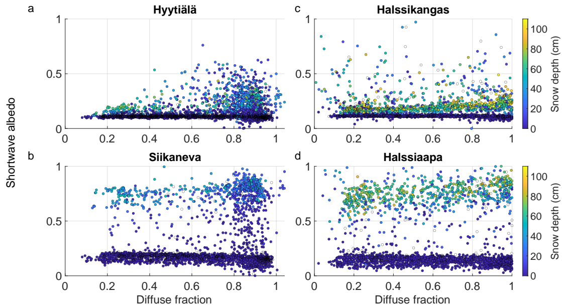
Figure 5. The dependence of albedo on the diffuse fraction of incoming radiation. The points are coloured by the snow depth. For the southern pair, the ratio is of diffuse and total photosynthetically active radiation (PAR) in Hyytiälä, and for the northern pair, of diffuse shortwave radiation at the Sodankylä Tähtelä observatory to global shortwave radiation at the forest site.
