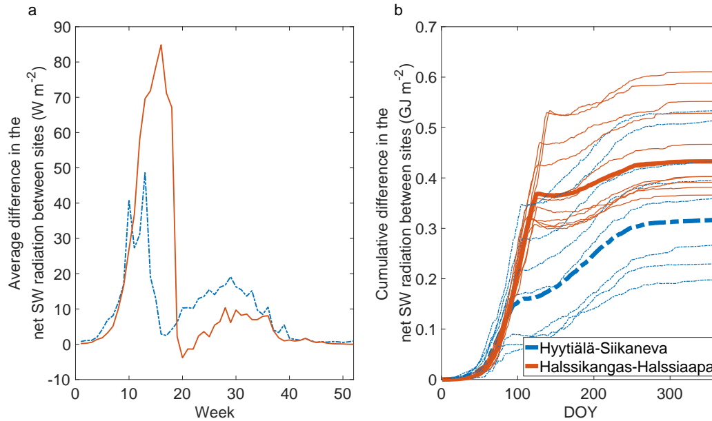
Figure 9. (a) The typical annual cycle in the net SW radiation differences between Hyytiälä and Siikaneva in dashed blue, and Halssikangas and Halssiaapa in red. Positive values mean that the forest absorbs more shortwave radiation than the peatland. For each week, the average net SW difference was calculated as the median of all daily values belonging to that week over the years. Interannual variation shown in Fig. A9. (b) same as a, but cumulative from the start of the year, and calculated for each day of year. Thin lines are individual years. The bold lines are cumulative values calculated of the median years. Note that the median annual difference presented in this way differs from the median calculated from the cumulative individual years. All data shown are gapfilled.
