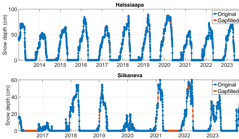
Figure A1. Measured and gapfilled daily snow depth averages from Siikaneva and Halssiaapa.
