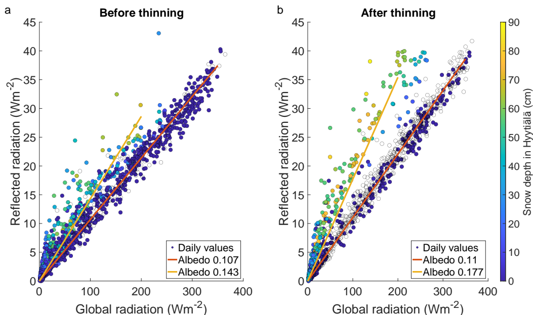
Figure 7. The reflected shortwave radiation in Hyttiälä as a function of global shortwave radiation, coloured by the snow depth. Unfilled markers have snow depth data missing. a) Time up to end of January 2020, before the thinning, b) after the thinning, starting from April 2020. Open circles have no snow depth value available, and are typically snow-free points. The albedo values are from a linear model in which the p-values of all predictors are below 1 \times 10^{-6} . Albedo values are presented in Figs Fig. A7 and ??.
