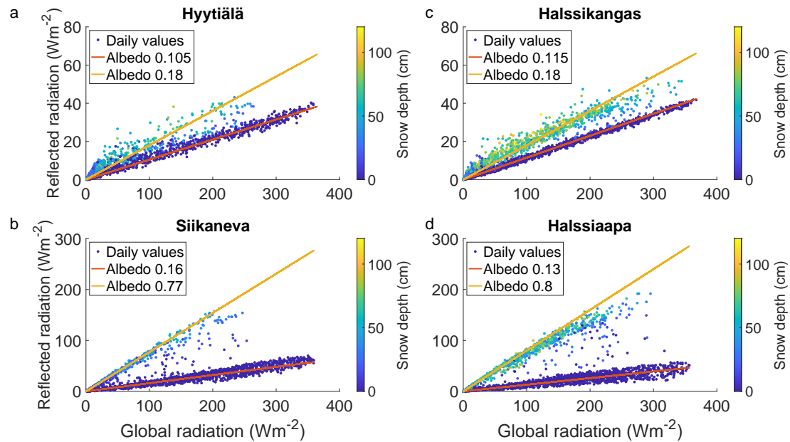
Figure 3. The reflected global radiation as a function of the global radiation for a) Hyytiälä, b) Siikaneva, c) Halssikangas and d) Halssiaapa, 30-minute-daily values. The points are coloured by the snow depth measured at each site: note differing y-axis scales for forest and open peatland sites. Two example lines are drawn in each figure, corresponding to illustrative albedo values that are different for each site. The peatland sites both have a well-defined upper edge of the plot, corresponding to albedos around 0.8, while the forested sites have much less clear edges, and the values are chosen as illustrative examples.
