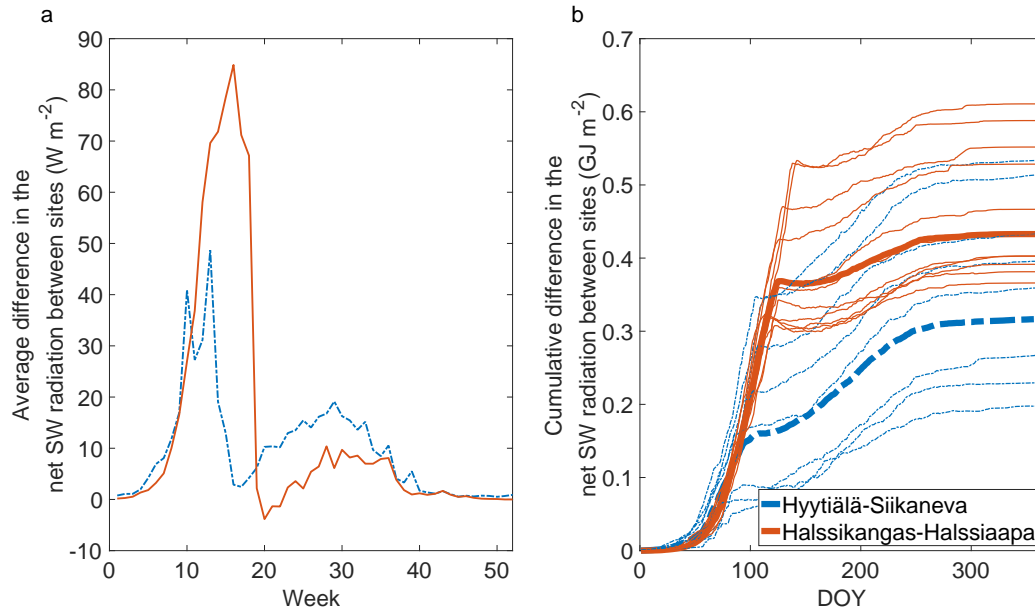
Figure 9. (a) The typical annual cycle in the net SW radiation differences between Hyytiälä and Siikaneva in dashed blue, and Halssikangas and Halssiaapa in red. Positive values mean that the forest absorbs more shortwave radiation than the peatland. For each week, the average net SW difference was calculated as the median of all daily values belonging to that week over the years. Interannual variation shown in Fig. A9. (b) same as a, but cumulative from the start of the year, and calculated for each day of year. Thin lines are individual years. The bold lines are cumulative values calculated of the median years. Note that the median annual difference presented in this way differs from the median calculated from the cumulative individual years. All data shown are gapfilled.
