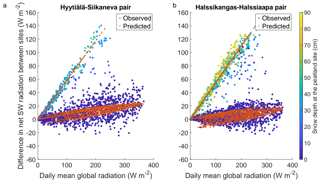
Figure A18. The difference in the net SW radiation between (a) Hyytiälä and Siikaneva and (b) Halssikangas site and Halssiaapa as a function of the mean global radiation between over the sites. Daily averages, colour of the markers by the snow depth in at the peatland site. Fitted points based on linear model with global radiation, snow cover and DOY as predictors.
