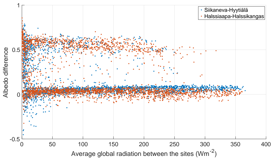
Figure A10. The albedo difference (peatland - forest) as a function of the incoming radiation. The product of these two parameters the global radiation and the difference in albedo determines the difference in the net SW radiation between the sites (Eq. (2)).
