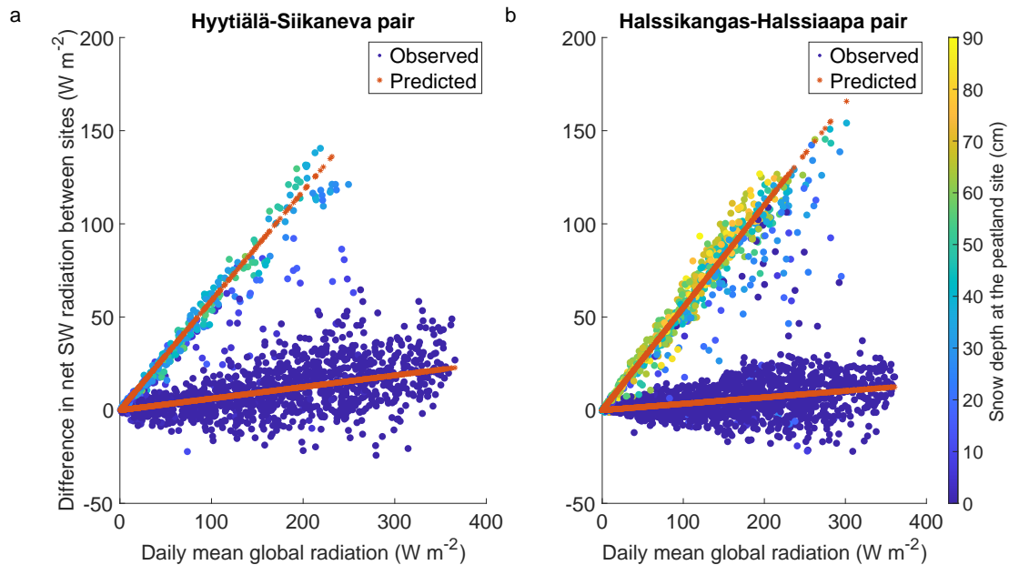
Figure A14. The difference in the net SW radiation between the Halssikangas and Halssiaapa sites as a function of the mean global radiation between over the sites. Daily averages, colour of the markers by the snow depth in Halssiaapa. Fitted points based on linear model with different slopes for snow cover categories less and over 30 cm.
