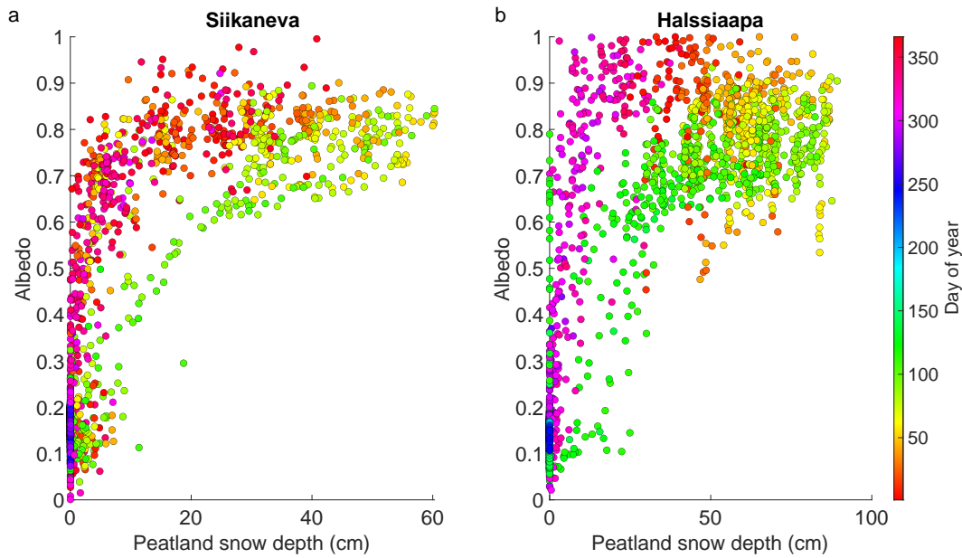
Figure A5. The peatland albedo as a function of forest daily albedo and peatland snow depth in at the peatland sites, (a) the southern Siikaneva and (b) the northern Halssiaapa. The points are coloured by the day of year (DOY). The springtime values in Halssiaapa around DOY 100, with a high albedo but a low snow depth, are associated with the times when the peatland snow depth measurement has reached zero, but snow is still detected at the forest site pair.
