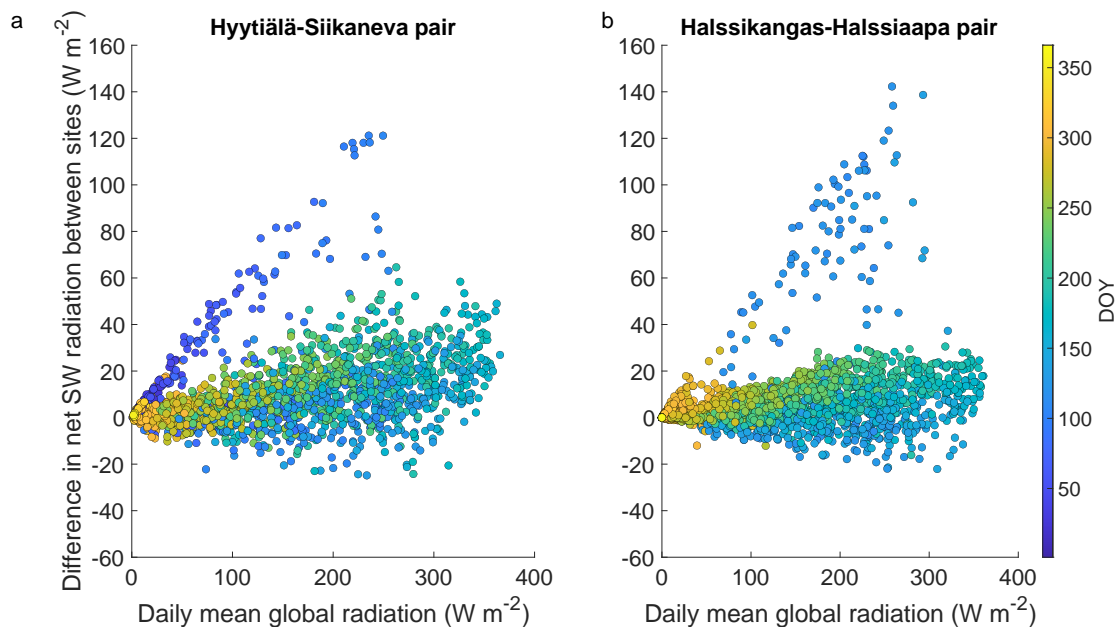
Figure A12. The difference in the net SW radiation between (a) Hyytiälä and Siikaneva and (b) Halssikangas site and Halssiaapa as a function of the mean global radiation between-over the sites. Daily averages, colour of the markers by DOY. Only days with snow depth at the peatland site of less than 30 cm are included.
