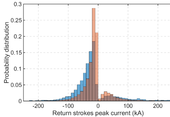
Figure 7: Distribution of AEMET return strokes detected by the WLLN, in blue color, and total AEMET return strokes, in orange color.
