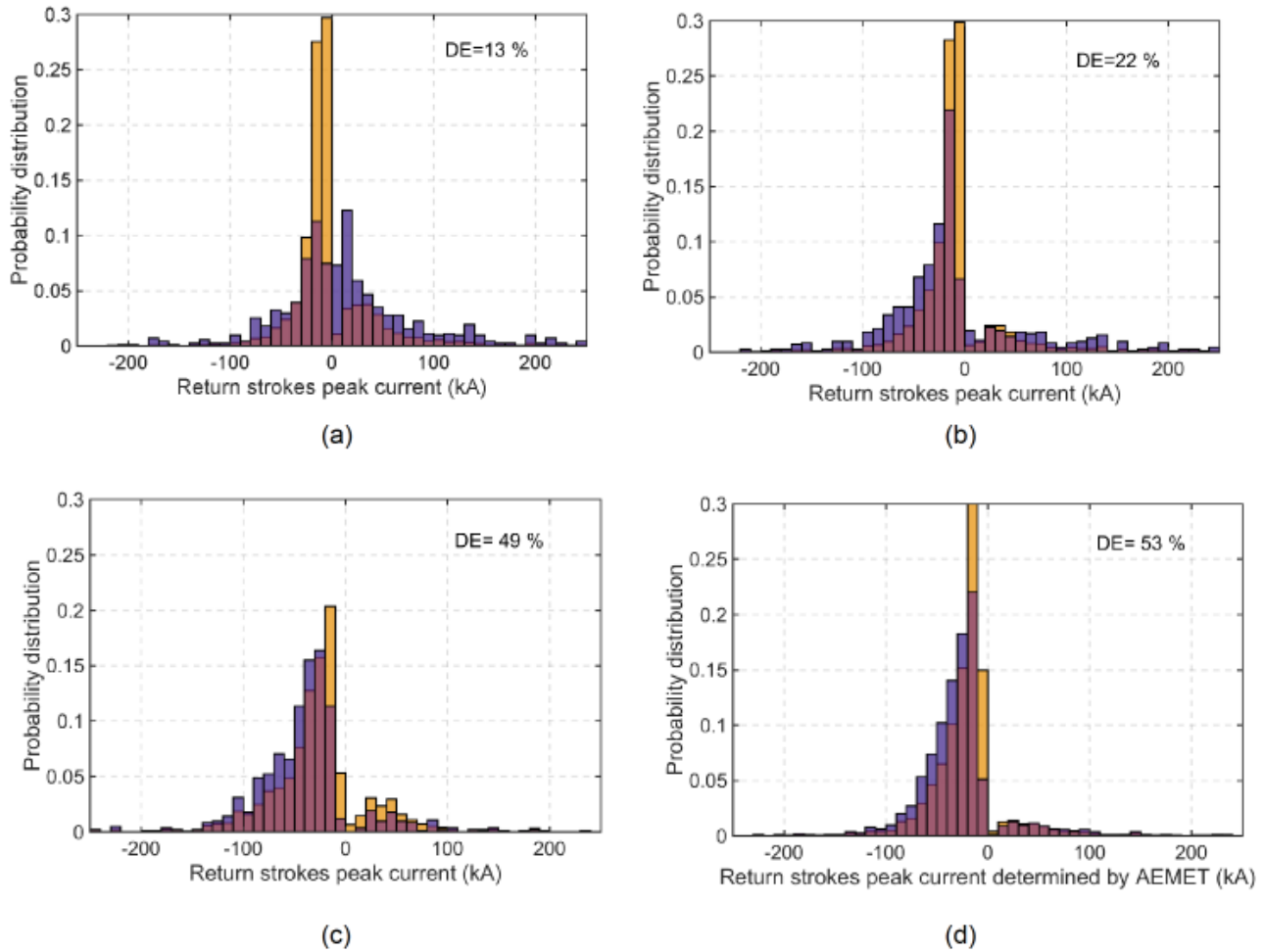
570 Figure 10: Distribution of AEMET return strokes also detected by the WWLLN, in blue color, and total AEMET return strokes, in orange color for different subregions: a) Spanish Plateau, b) East Spanish Mediterranean coast, c) West African Atlantic coast, and d) South Spanish Mediterranean coast.
