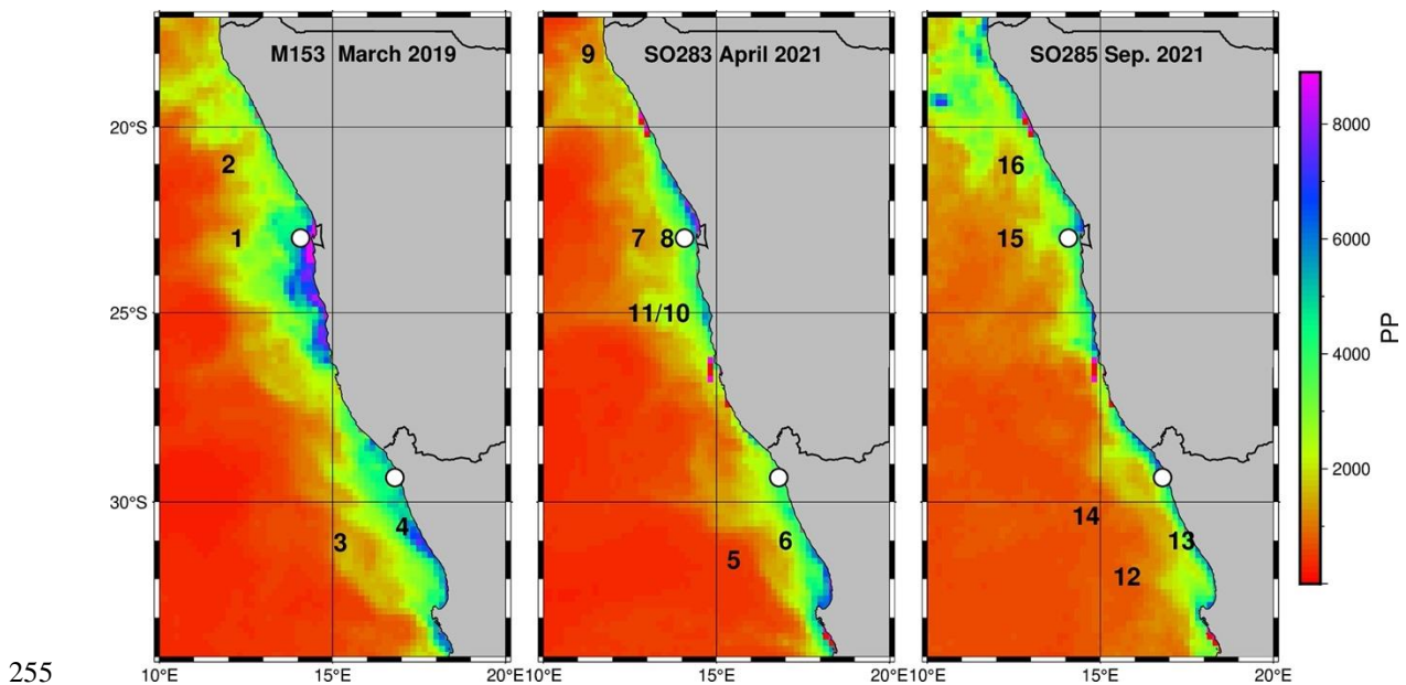
255 Figure 4 Primary production rates (SeaWiFS) in \text{mg C m}^{-2} \text{ day}^{-1} during the research cruises M153, SO283 and SO285 as well as the locations of the drifter deployments (black numbers) and long-term sediment trap mooring sites (white circles).
