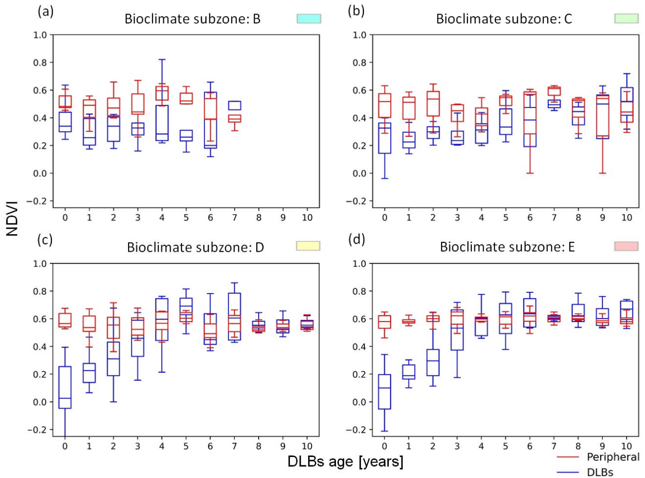
Figure 2. Subplots (a - d) , NDVI change within the first ten years after drainage separated by bioclimatic subzone ( a-B - dE ). The peripheral area refers to the area around the DLBs for a zone of 1 km.
