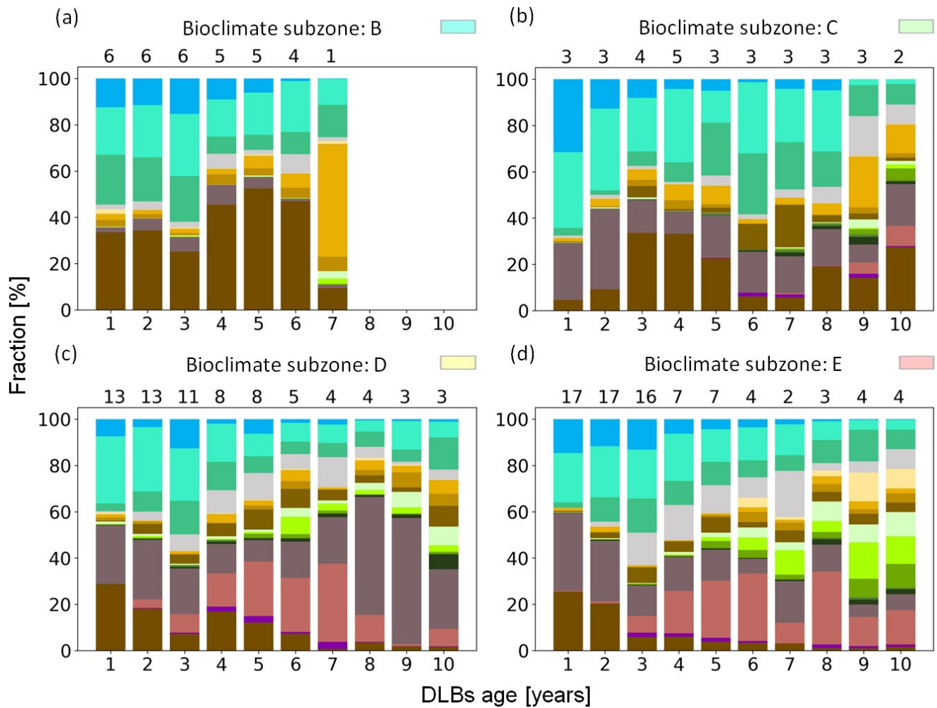
Figure 3. Subplots (a - d) . Landcover change in time for the DLBs separated by the different bioclimate subzones ( a-d ) ( B - E ). The sum of available basins for a certain age is displayed on top. For color legend see Table 1.
