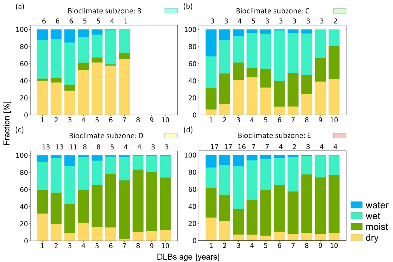
Figure 6. Subplots (a - d). Fraction change of wetness groups (see Table 1) for different DLB ages (1 - 10) separated into the bioclimatic subzones (a-d) (B - E).
