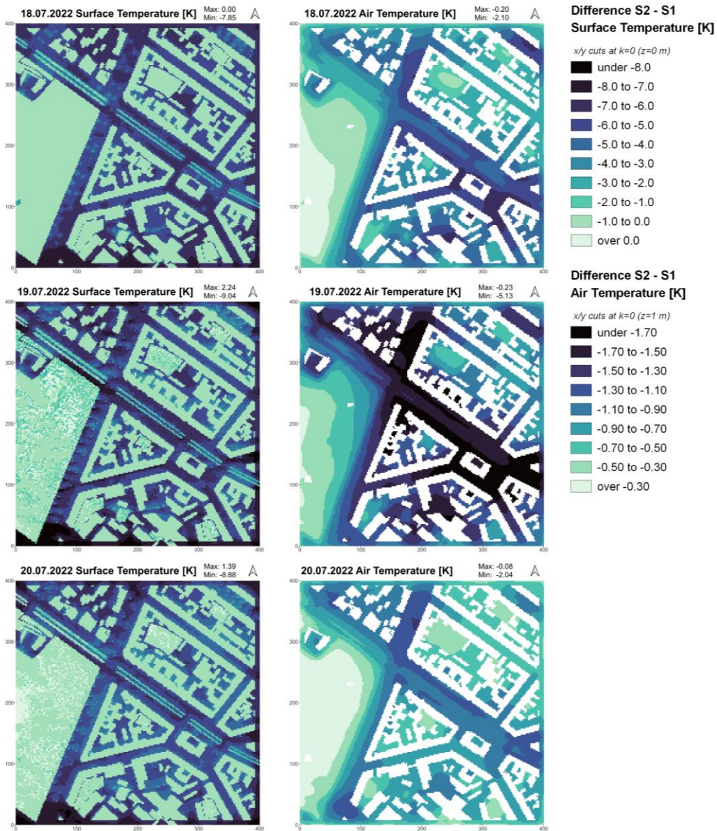
Figure 8: Spatial distribution of the mean differences in surface temperature [K] (left) and air temperature [K] (right) between S1 (reference run) and S2 (extreme scenario) for all three single days of the study period. The color scales correspond to those in Figure 6 and Figure 7. The x- and y-axes indicate the spatial distance in the study area [in m].
