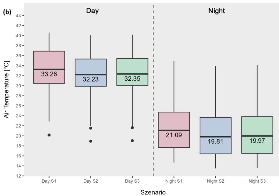
805 Figure 11a (above): Boxplots of the mean air temperature for the three simulations S1, S2 and S3 in 1 m height above ground level (left), 3 m height above ground level (middle), and 5 m height above ground level (right). Averages of all GGP grid cells for the 72 hourly output values. Figure 11b (below): Boxplots of the mean air temperature in 1 m height above ground level for the three simulations S1, S2 and S3 divided into daytime (left) and nighttime (right). Averages of all GGP grid cells for the 72 hourly output values.
