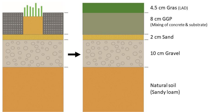
Figure 1: Schematic structure of a GGP on the left, and developed implementation in ENVI-met on the right (own illustration based on HOFFMANN & GEISSLER 2022).
