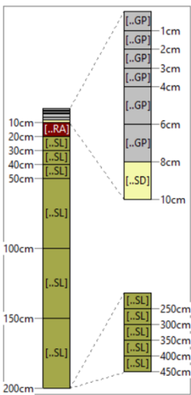
Figure 3: Vertical structure of the GGP soil profile in the Database Manager; SL = Sandy Loam, RA = Gravel, SD = Sand, GP = Grass Grid Pavers (own illustration in ENVI-met DBManager).
