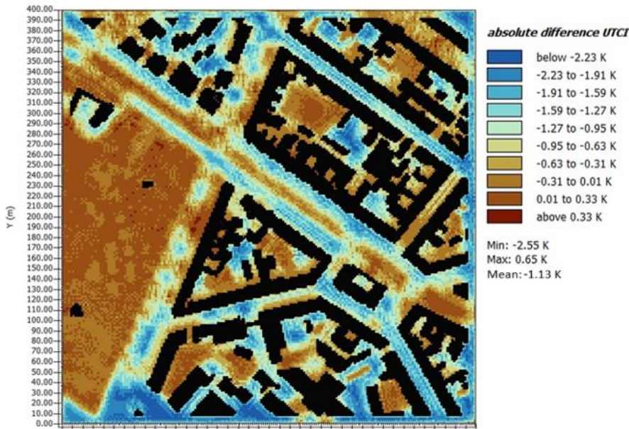
Figure 126: Absolute difference in the biometeorological Universal Thermal Climate Index (UTCI) between the reference run S1 and the extreme scenario S2 in a height of 1.3 m above ground level.
