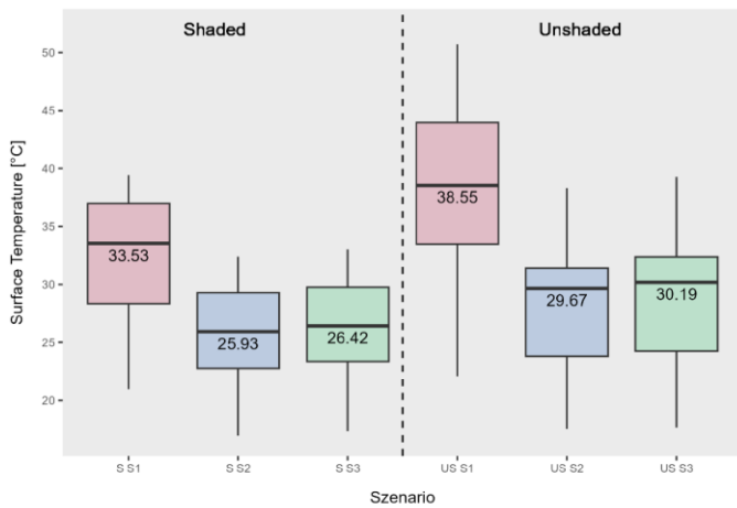
Figure 9a (above): Boxplots of the mean surface temperature for the three simulations S1, S2 and S3. Averages of all GGP grid cells for the 72 hourly output values.
