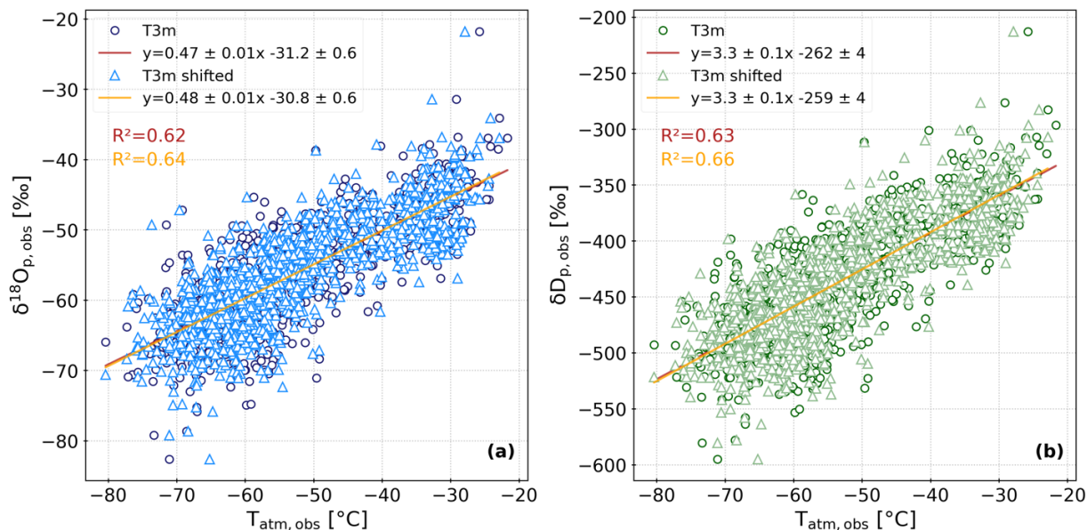
925 Figure A1. Daily observed precipitation \delta^{18}\text{O} (a) and \delta\text{D} (b) versus observed daily mean temperature at Dome C. All precipitation samples collected between 2017 and 2021 are shown against the corresponding daily mean temperature (T3m, dark colours) and the daily mean temperature of the day before (T3m shifted, light colours). The linear regressions with the associated coefficients of determination ( R^2 ) are shown. Both linear slopes are significant ( p -values < 0.001 ).
