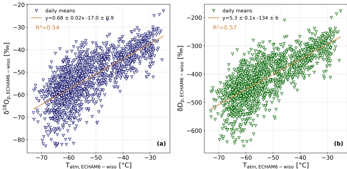
930 Figure A2. Daily precipitation \delta^{18}\text{O} (a) and \delta\text{D} (b) modelled by ECHAM6-wiso versus daily mean temperature modelled by ECHAM6-wiso. The linear regressions with the associated coefficients of determination ( R^2 ) are shown. Both linear slopes are significant ( p -values < 0.001 ).
