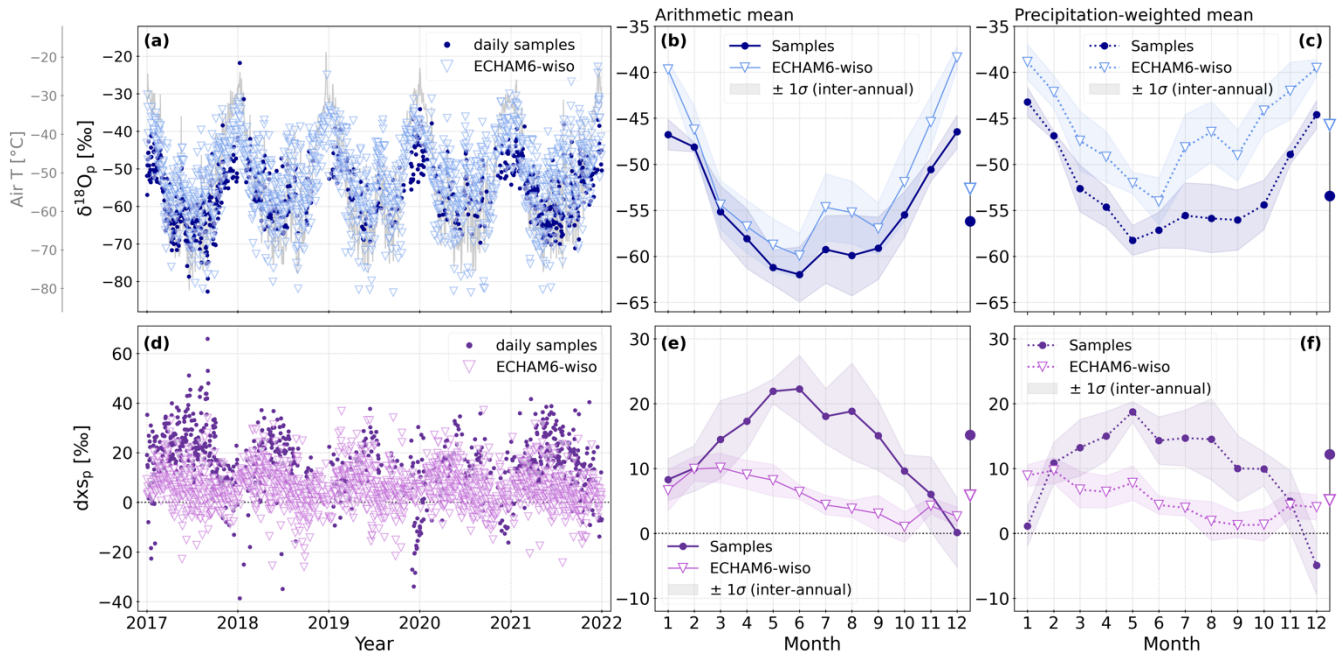
475 Figure 6. Observed and modelled precipitation isotopic composition at Dome C. Panels (a) and (d) show the 5-year time series (2017-2021) for \delta^{18}\text{O} and d-excess (dxs) respectively. The dots represent the daily samples collected in the field (sample description in Sect. 2.3) and the triangles represent the daily precipitation isotopic composition modelled by ECHAM6-wiso (description of simulations in Sect.
