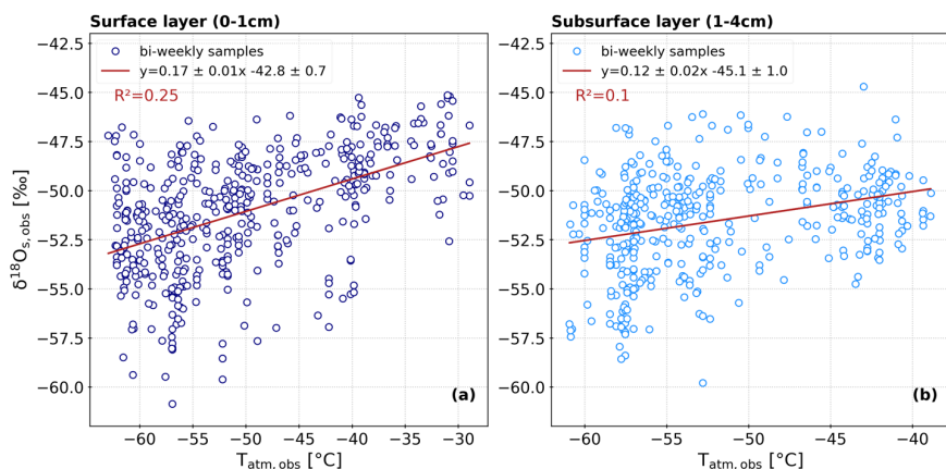
Figure A3. Bi-weekly observed snow surface (a) and subsurface (b) \delta^{18}\text{O} versus temperature at Dome C. All snow samples collected between 2017 and 2021 are shown against the weighted-average temperature (by precipitation amounts) over the period corresponding to the accumulation of the snow samples (see Sect. 4.2.3). The linear regressions with the associated coefficients of determination ( R^2 ) are shown. Both linear slopes are significant ( p -values < 0.001 ).
