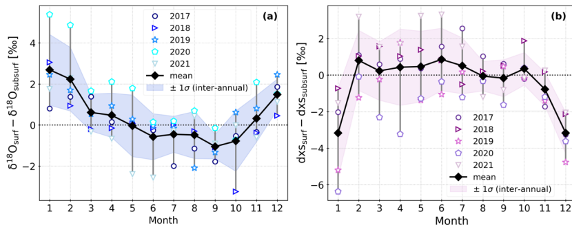
480 Figure 4. Mean annual cycle (monthly means) of the observed vertical difference between the snow surface and subsurface isotopic composition at Dome C. Panel (a) shows the mean annual cycle of the vertical difference in \delta^{18}\text{O} , panel (b) shows the mean annual cycle of the vertical difference in d-excess. In both panels, the black diamonds correspond to the overall monthly means calculated over the 2017-2021 period. The shaded area shows the inter-annual variability of individual years around the overall monthly means (one standard deviation) and the coloured markers show the monthly means for each individual year.
