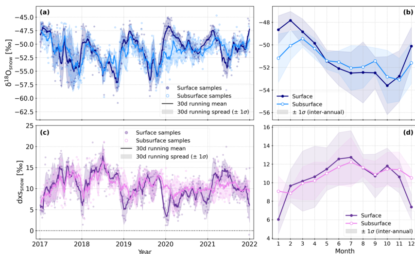
405 Figure 3. Observations of the snow surface and subsurface isotopic compositions at Dome C. Panels (a) and (c) show the 5-year time series (2017-2021) for \delta^{18}\text{O} and d-excess (dxs) respectively. The circles represent the horizontal average between the two samples taken at the two locations 50 m apart on the sampling lines (described in Sect. 2.2) and the solid lines show a 30-day running mean of these horizontal averages. The shaded area represents the 30-day running average of the spatial spread between the two samples taken at the two locations 50 m apart on the sampling lines (one standard deviation). Panels (b) and (d) show the mean annual cycles (monthly means) of
