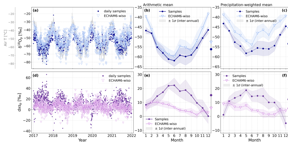
570 Figure 6. Observed and modelled precipitation isotopic composition at Dome C. Panels (a) and (d) show the 5-year time series (2017-2021) for \delta^{18}\text{O} and d-excess (dxs) respectively. The dots represent the daily samples collected in the field (sample description in Sect. 2.3) and the triangles represent the daily precipitation isotopic composition modelled by ECHAM6-wiso (description of simulations in Sect.
