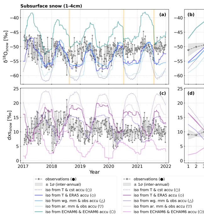
Figure 9. Comparison between observed and simulated snow subsurface (1 to 4 cm depth) isotopic compositions at Dome C. Panels (a) and (c) show the 5-year time series (2017-2021) of \delta^{18}\text{O} and d-excess (dxs) respectively. The grey dots represent the horizontal average between the two samples taken at the two locations 50 m apart on the sampling lines (described in Sect. 2.2, also presented in Fig. 3). The coloured lines (dotted and plain) represent the different SISG model experiments (described in Table 3). Panels (b) and (d) show the mean annual cycles (monthly means) of \delta^{18}\text{O} and d-excess, respectively, calculated over the period 2017-2021. The grey dots and line represent the observations and the shaded area represents the inter-annual variability around the mean annual cycle (one standard deviation). The coloured lines (dotted and plain) represent the different SISG experiments (described in Table 3). The markers on the right vertical axis indicate the mean isotopic composition of the observed and simulated snow subsurface over 5 years (see Table S2 in Supplement S4.2).
