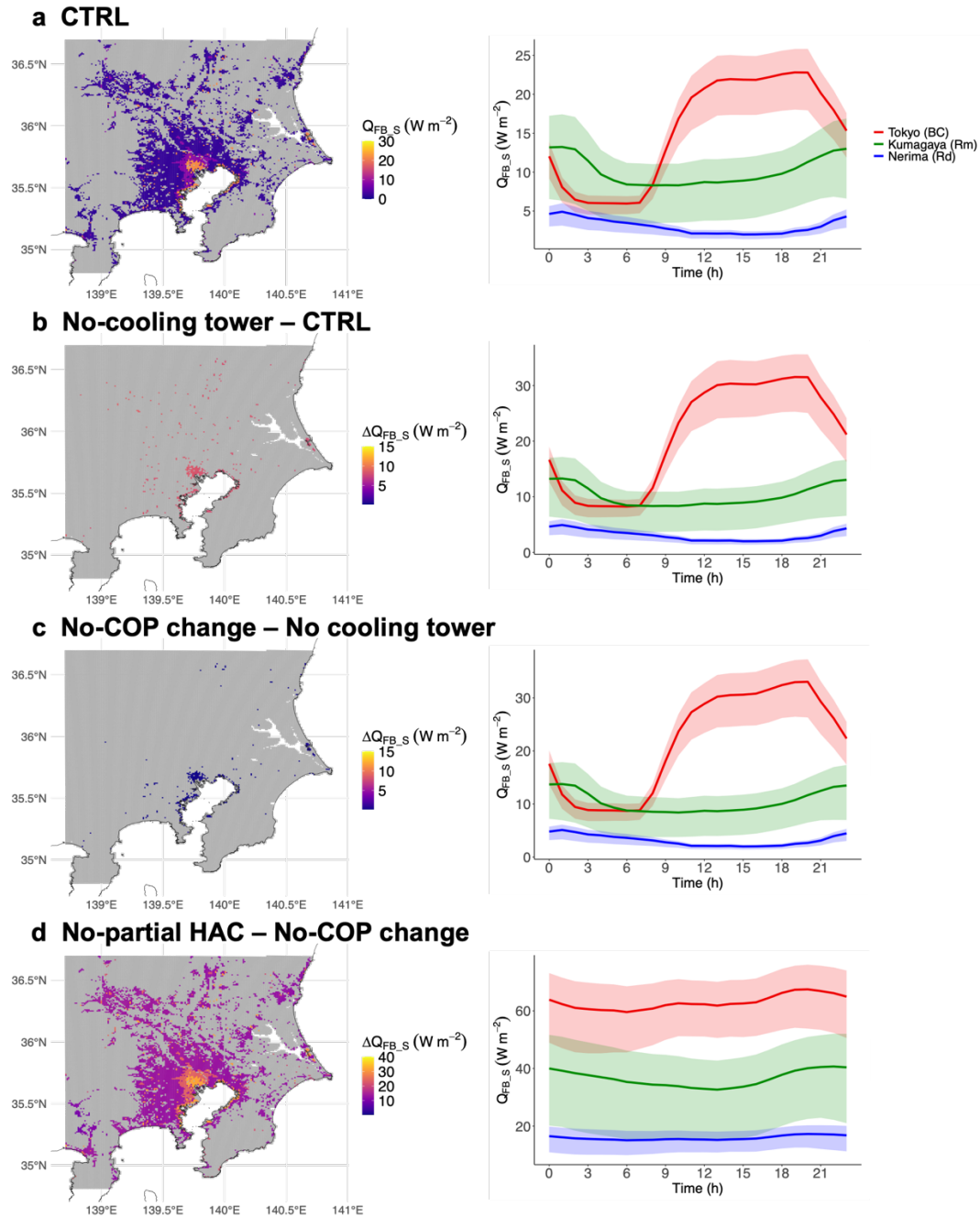
Figure 11: The average, SLUCM+BEM-simulated Q_{FB,S} in distributions over the Tokyo Metropolitan Area averaged forat 14:00 LT in summer obtained from SLUCM+BEM (left). Diurnal changes in the Q_{FB,S} in values for Tokyo (BC), Kumagaya (Rm), and Nerima (Rd) (right). Lines and error bars are the simulated average values and the 5th–95th percentiles, respectively. The simulations were run for (a) control (CTRL), (b) no cooling tower, (c) no coefficient of performance (COP) change, and (d) no partial HAC scenarios.
