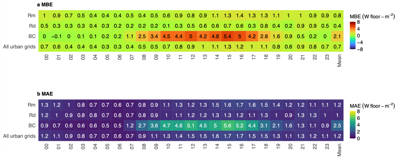
Figure 7: Diurnal changes in (a) MBE and (b) MAE of EC_{HAC} for each urban building use type, Rm, Rd, and BC, and the average of all grids from SLUCM+BEM (upper panels) and CM-BEM (new model; lower panels) averaged over the summer season's weekdays.
