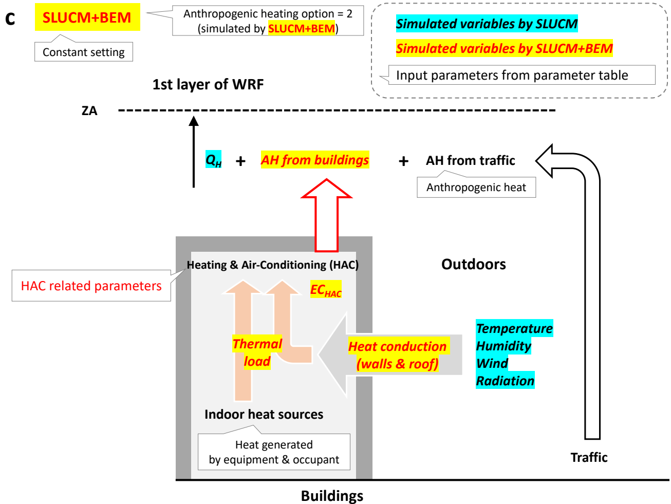
Figure 1: Schematic of energy budgets for an urban canopy layer that includes buildings. The single-layer urban canopy model (SLUCM) with (a) “Zero-Flux” and (b) “Constant” settings. (c): The updated SLUCM based on a building energy model (BEM), thus SLUCM+BEM, with a “Constant” setting. Blue and yellow highlighting indicate variables simulated by SLUCM and SLUCM+BEM respectively. The text in the callouts indicates original or newly introduced inputs to the WRF parameter table URBNPRAM.TBL.
