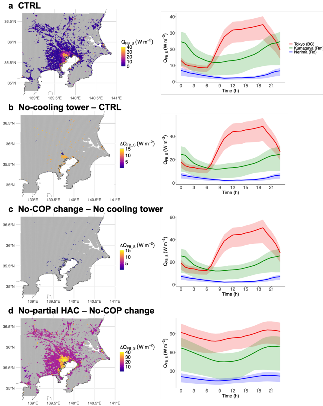
Figure 11: The average, SLUCM+BEM-simulated Q_{FB,S} in distributions over the Tokyo Metropolitan Area averaged forat 14:00 LT in summer obtained from SLUCM+BEM (left). Diurnal changes in the Q_{FB,S} invalues for Tokyo (BC), Kumagaya (Rm), and Nerima (Rd) (right). Lines and error bars are the simulated average values and the 5th–95th percentiles, respectively. Simulation results areThe simulations were run for cases including (a) control (CTRL), (b) no cooling towertower, (c) no coefficient of performance (COP) change, and (d) no partial HAC scenarios.
