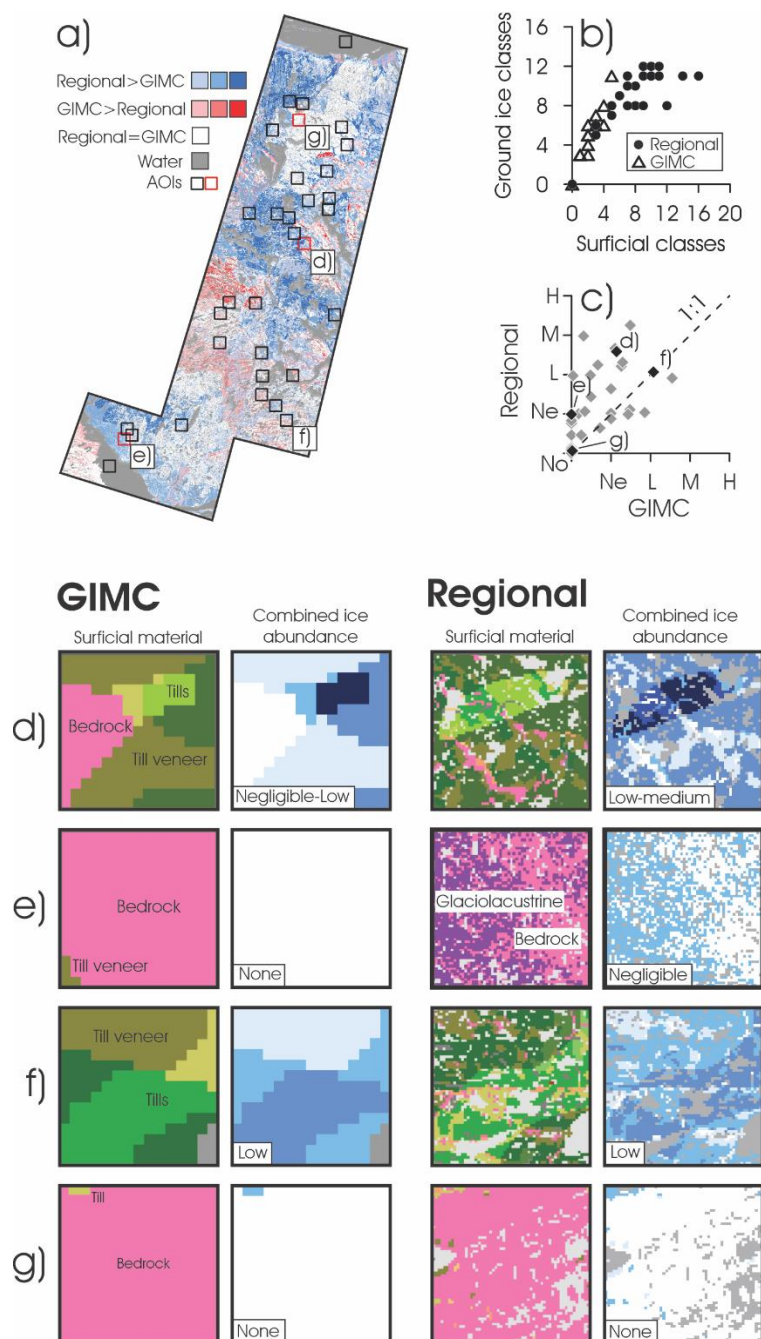
205 Figure 4. Difference map between a) modelled regional and GIMC combined ice abundance; greater differences are indicated by darker shades; squares indicate random (black) and selected (red) 15 x 15 km areas of interest (AOIs) used in the analysis, b) relation between the number of surficial materials classes and number of ground ice classes represented in each AOI shown in a), c) average ground ice content in each AOI for the GIMC vs. regional outputs; No, Ne, L, M, H = none, negligible, low, medium, and high,
