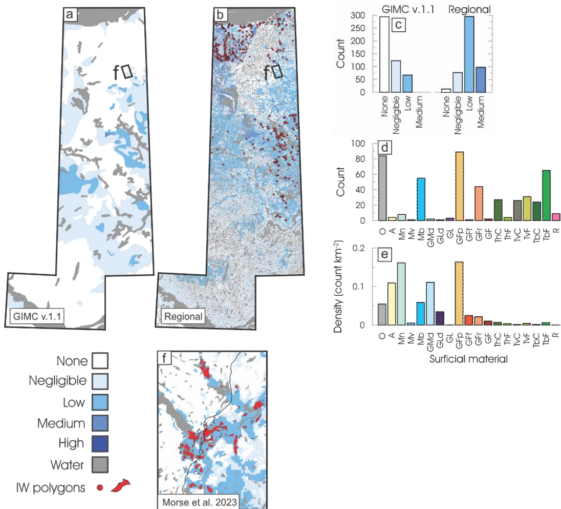
270 Figure 7. Modelled wedge ice abundance from a) GIMC v.1.1, b) the regional modelling, with ice wedge polygons mapped on five Canadian Geoscience Maps overlain (n=484), c) histogram of mapped ice wedge polygon points from b) and corresponding ground ice abundance on the regional and national-scale mapping, respectively, d) histogram of surficial geology from the regional 275 compilation underlying each mapped ice wedge polygon point, e) corresponding density of ice wedge polygon points in each surficial material unit; the area for each unit is based on coverage for the entire modelled domain, and f) ice-wedge polygons mapped along the proposed transportation infrastructure corridor (Morse et al., 2023).
