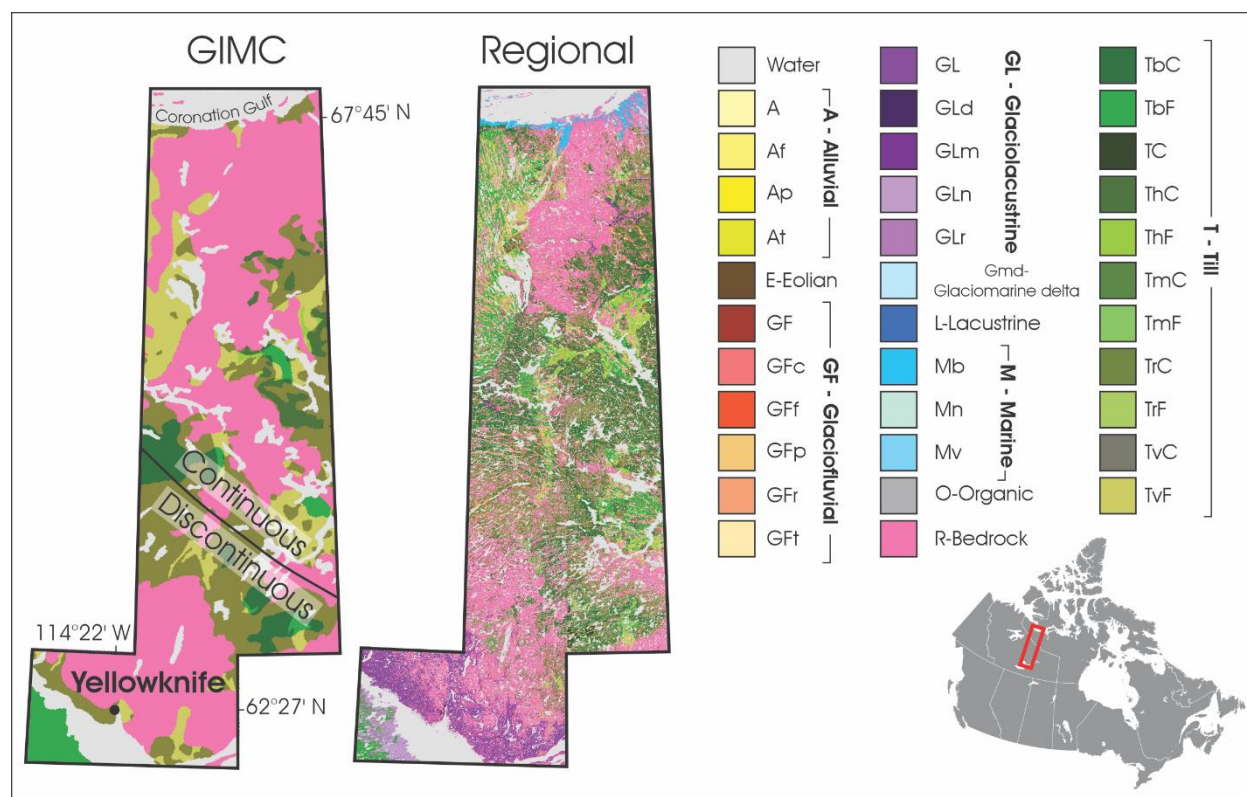
75 Figure 1. Surficial materials classes from the compilation used for the GMC (O'Neill et al., 2019) and regional compilation. Surficial geology unit abbreviations are from the Geological Survey of Canada Surficial Data Model (Deblonde et al., 2019, Appendix 2). Suffixes: f = fan, p = plain, t = terrace(d), c = ice contact, r = ridged (T)/esker (GF)/beach (GL), d = deltaic, m = moraine, b = blanket, n = nearshore, v = veneer, h = hummocky. Till suffixes 'C' and 'F' indicate coarse- and fine-grained units, respectively, based on underlying bedrock geology (see Sect. 3).
