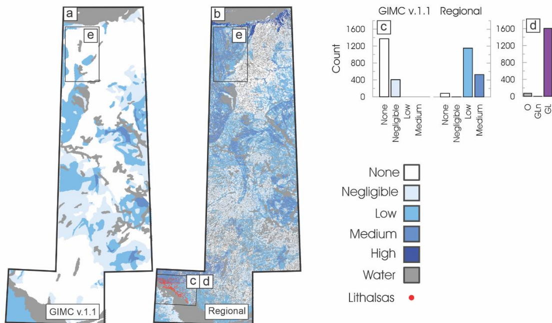
255 Figure 6. Modelled segregated ice abundance from a) GIMC v.1.1, b) the regional modelling, with inset (labelled c,d) showing mapped lithalsas within the modelled domain (n=1683) in the Great Slave Lowlands from Stevens et al. (2012), c) histogram of mapped lithalsas from b) and corresponding ground ice abundance on the national and regional-scale mapping, respectively, d) histogram of surficial geology from the regional compilation underlying each mapped lithalsal point, and e) region with widespread tills mapped on the RC, where mudboils and solifluction lobes are common, indicating frost-susceptible sediments (Dredge et al., 1999).
