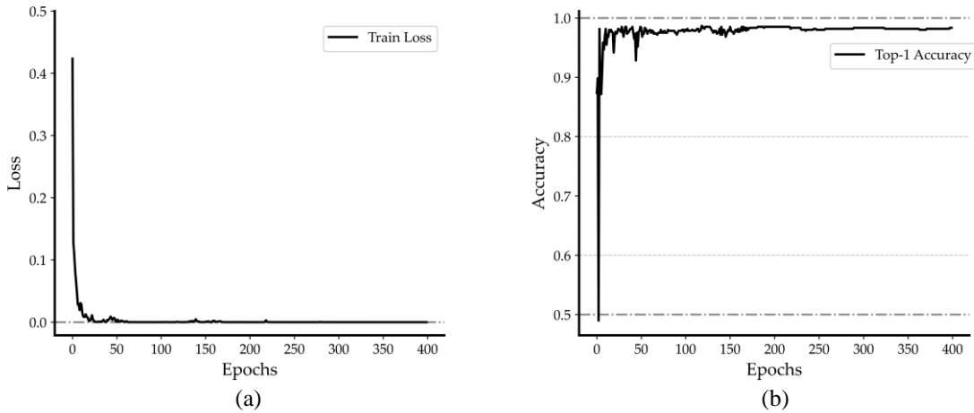
380 Figure 5. YOLOv8 classification model training results. (a) Loss curve for network training; (b) Top-1 network 385 training accuracy curve of the training set.
