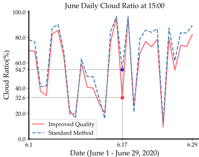
485 Figure 9. Comparison of cloud cover between the traditional NRBR threshold segmentation method and the finite sector partitioned K-means clustering method in June 2020.
