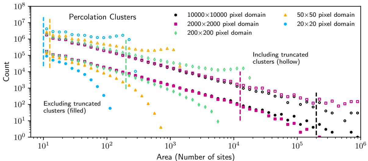
Figure 6. As for Figure 4, but for cluster areas in the percolation lattices.
