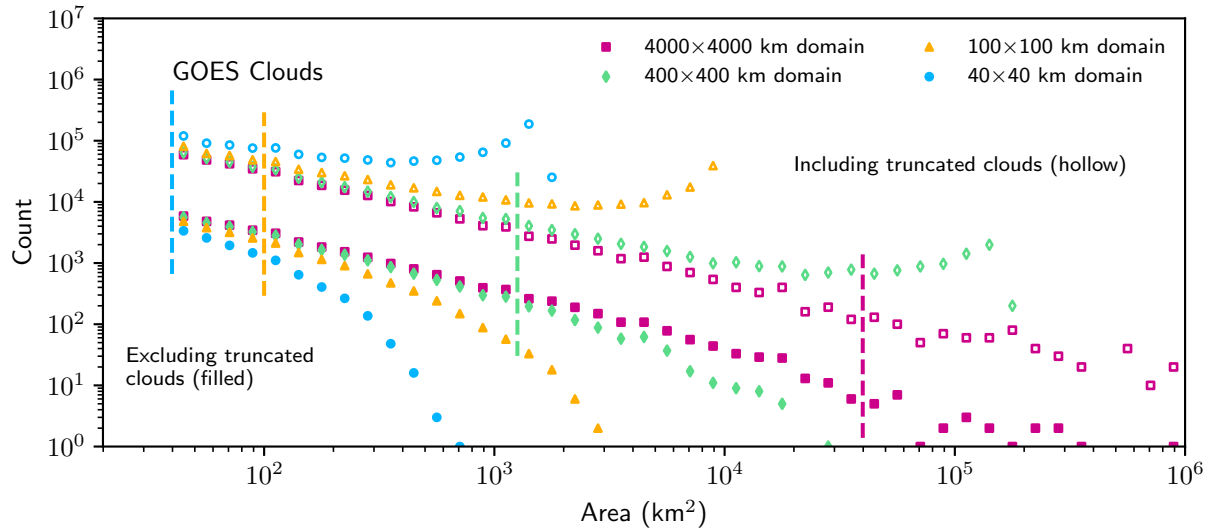
Figure 4. Histograms of cloud areas for several sizes of subdomain from GOES West. Filled shapes indicate histograms which do not include truncated clouds, while hollow shapes include truncated clouds. Hollow shapes are offset vertically by a factor of 10 for clarity. The vertical dashed lines mark the first bin in which 50% of objects are truncated by the domain edge for each domain size.
