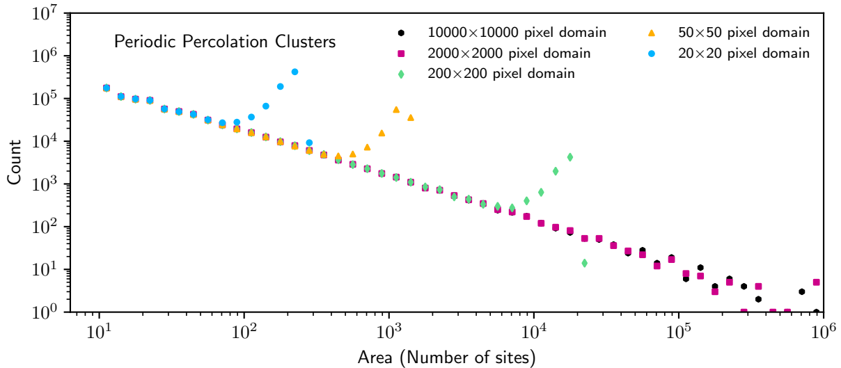
Figure 8. Histogram of cluster areas in doubly-periodic percolation lattices for several domain sizes.
