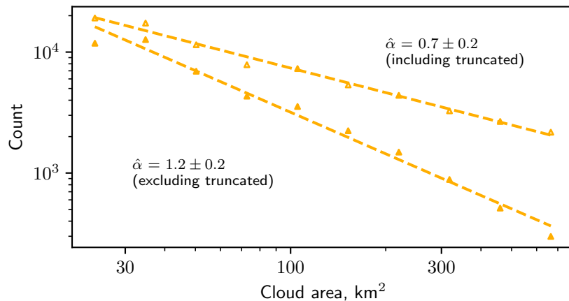
Figure 7. Example of how a measurement \hat{\alpha} of the power law exponent could be biased by whether or not truncated clouds are included in the analysis. The histograms shown are a subset of created using all the 100 \times 100 km subdomains from GOES. The same histograms are shown in Fig. 4 but spanning a wider range of scales. This region-particular range of scales is heavily influenced by the choice of including truncated clouds. Fits for \alpha are shown in Table 1.
