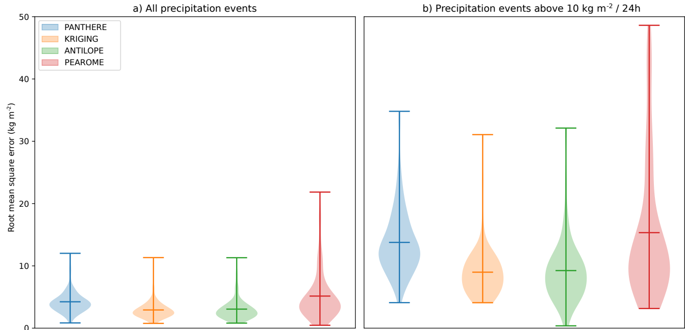
Figure 6. Distribution of the root mean square deviation of the existing precipitation estimation products from all ski-resort reference observations of daily precipitation (a) and daily precipitation above 10 \text{ kg m}^{-2} (b) over all evaluation stations. Precipitation estimates come from radar-only observations (PANTHERE), a kriging of gauge observations (KRIGING), a fusion of radar and gauge observations (ANTILOPE), and the ensemble mean of the post-processed high-resolution ensemble NWP model (PEAROME).
