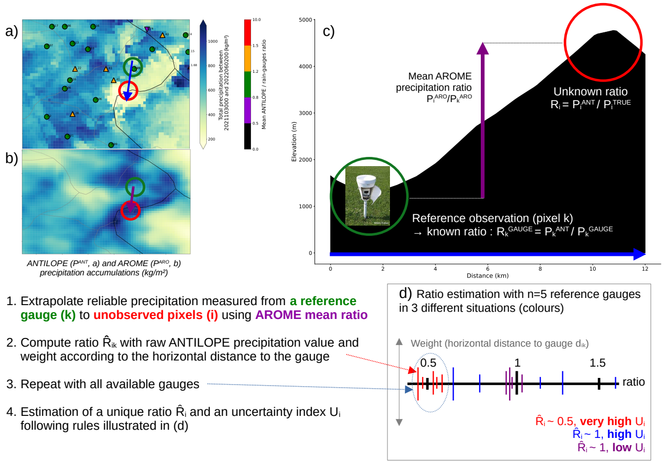
Figure 3. Illustration of the climatological ANTILOPE error estimation over the Mont-Blanc (circled in red) based on (a) the Yearly ANTILOPE precipitation accumulation ( P^{ANT} ) from 30 October 2021 to 2 June 2022 and the mean ANTILOPE / gauge ratio ( R^{GAUGE} ) observed at automatic stations and (b) the AROME precipitation accumulation. The marker associated with each evaluation station on panel a is a circle if the ratio between ANTILOPE and the reference gauge precipitation estimates is not considered significant (between 0.8 and 1.2) and a triangle facing up (resp. down) if this ratio is significantly higher (resp. lower) than 1.
