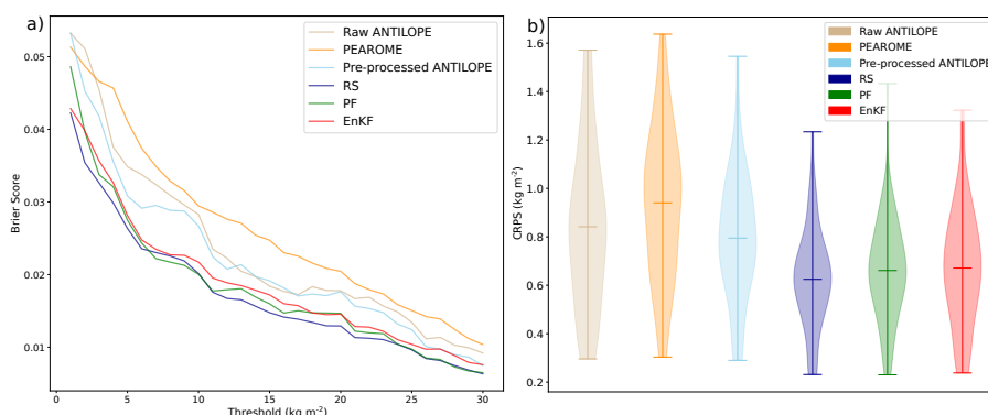
Figure 9. Evolution of the mean Brier score over all evaluation stations and dates for different daily precipitation thresholds ranging from 1 \text{ kg m}^{-2} to 30 \text{ kg m}^{-2} (a). Distribution of the mean continuous rank probability score over the reference stations (b). Six precipitation
