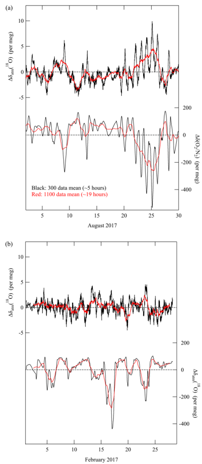
1000 Figure 6: (a) Rolling average values of \Delta\delta_{\text{atm}}(^{18}\text{O}) and \Delta\delta(\text{O}_2/\text{N}_2) for 300 data (black) and 1100 data (red) at TKB in August 2017. \Delta denotes deviations from the monthly mean value. (b) Same as in (a), but for February 2017.
