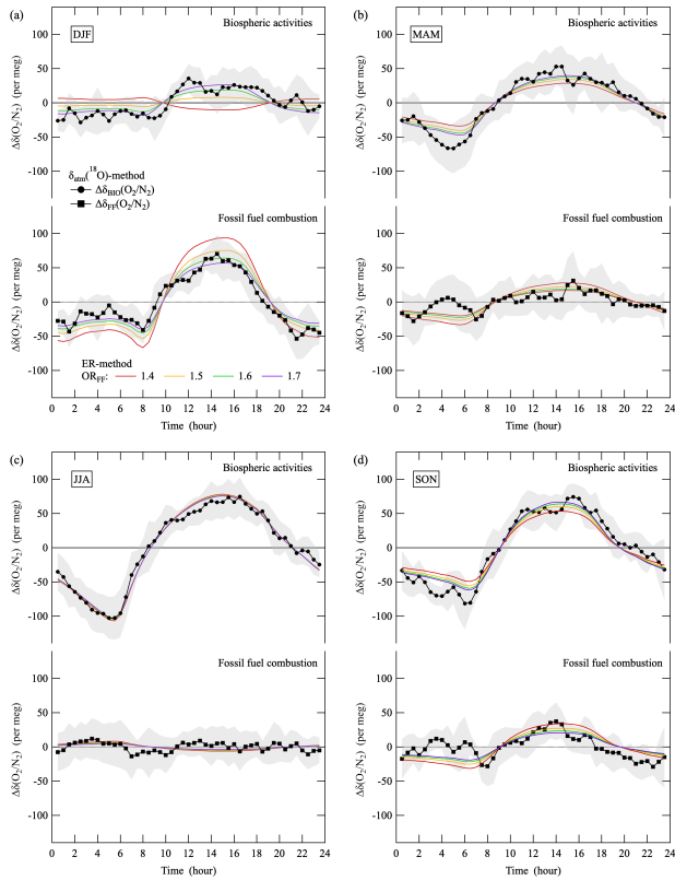
990 Figure 5: (a) Plots of average diurnal cycles of the \Delta\delta_{\text{BIO}}(\text{O}_2/\text{N}_2) and \Delta\delta_{\text{FF}}(\text{O}_2/\text{N}_2) for each season estimated by the \delta_{\text{atm}}(^{18}\text{O}) -method. \Delta\delta(\text{O}_2/\text{N}_2) driven by activities in the terrestrial biosphere and fossil fuel combustion estimated by the ER-method are also shown. See text for details of the \delta_{\text{atm}}(^{18}\text{O}) - and ER-methods. \Delta denotes deviations from the diurnal mean values. Error bands for \Delta\delta_{\text{BIO}}(\text{O}_2/\text{N}_2) are derived from \Delta\delta_{\text{atm}}(^{18}\text{O}) in Figure 4a. Error bands for \Delta\delta_{\text{FF}}(\text{O}_2/\text{N}_2) are assumed to be the same as those for \Delta\delta_{\text{BIO}}(\text{O}_2/\text{N}_2) .
