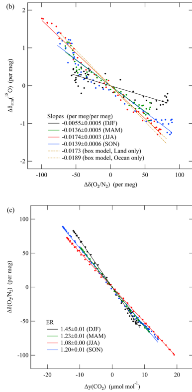
975 Figure 4: (a) Plots of average diurnal cycles of \Delta\delta_{\text{atm}}(^{18}\text{O}) , \Delta\delta(\text{O}_2/\text{N}_2) , \Delta\gamma(\text{CO}_2) , and \Delta\delta(\text{Ar}/\text{N}_2) (open circles) observed at the TKB site during 2013–2022 for each season: December to February (black), March to May (green), June to August (red), and September 980 to November (blue). Error bands indicate year-to-year variations during the observation periods ( \pm 1\sigma ). Those of \Delta\delta_{\text{atm}}(^{18}\text{O}) , \Delta\delta(\text{O}_2/\text{N}_2) , and \Delta\gamma(\text{CO}_2) , corrected for thermally diffusive fractionation, are also plotted (filled circles) (see text). The range of the vertical axis for \Delta\delta(\text{Ar}/\text{N}_2) was adjusted arbitrarily to facilitate visual assessment of the variations of the observed \Delta\delta_{\text{atm}}(^{18}\text{O}) due to thermally diffusive fractionation. Average diurnal cycles of \Delta\delta_{\text{atm}}(^{18}\text{O}) and \Delta\delta(\text{O}_2/\text{N}_2) that were simulated with a box model are also shown. The simulated values that considered only terrestrial and marine respiration/production are shown by solid and dashed other lines, respectively (see text). \Delta denotes deviations from the diurnal mean values. (b) Relationships between \Delta\delta_{\text{atm}}(^{18}\text{O}) and
