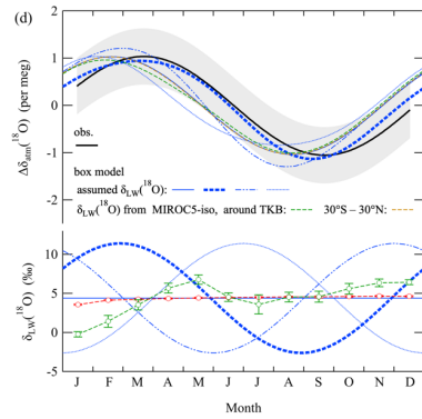
1010 Figure 7: (a) Monthly mean values of \delta_{\text{atm}}(^{18}\text{O}) and \delta(\text{O}_2/\text{N}_2) observed at TKB for the period 2013–2022. Local effects of fossil fuel combustion around TKB were excluded from \delta(\text{O}_2/\text{N}_2) . See text for details. (b) Detrended monthly mean values (open black circles) and their 10-year average (filled black circles) of \Delta\delta_{\text{atm}}(^{18}\text{O}) at TKB for the period 2013–2022. Those of \Delta\delta(\text{O}_2/\text{N}_2) , extracted by removing the contributions of solubility change by using the average seasonal \delta(\text{Ar}/\text{N}_2) cycle at TKB (see text), are also shown. Average seasonal cycles of \Delta\delta_{\text{atm}}(^{18}\text{O}) and \Delta\delta(\text{O}_2/\text{N}_2) obtained by applying one-harmonic best-fit curves to the data (solid black lines) and those simulated by the box model (solid blue lines) are also shown. We assumed a constant \delta_{\text{atm}}(^{18}\text{O}) of 4.4 ‰ for the simulation. \Delta denotes deviations from the annual mean values. (c) Same average seasonal cycles of \Delta\delta_{\text{atm}}(^{18}\text{O}) and \Delta\delta(\text{O}_2/\text{N}_2) simulated by the box model in (b) (blue solid lines), and the respective contributions of terrestrial production (green dashed lines), terrestrial
