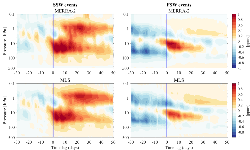
Figure 7. Evolution of the ozone anomalies for the composite of SSW and FSW events as a function of time and pressure averaged the polar regions ( 70^{\circ} - 90^{\circ} \text{ N} ) for (a, b) MERRA-2 and (c, d) MLS.
