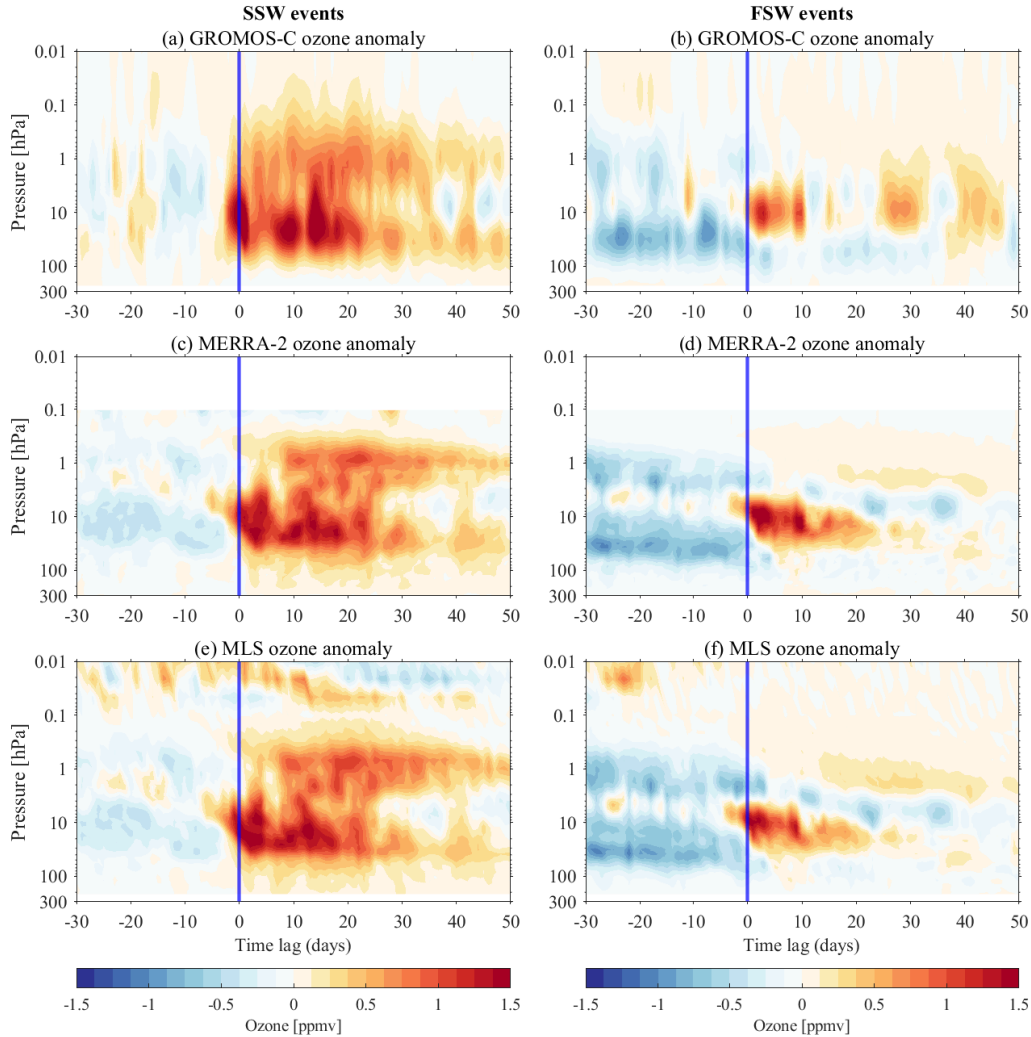
Figure 4. Same as Fig. 3, but for anomalies at Ny-Ålesund, Svalbard (79° N, 12° E)
