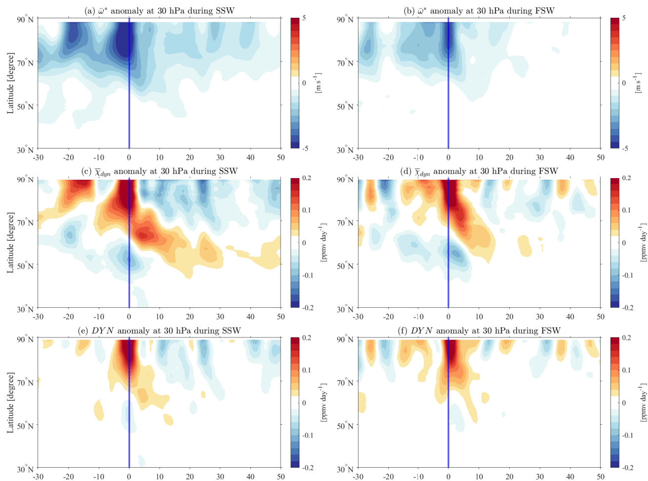
Figure A1. Evolution of the \bar{\omega}^* anomalies dO_3/dt ( m s^{-1} ), \bar{\chi}_{dyn} , and DYN anomalies at 30 hPa ( ppmv day^{-1} ) for the composite of SSW (a, c, e) and FSW (b, d, f) events as a function of time and latitude in the northern hemisphere.
