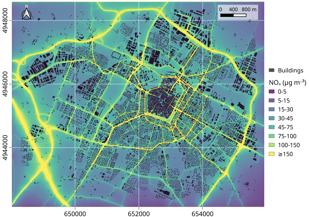
Figure 6. Spatial distribution of average simulated NO x concentrations in the city of Modena from January 8 to March 8, 2020, as modelled by GRAMM-GRAL. Urban building locations are depicted in black, while NO x concentrations are colour-coded from purple to yellow, illustrating variations across the city.
