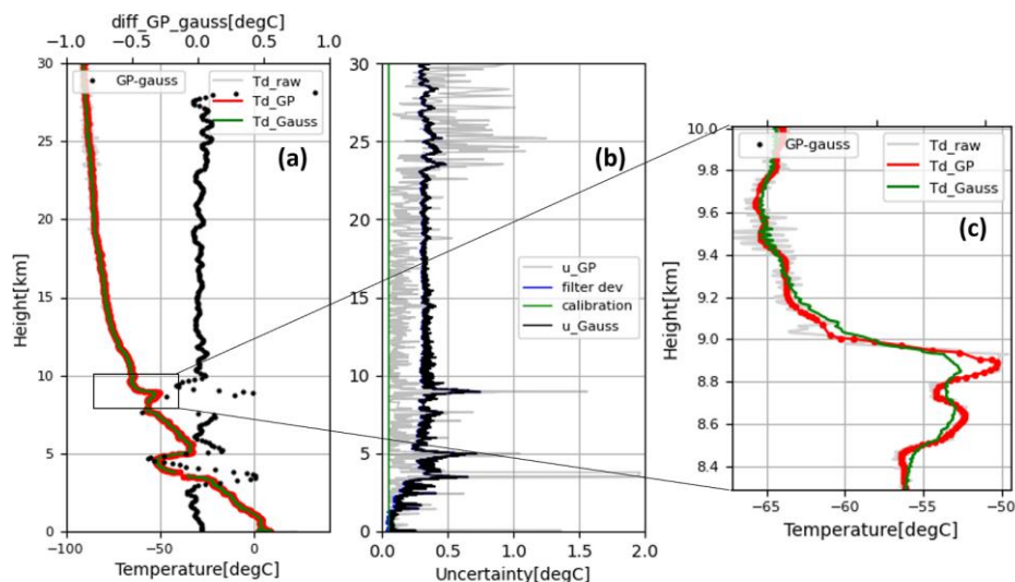
Figure 10: Frost point profiles on 26 November 2021 at Tateno smoothed with the golden point method (red line) and gaussian filter with \sigma = 13 (green line). (a) Whole profile of frost point and black dots indicates differences between frost points smoothed with each method. (b) Frost point uncertainty in the case of a gaussian filter, filtering deviation (blue), calibration error (green), and total uncertainty (black). Gray line is the uncertainty of the golden point method. (c) Close-up profiles between 8.4 and 10 km. The grey line indicates the raw profile of mirror temperature.
