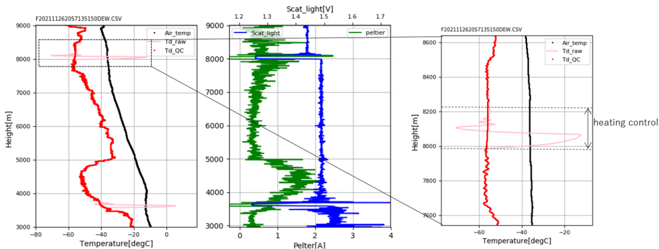
Figure 6: Heating control stage at -36\text{ }^{\circ}\text{C} and -58\text{ }^{\circ}\text{C} for the profile on 26 November 2021 at Tateno, Japan ( 36.06^{\circ}\text{ N} , 140.13^{\circ}\text{ E} ). For each control, the mirror is heated for \sim 5\text{ s} to clear the mirror surface. When the mirror temperature (pink) is heated, the scattered light signal (blue) goes down to the base level, indicating that the frost layer disappears. Red lines indicate the mirror temperatures after quality control and interpolation.
