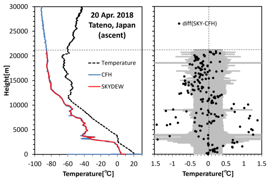
Figure 12. Comparison of soundings with CFH (blue line) and SKYDEW (red line) at Tateno on 20 April 2018. The cooling limit for SKYDEW was 21 km for this sounding, as shown by the black dashed line. In the right panel, the black dots are the differences and light grey indicates the combined uncertainties ( k = 2 ) calculated from SKYDEW and CFH measurement uncertainties. The uncertainty of CFH was assumed as a constant value of 0.2 K.
