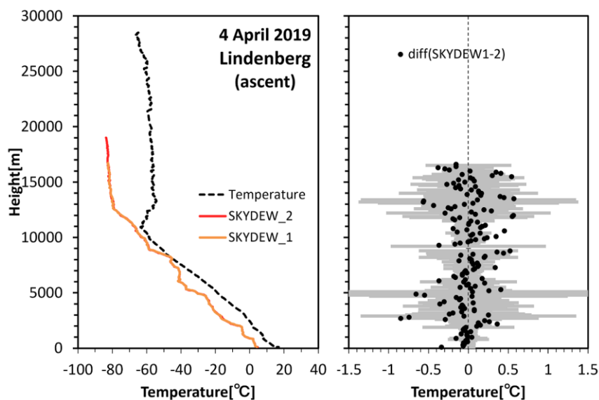
845 Figure 11. Dual sounding with two SKYDEWs on 4 April 2019 in Lindenberg, Germany (52.21° N, 14.12° E). The left panel shows the dew/frost point profile (red and orange lines) and air temperature measured by radiosonde (black line). In the right panel, the black dots are the differences between the two SKYDEW measurements and light grey indicates the combined uncertainties ( k = 2 ).
