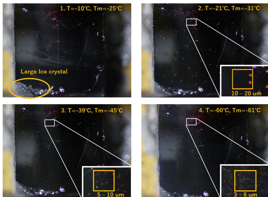
Figure 5: Condensates on the mirror at temperatures of -10\text{ }^{\circ}\text{C} (top left), -20\text{ }^{\circ}\text{C} (top right), -40\text{ }^{\circ}\text{C} (bottom left), and -60\text{ }^{\circ}\text{C} (bottom right) in the thermostatic chamber.
