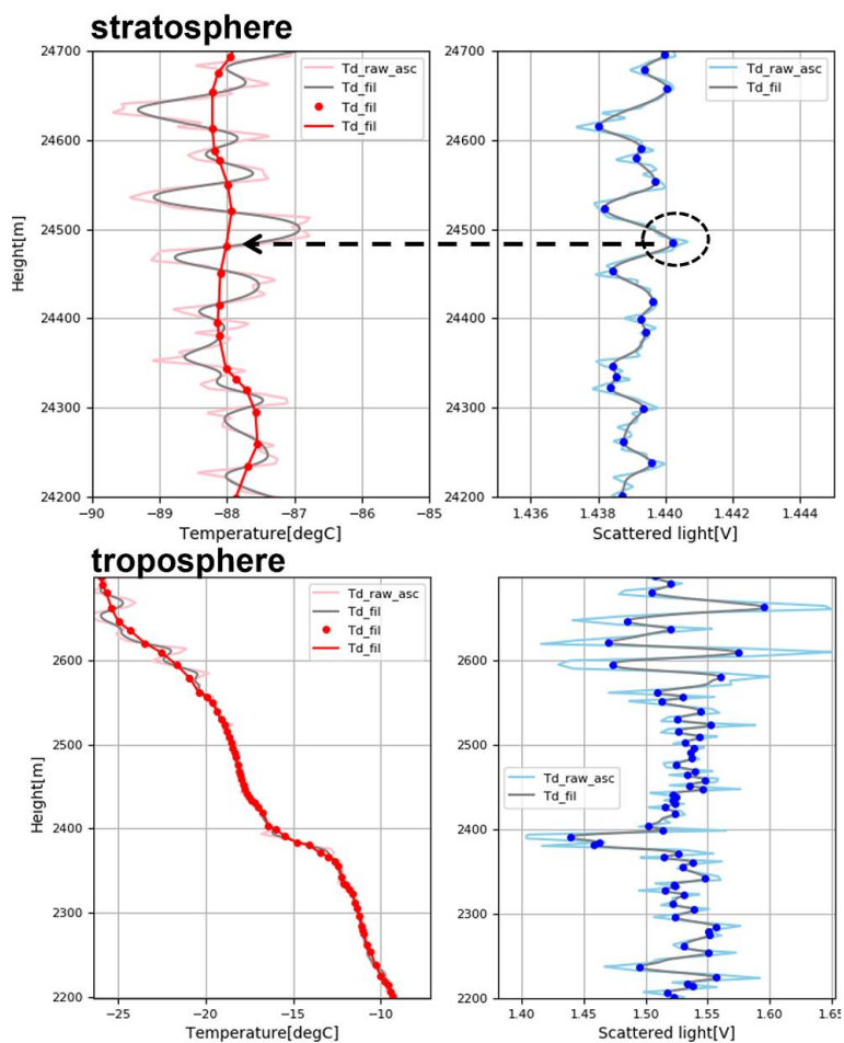
Figure 7: Golden point detection for the sounding shown in Fig. 6. Example profiles are shown of dew/frost point in the troposphere (bottom) and stratosphere (top). The right panels show the scattered light, including the raw data (light blue) and its smoothed profile (grey line). The blue dots are the detected golden points. The left panel shows the mirror temperature, including the raw data (pink) and its smoothed profile (grey line). Red dots are mirror temperatures corresponding to golden points, which are frost points.
