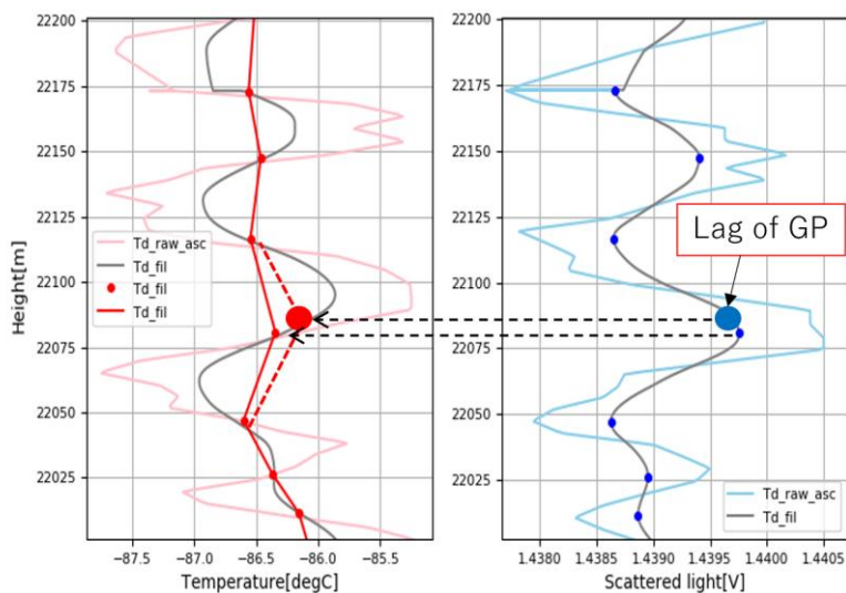
Figure 8. As for Fig. 7, but explaining the timing error of the golden point. If the equilibrium point of scattered light is mistakenly detected as the golden point (large blue dot in the right panel), the frost point is erroneously determined (large red dot in the left panel).
