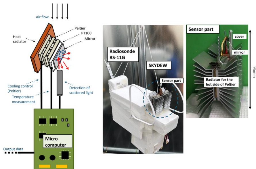
Figure 1: Left: Schematic of SKYDEW. Right: Photograph of SKYDEW with the Meisei RS-11G and a close-up of the sensor part. The sensor probe is positioned on top because SKYDEW is designed for measurement during balloon ascent.
