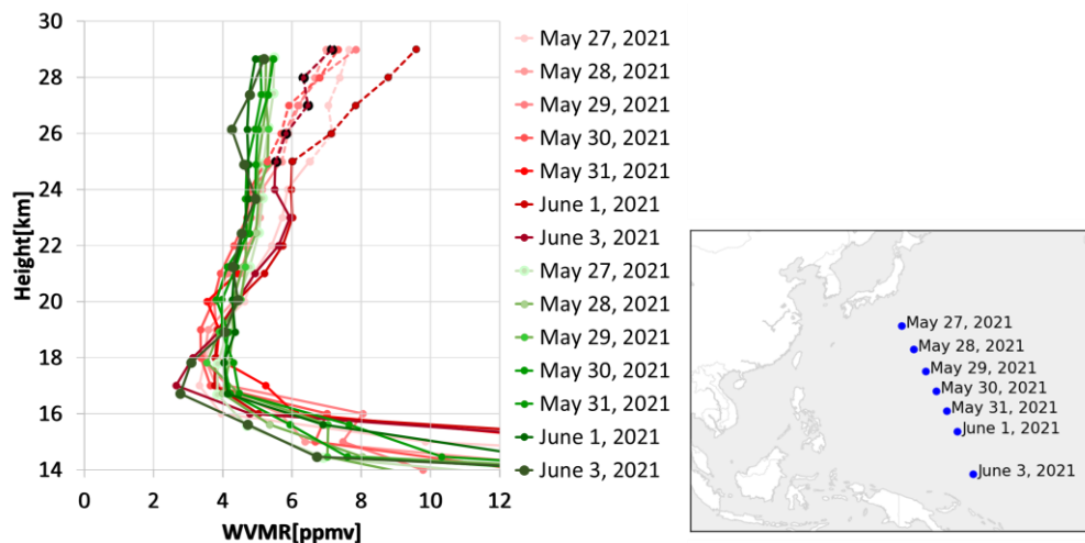
870 Figure 15. Water vapor mixing ratio from SKYDEW (red) and Aura MLS (green). Dashed lines indicate the suspected contaminated profiles. Right panel shows the launching points and dates for SKYDEW.
