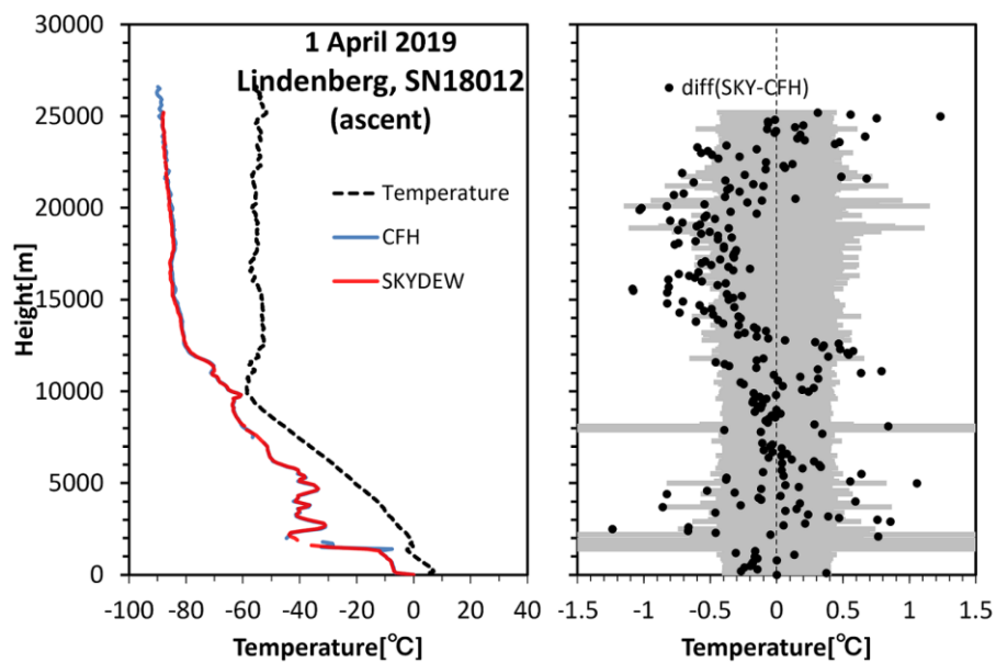
Figure 13. As in Fig. 12, but for the profile at Lindenberg on 1 April 2019.
