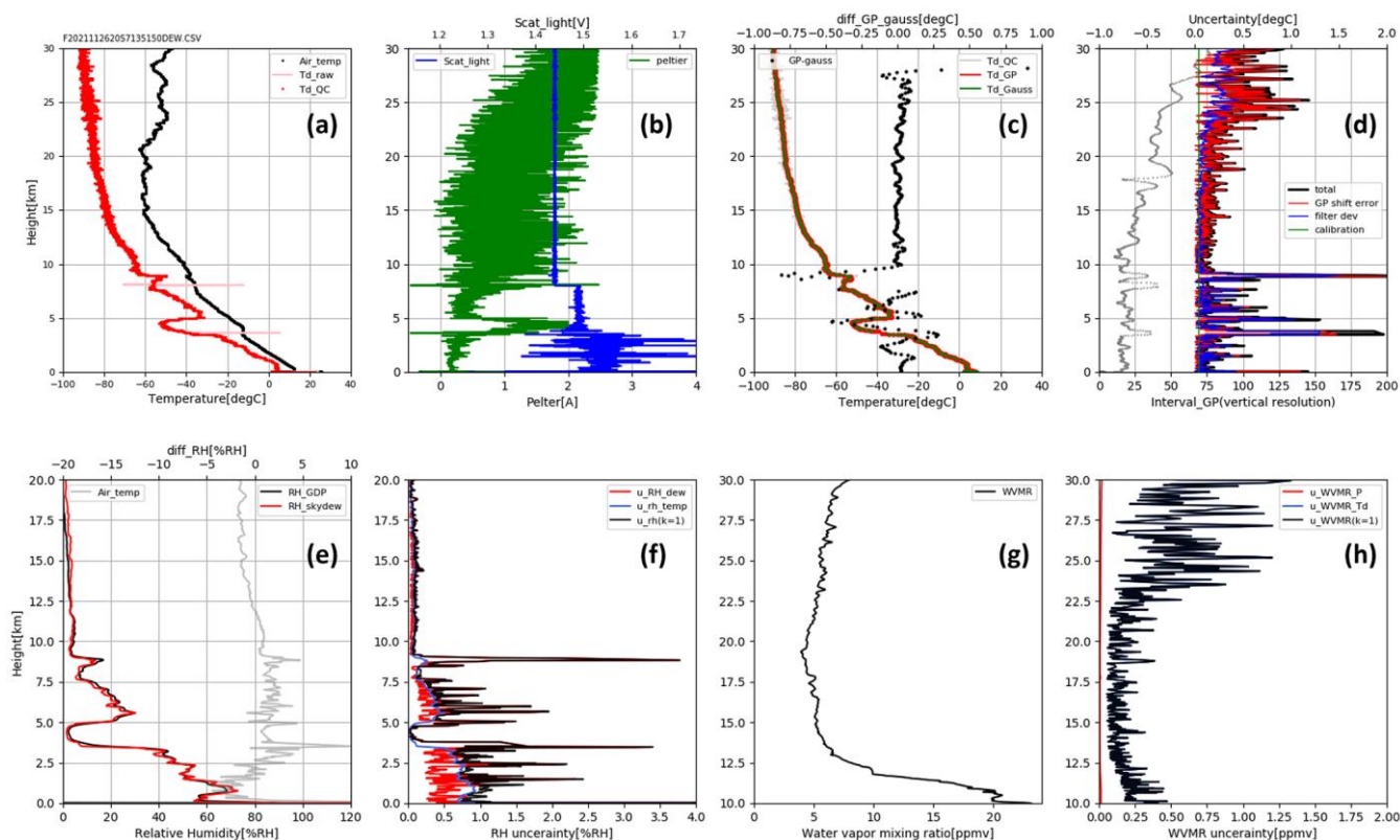
Figure 9. Profiles of dew/frost point and its uncertainty from SKYDEW on 26 November 2021 at Tateno. Mirror temperature and air temperature (a), scattered light intensity and Peltier current (b), smoothed dew/frost point with the golden point method and gaussian filter (c), uncertainty ( k = 1 ) and the vertical resolution (d), RH profiles and its difference (e), uncertainty of RH calculated from SKYDEW ( k = 1 ) (f), water vapor mixing ratio from SKYDEW (g), and uncertainty of water vapor mixing ratio( k = 1 ) (h).
