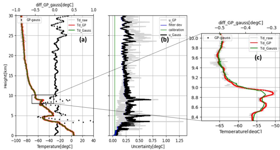
Figure 10: Frost point profile on 26 November 2021 at Tateno smoothed with the golden point method (red line) and 910 gaussian filter with \sigma = 13 (green line). (a) Whole profile of frost point and black dots indicates differences between frost points smoothed with each method. (b) Frost point uncertainty in the case of a gaussian filter, filtering deviation (blue), calibration error (green), and total uncertainty (black). Gray line is the uncertainty of the golden point method. (c) Close-up profiles between 8.4 and 10 km. The grey line indicates the raw profile of mirror temperature.
