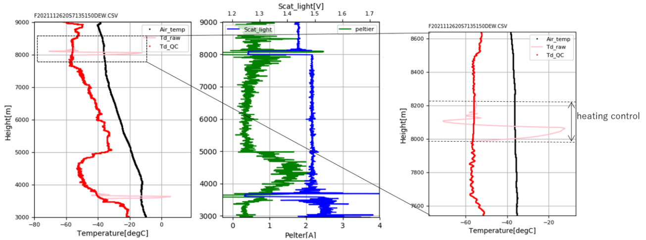
Figure 6: Heating control stage at -36\text{ }^{\circ}\text{C} and -58\text{ }^{\circ}\text{C} for the profile on 26 November 2021 at Tateno, Japan ( 36.06^{\circ}\text{ N} , 140.13^{\circ}\text{ E} ). For each control, the mirror is heated for \sim 5\text{ s} to clear the mirror surface. When the mirror temperature (pink) is heated, the scattered light signal (blue) goes down to the base level, indicating that the frost layer disappears. Note that in this figure the Peltier current is defined that cooling is positive and heating is negative. Red lines indicate the mirror temperatures after quality control and interpolation.
