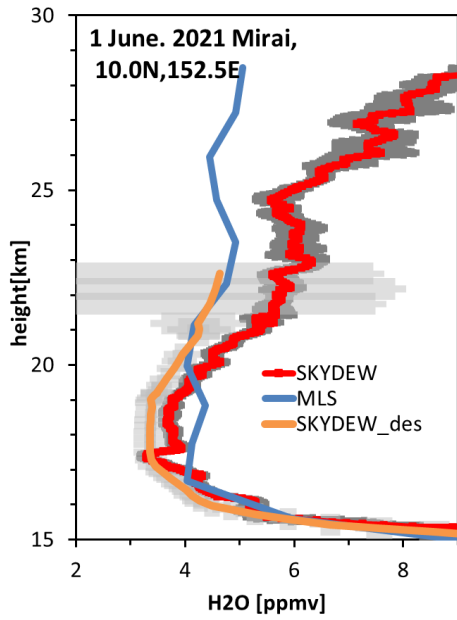
Figure 17. Water vapor mixing ratio from SKYDEW and MLS on 1 June 2021. Red line is the ascent profile and orange line 965 the descent profile. Gray shading indicates the uncertainty of SKYDEW( k = 2 ).
