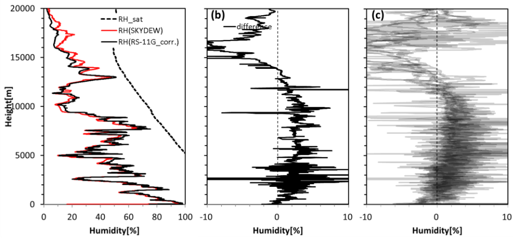
Figure 15. Comparison of RH with SKYDEW and RS-11G. The left panel shows the RH profiles on 27 May 2021 with SKYDEW (red) and RS-11G (black). Black dashed line indicates the RH of ice saturation. The center panel shows the difference. The right panel shows the differences of eight soundings over the Pacific Ocean between 27 May and 3 June.
