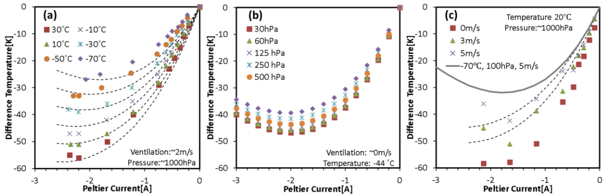
Figure 2: Cooling capability of the Peltier device used in this study. Shown are the temperature differences between the cold side of the Peltier device and the ambient air versus the Peltier current under various conditions obtained in a thermostatic chamber. The panels show the dependence on (a) air temperature, (b) air pressure, and (c) airflow rate. The dashed lines in the left and right panel indicate the theoretical values calculated by Eq. (10), using the parameter \alpha = 0.0099 , \beta = 0.0432 , R_e = 0.48 , and S = 0.00025 . The grey line in the panel (c) indicates the theoretical curve at the condition of -70^\circ\text{C} , 100 hPa and 5m/s.
