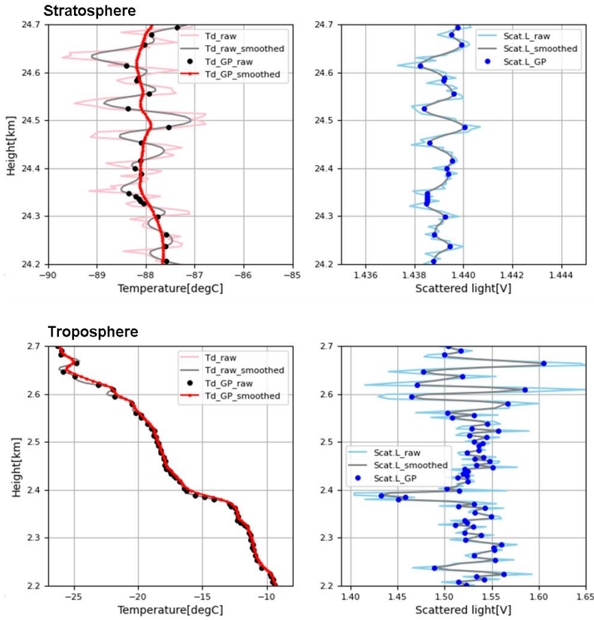
Figure 7: Golden point detection for the profile on 5 November 2019 at Moriya, Japan ( 35.93^\circ N, 140.00^\circ E). Example profiles are shown of dew/frost point in the troposphere (bottom) and stratosphere (top). The right panels show the scattered light, including the raw data (light blue) and its smoothed profile (grey line). The blue dots are the detected golden points. The left panel shows the mirror temperature, including the raw data (pink) and its smoothed profile (grey line). Red dots are mirror temperatures corresponding to golden points, which are frost points.
